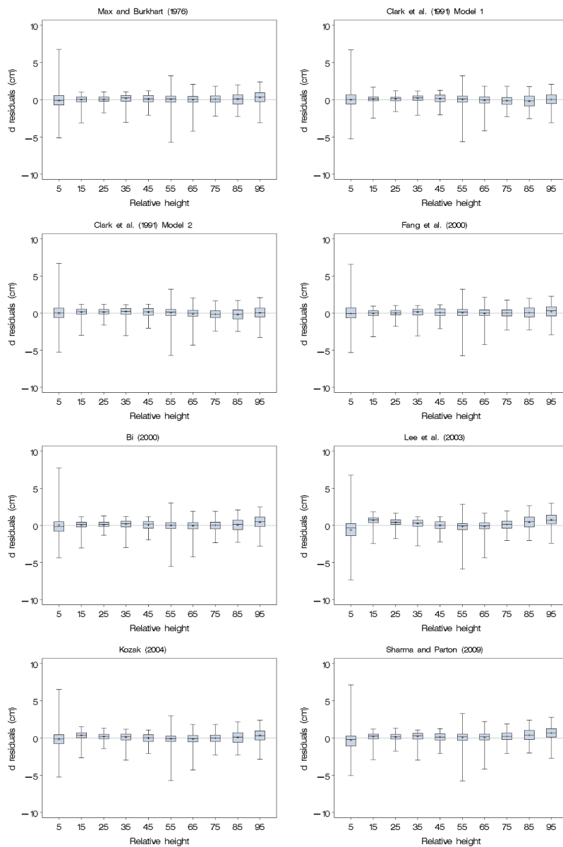
Fig. 2 Box plots of d residuals (cm) against relative heights for Manchurian Fir.
