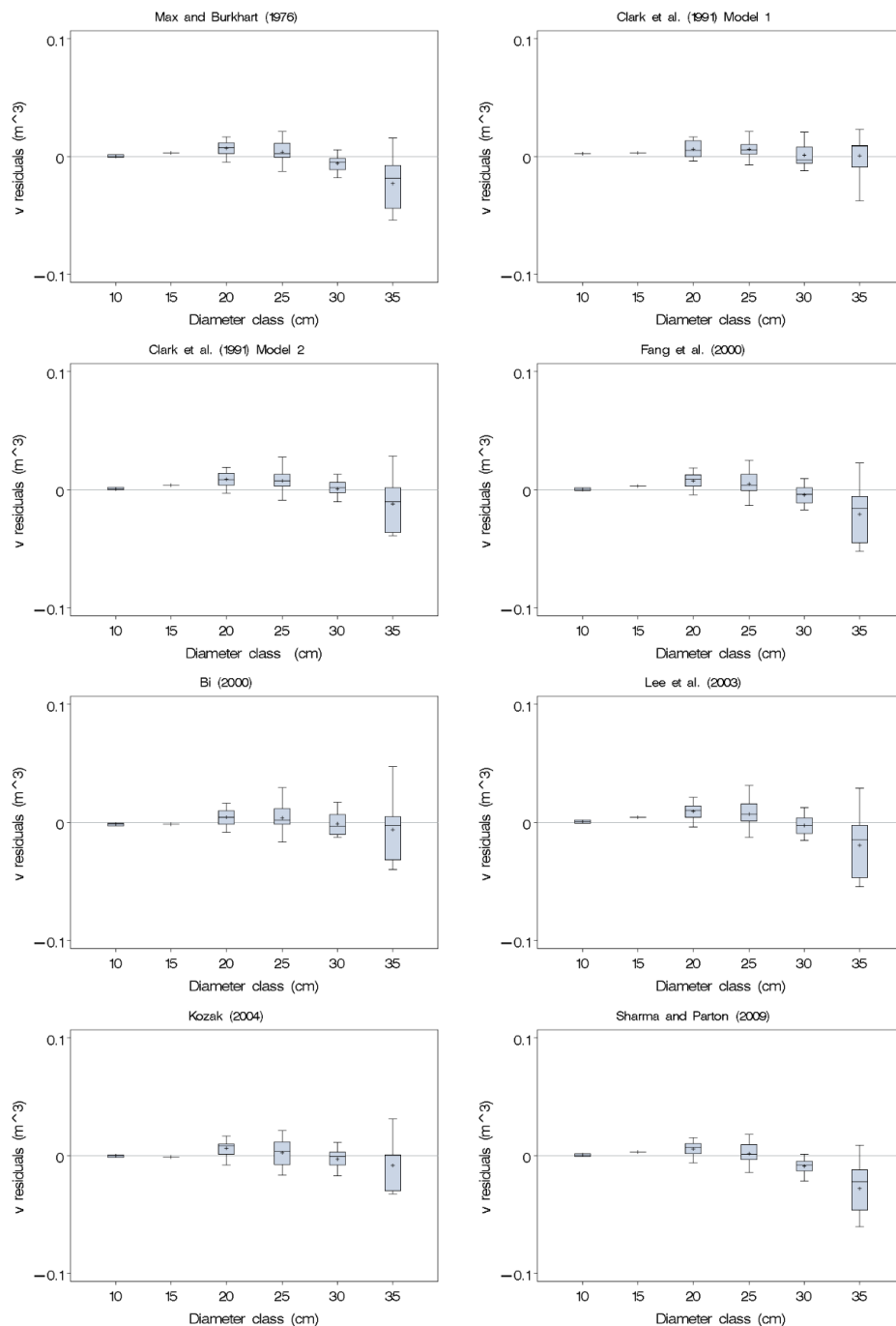
Fig. 5 Box plots of total volume residuals ( m^3 ) against diameter classes (cm) for Korean Spruce.
