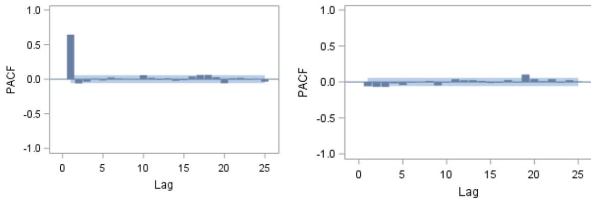
Fig. 1 An example of partial autocorrelation plotted against lag for Clark et al. (1991) Model 1 fit without considering the autocorrelation parameters (a) and using a first-order (b) continuous autoregressive error structure for Korean spruce.
