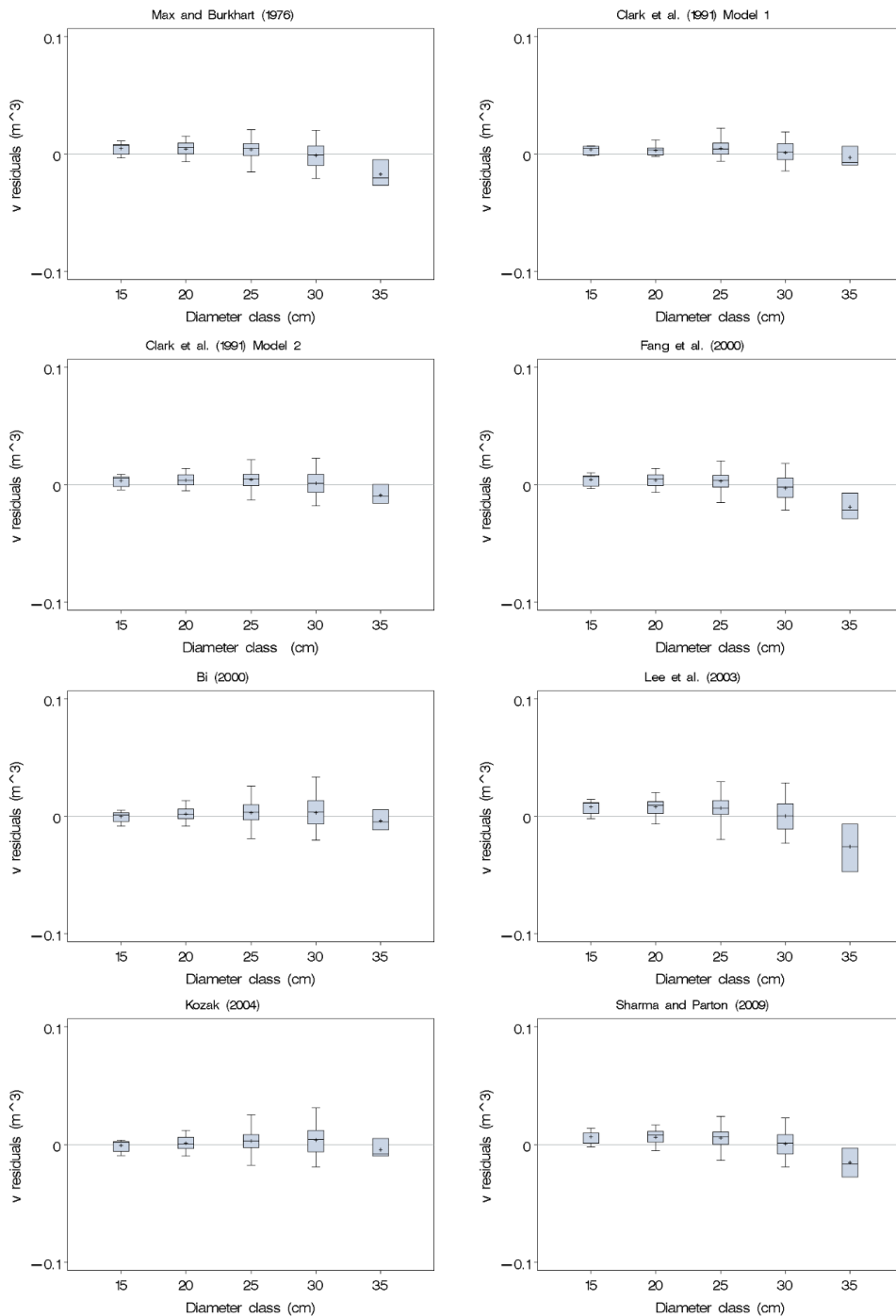
Fig. 4 Box plots of total volume residuals ( m^3 ) against diameter classes (cm) for Manchurian Fir.
