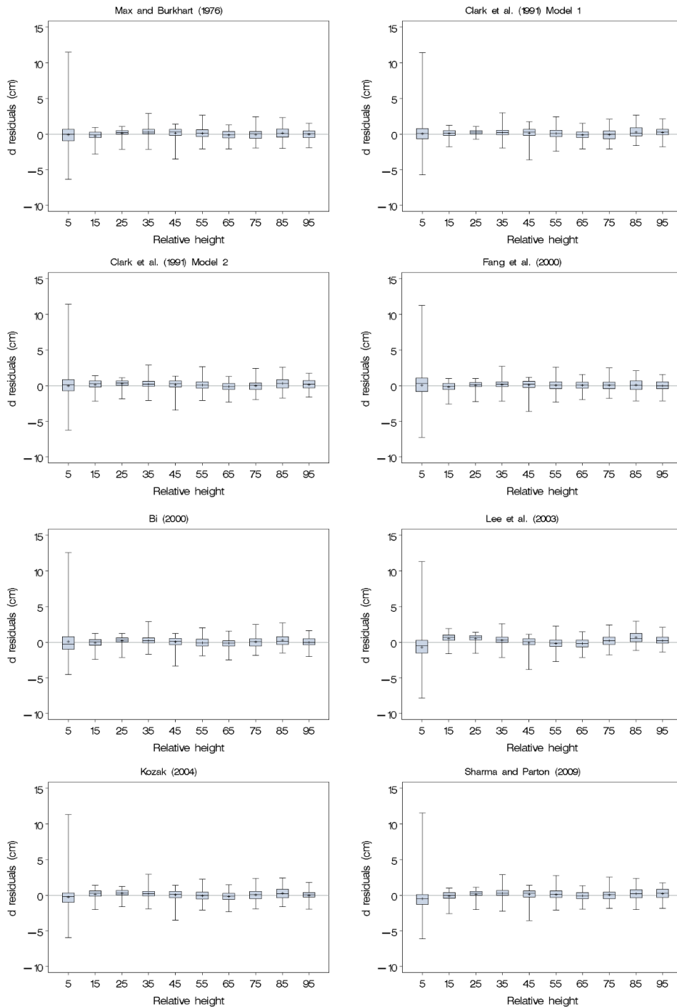
Fig. 3 Box plots of d residuals (cm) against relative heights for Korean Spruce.
