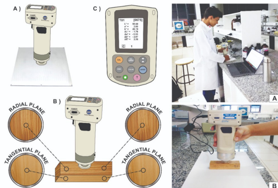
FIGURE 1 Mensuration of the wood colorimetric parameters. Where: A) Device calibration; B) Measurements on the sample surface in the radial and tangential planes and, C) Storage of colorimetric variables.
