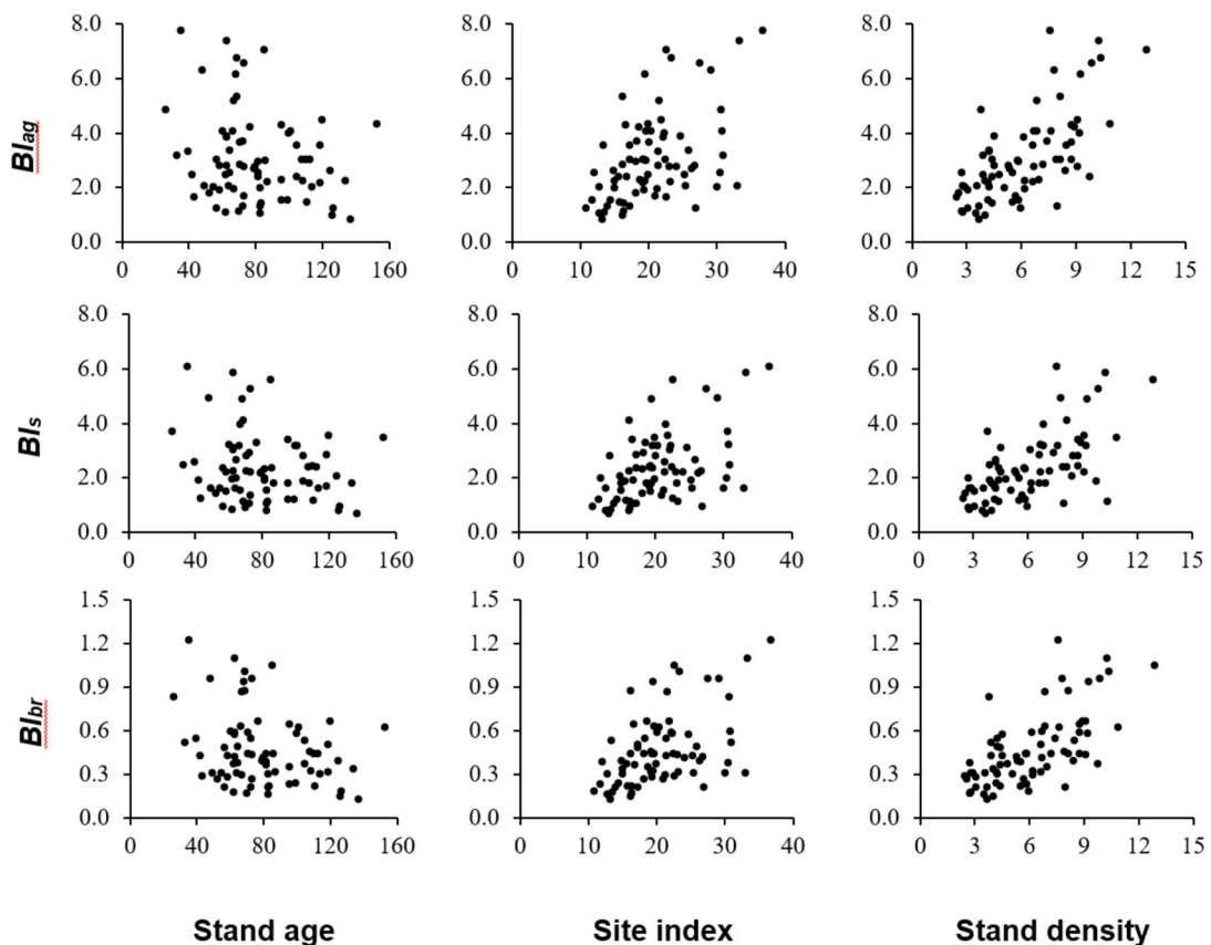
Figure 2: The relationships between biomass increments and stand characteristics.
