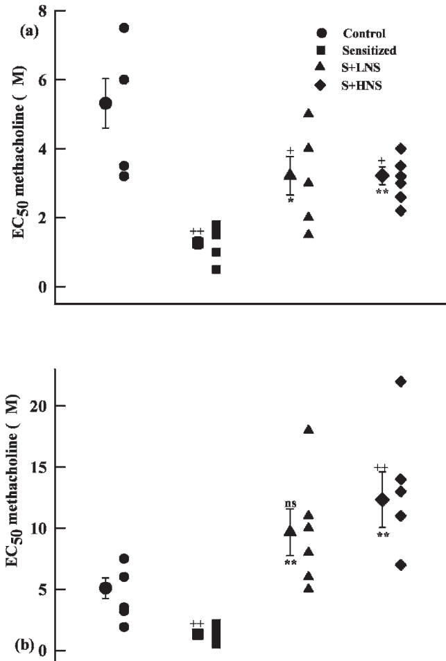
Figure 3 - Individual values and the mean \pm SEM (larger symbols with bars) of the tracheal response to methacholine ( EC_{50} ) in tissues either non incubated treated (a) or treated with 0.25 g% N. sativa extract (b; for each group, n=7 ). Statistical differences between the control and different groups: +; p < 0.05 , ++; p < 0.01 . Statistical differences between the S+LNS and S+HNS vs. sensitized group: **: p < 0.01 . There was no significant difference in the effects of the two different concentrations of the extract.
