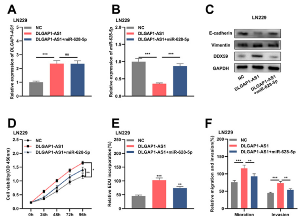
Figure 5. DLGAP1-AS1 regulates glioma cell proliferation, migration, invasion, and EMT via the miR-628-5p/DDX59 axis. A, The DLGAP1-AS1 overexpression vector and DLGAP1-AS1 overexpression vector + miR-628-5p mimic were transfected into LN229 cells, and the expression of DLGAP1-AS1 was detected using qRT-PCR. B, qRT-PCR was used to detect the expression of miR-628-5p in LN229 cells. C, Western blotting was used to detect the expression of DDX59 and EMT-related proteins E-cadherin and vimentin in LN229 cells. (D–E) The proliferation of LN229 cells was detected using CCK-8 (D) and EdU assays (E). F, Transwell assay was used to detect the migration and invasion of LN229 cells. The experiments were repeated three times, and the average was recorded. * p < 0.05 , ** p < 0.01 , and *** p < 0.001 , ns was not statistically significant.
