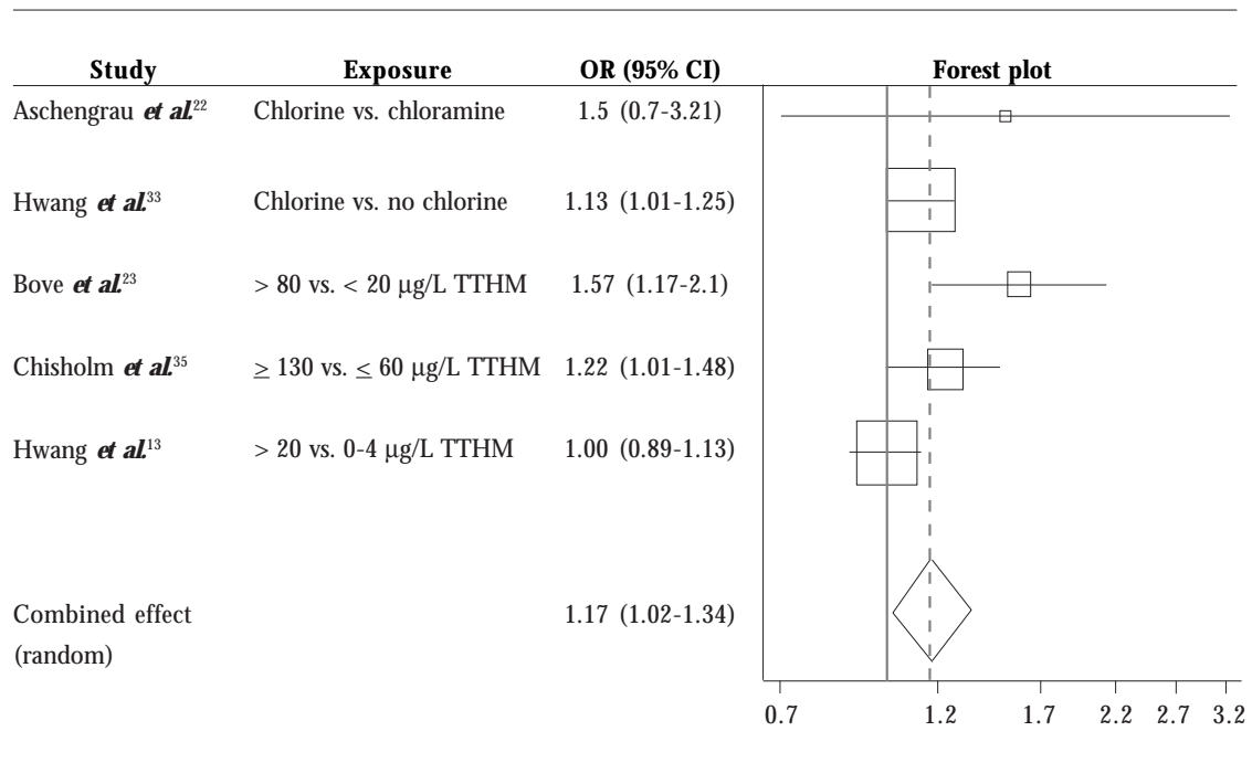
Figure 1. Study and summary risk estimates for any congenital anomalies and chlorination by-products. Test for heterogeneity: Q = 9.944 on four degrees of freedom ( p = 0.041 ). Egger test: weighted p -value for intercept 0.16.
