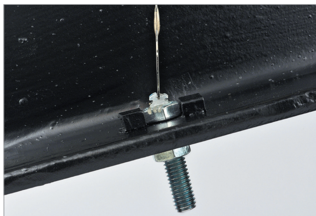
Figure 1 - Iron support customized for the tensile test with 12° inclination, so that the bracket slot was parallel to the machine test cell and the stainless steel 0.40 x 0.40 mm wire was engaged.
