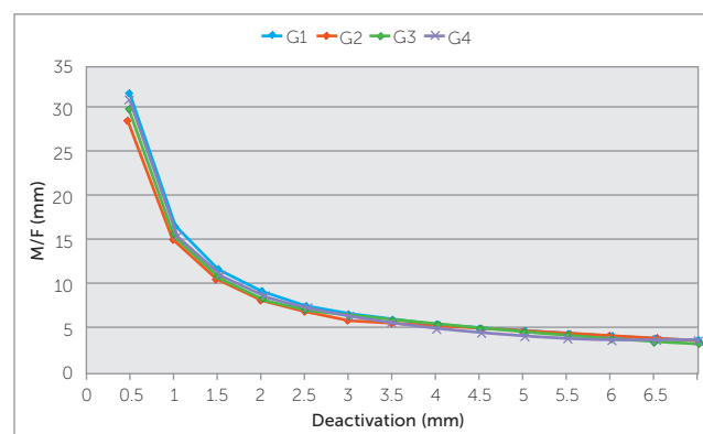
Figure 10 - Figure 7 mathematically adjusted in order to isolate the effect of the overactivation on the MF ratios produced by the groups caused by the overlapping of the vertical extensions. The force systems developed by the groups was quite similar.
