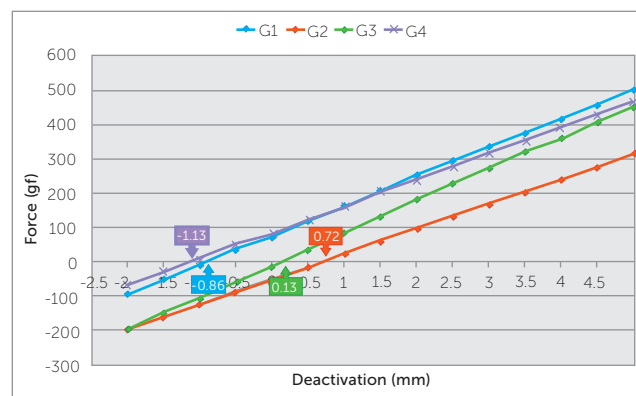
Figure 5 - Figure 4 slightly modified. The x- intercepts, pointed by the arrows, depict the amount of horizontal overlap of the vertical extensions of the TLSs in "neutral position" and were calculated by linear interpolation.
