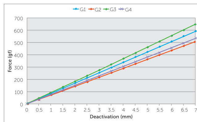
Figure 8 - Figure 4 mathematically adjusted in order to isolate the effect of the overactivation on the force produced by the groups caused by the overlapping of the vertical extensions.
