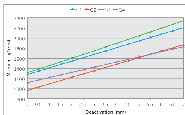
Figure 9 - Figure 6 mathematically adjusted in order to isolate the effect of the overactivation on the moments produced by the groups caused by the overlapping of the vertical extensions.
