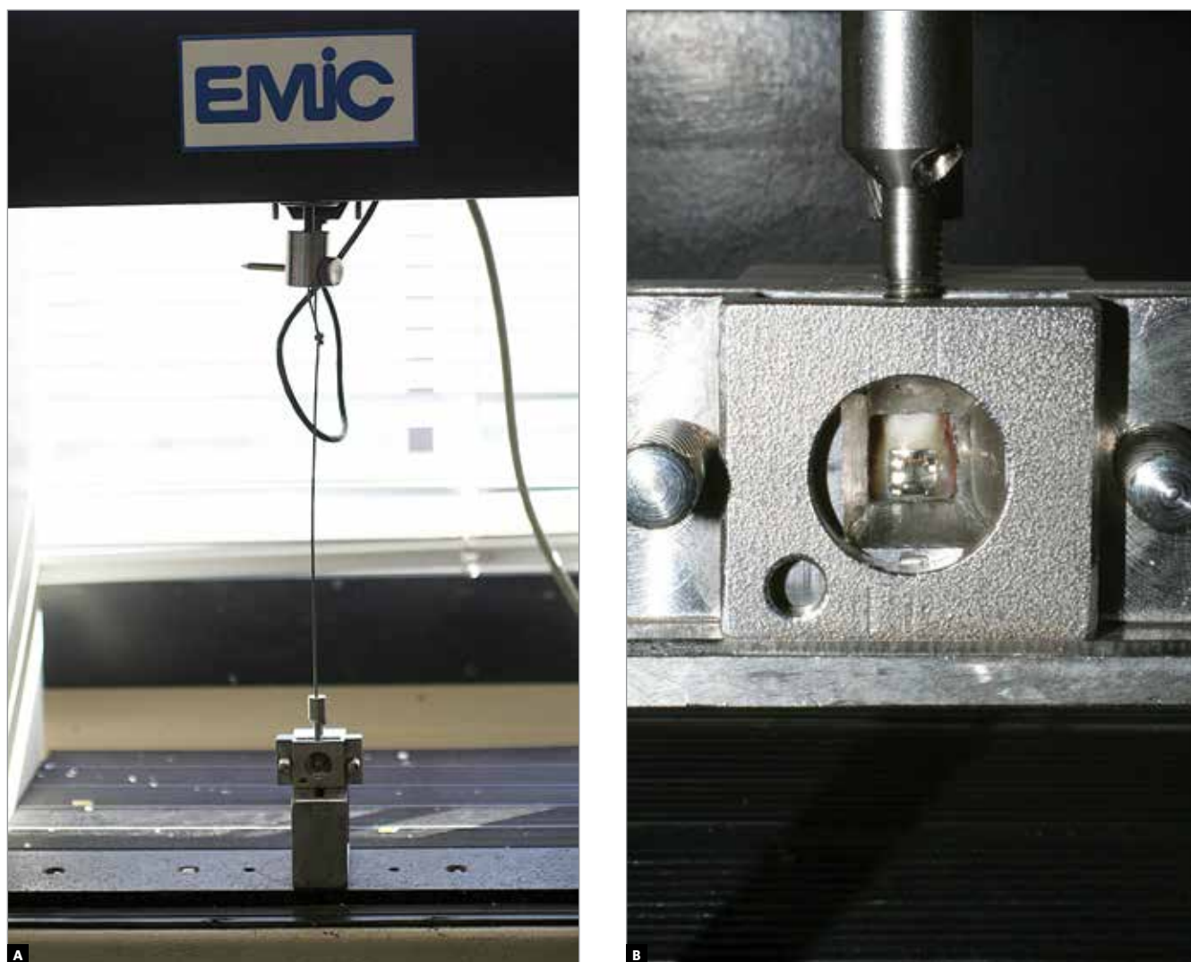
Figure 2 - Mechanical test: A) matrix used on the shear bond strength test, B) detail of the force applied in the occlusal gingival direction.
