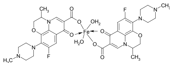
Figure 5. Probable structure of the OFX-iron(III) complex.
