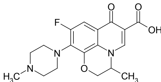
Figure 1. Chemical structure of OFX.
