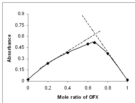
Figure 4. Continuous variation plot for OFX-iron(III) complex.
