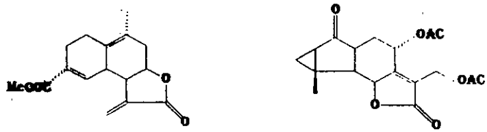
germacranolideo e scorpiolideo
