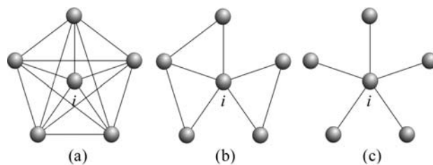
Figure 4 - Example of three networks and respective clustering coefficients (see Eq. (1)). In (a), cc_i = \frac{10(2)}{5(4)} = 1 (the vertices around i are fully connected), (b) cc_i = \frac{3(2)}{5(4)} = 0.3 and (c) cc_i = \frac{0(2)}{5(4)} = 0 . The maximum number of edges among the neighbors of i is given by k_i(k_i - 1)/2 .
