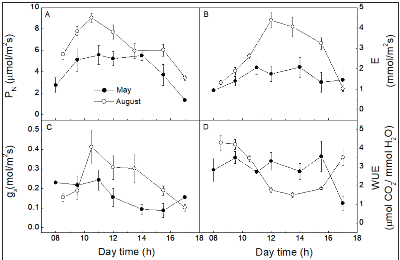
Figure 2. Diurnal courses of net CO 2 assimilation - P N (A), transpiration - E (B), stomatal conductance - g s (C) and water use efficiency - WUE (D), in gariroba palms, on May, 2012 (●) and on August, 2013 (○). Each symbol represents the mean value (± standard error) of three to six replications. Campinas, IAC, 2013.
