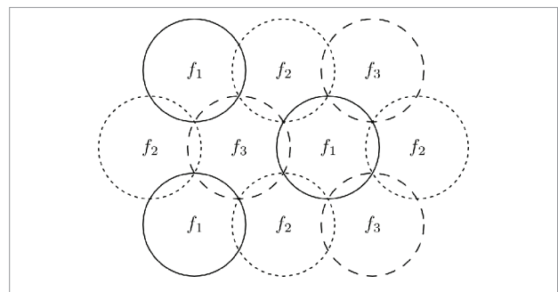
Figure 1. Frequency reuse in an idealised cellular network.
