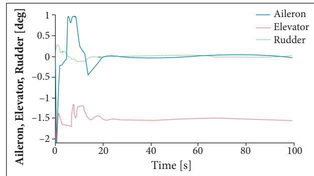
Figure 12. Control deflection of aileron, elevator and rudder.
