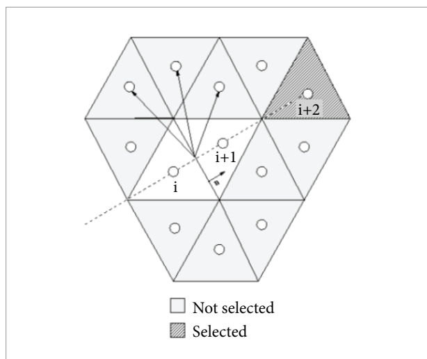
Figure 5. Search for the “ i+2 ” point inside an unstructured grid. (Scalabrin, 2007).
