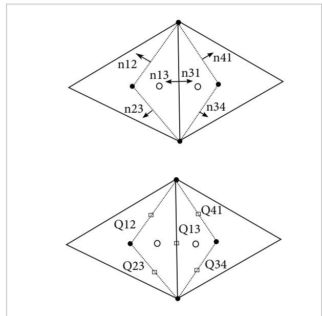
Figure 3. 2-D example of a derivative calculation.
