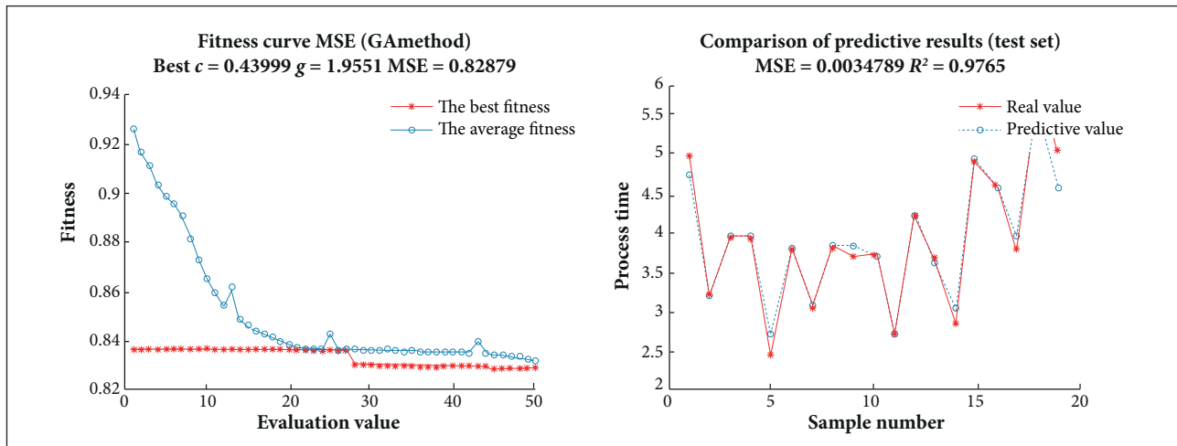
Figure 12. The optimization by GA when maxgen = 50; pop = 20.
