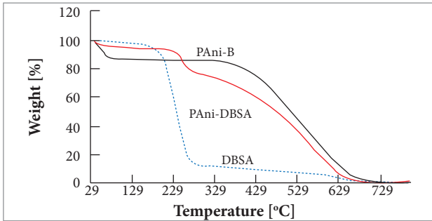
Figure 4. Thermogravimetric curves of PANi-B, PANi-DBSA, and pure DBSA.
