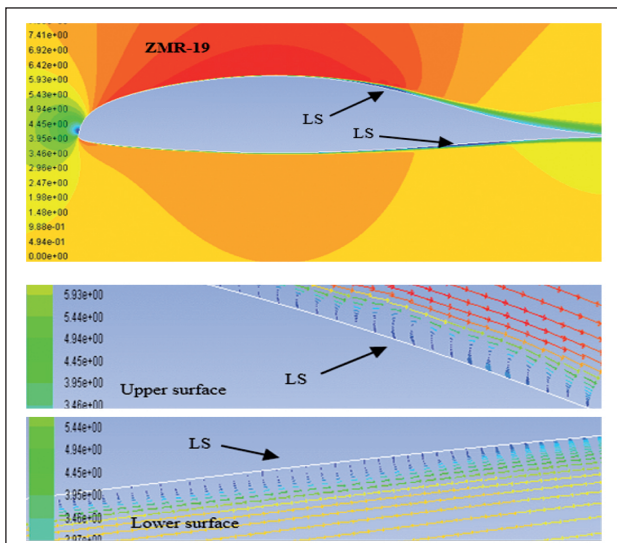
Figure 8. Velocity contour and vector at AoA = 0^\circ of ZMR-19 aerofoil.
