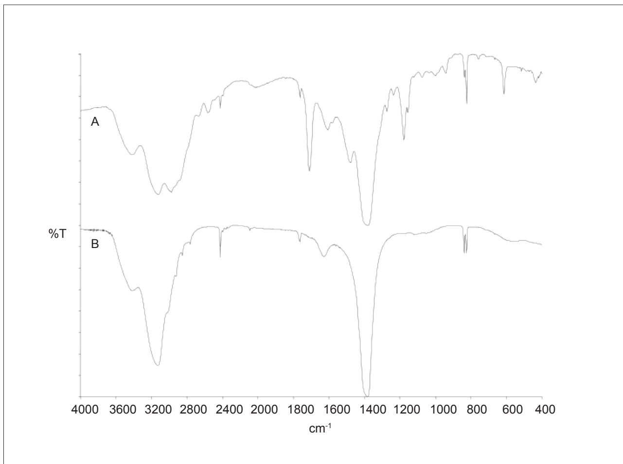
Figure 2. (A) MIR spectrum of the product obtained in synthesis 1 by using sulfamic acid: ADN 40F/20 (40 mL \text{HNO}_3 , Fuming/20 mL \text{H}_2\text{SO}_4 ); (B) MIR spectrum of ammonium nitrate – Lot n. 171169 – B. Herzog.
