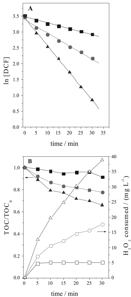
Figure 2. Influence of \text{FecitNH}_3 concentration on (A) DCF abatement kinetics, (B) TOC decay (solid symbols) and \text{H}_2\text{O}_2 consumption (open symbols), during the photo-Fenton process under solar irradiation in distilled water. Initial conditions: [\text{DCF}] = 33.4 \text{ mg L}^{-1} ( \text{TOC} = 16.8 \text{ mg C L}^{-1} ); [\text{H}_2\text{O}_2] = 68 \text{ mg L}^{-1} ; \text{pH} = 7 . ■ 0.05 \text{mmol L}^{-1} ; ● 0.1 \text{mmol L}^{-1} ; ▲ 0.2 \text{mmol L}^{-1} \text{FecitNH}_3 .
