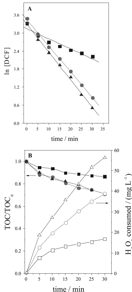
Figure 3. Influence of \text{H}_2\text{O}_2 concentration on (A) DCF abatement kinetics, (B) TOC decay (solid symbols) and \text{H}_2\text{O}_2 consumption (open symbols), during the photo-Fenton process under solar irradiation in distilled water. Initial conditions: [\text{DCF}] = 33.4 \text{ mg L}^{-1} ( \text{TOC} = 16.8 \text{ mg C L}^{-1} ); [\text{FecitNH}_3] = 0.2 \text{ mmol L}^{-1} ; \text{pH} = 7 . ■ 34 \text{mg L}^{-1} ; ● 68 \text{mg L}^{-1} ; ▲ 170 \text{mg L}^{-1} \text{H}_2\text{O}_2 .
