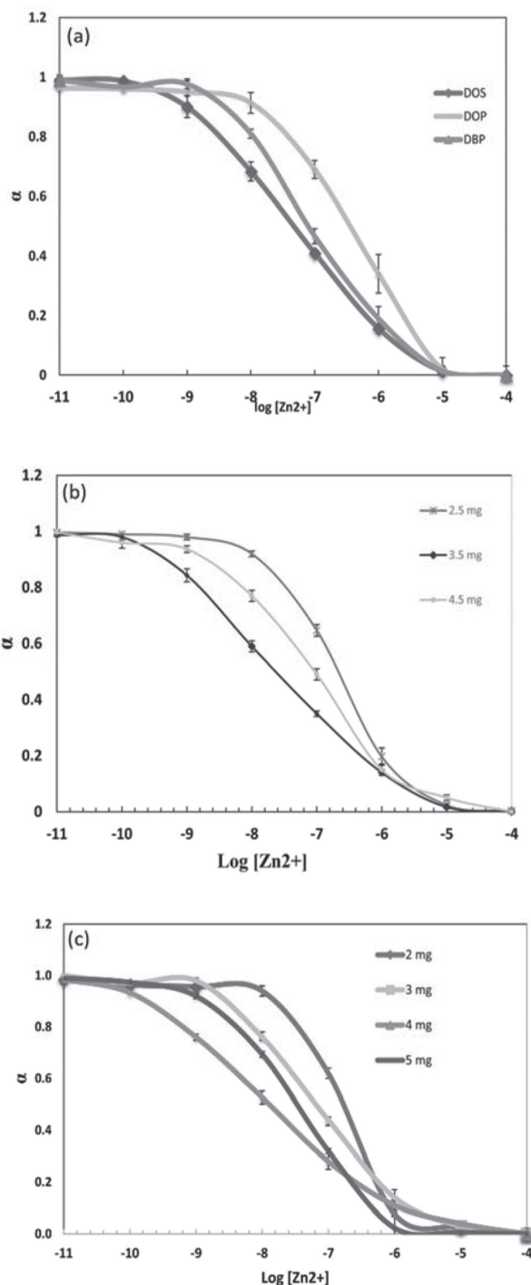
Figure 5. (a) Effect of the type of plasticizer; (b) the amount of ionophore; and (c) the amount of additive on the response of the optical sensing film in aqueous solution with pH = 5.7.
