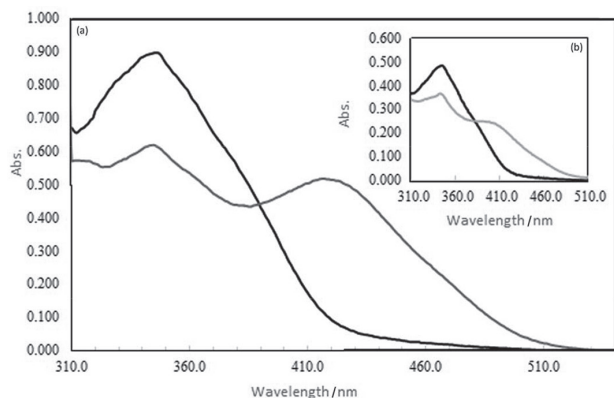
Figure 2. (a) Absorption spectra for 1 \times 10^{-5} M 5-Br salophen in the presence of Zn^{2+} ( 1 \times 10^{-6} M) at pH 5.7; (b) absorption spectra of optode film response to Zn^{2+} in the solution of 1 \times 10^{-6} M at pH 5.7.
