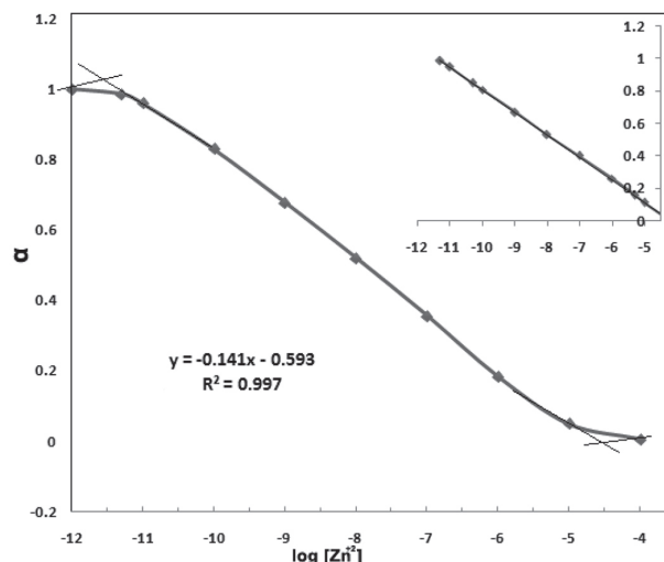
Figure 7. Response signal of the sensor to \text{Zn}^{2+} ions in buffer solution (pH = 5.7) at the optimum conditions.
