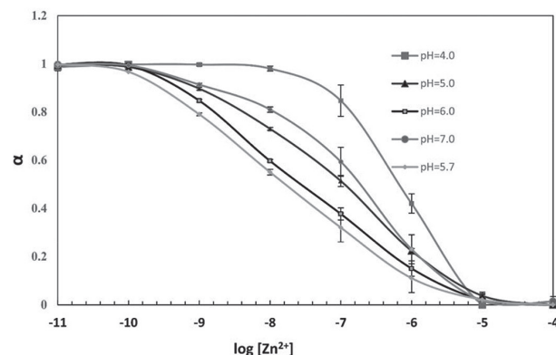
Figure 4. Effect of pH on the response of membrane in the presence of 1 \times 10^{-11} - 1 \times 10^{-4} mol L^{-1} Zn^{2+} at 345 nm; membrane composition: 3.5 mg of 5-Br salophen, 60 mg of DOS, 30 mg of PVC, 4 mg of NaTPB.
