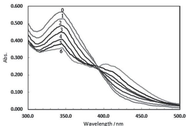
Figure 3. Absorption spectra of the optode at pH 5.7 for Zn^{2+} concentration of 1 \times 10^{-10} - 1 \times 10^{-5} M in which 1-6 refer to Zn^{2+} concentration and 0 refers to the blank solution (buffer).
