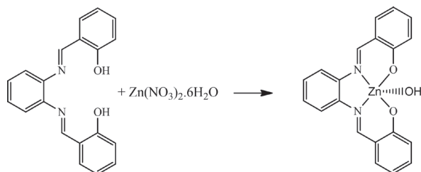
Figure 1. Reaction between 5-Br salophen and Zn^{2+} .
