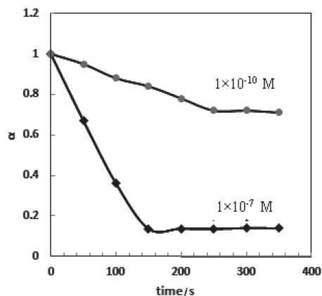
Figure 6. Response time of the optode at pH 5.7.
