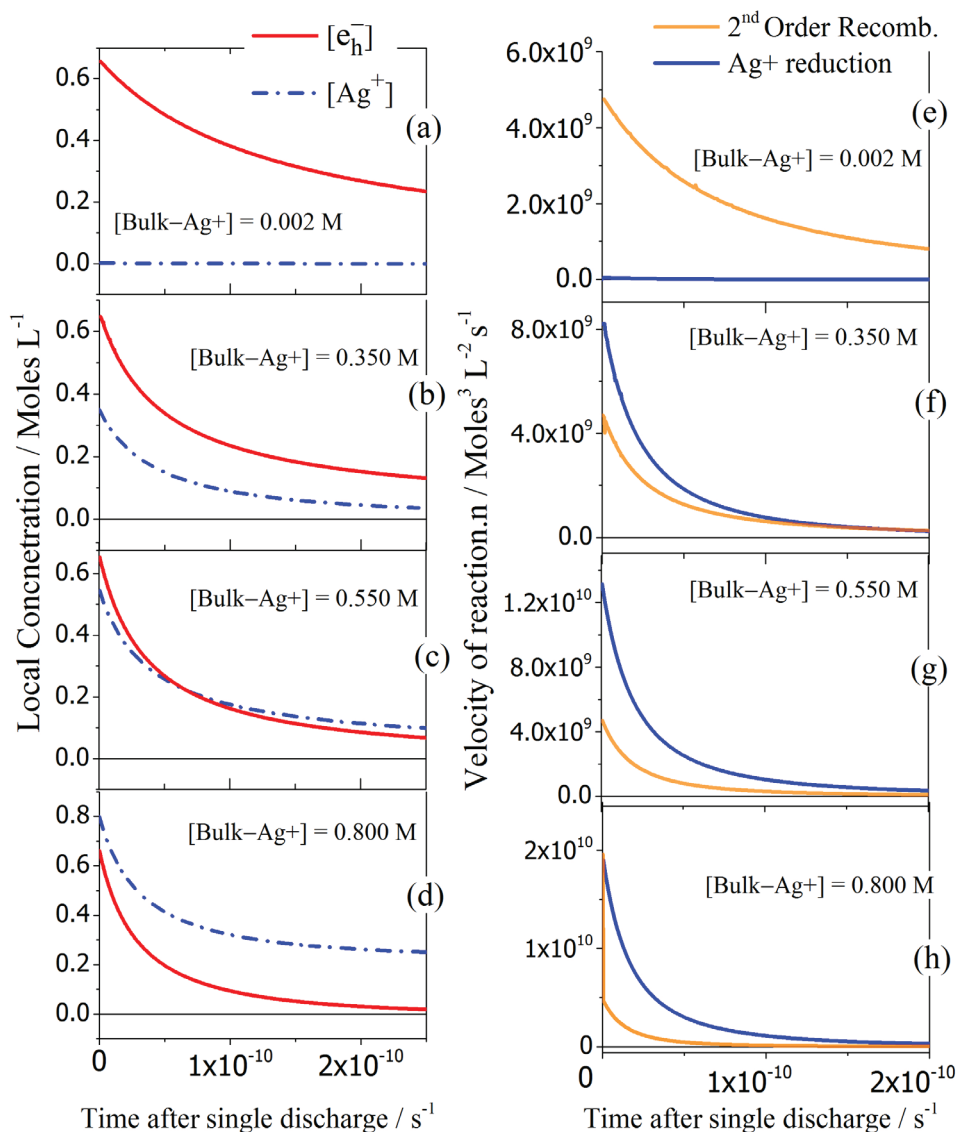
Figure 7. First column shows the temporal evolution of local concentration for the silver cations ( Ag^+ ) and hydrated electrons ( e_h^- ) obtained by computational experiments using equations 3 and 4; and considering 0.661 \text{ mol L}^{-1} as initial concentration for e_h^- combined with different initial concentration for Ag^+ : (a) 0.002 ; (b) 0.350 ; (c) 0.550 and (d) 0.800 \text{ mol L}^{-1} . Second column shows rate of reaction for silver reduction and second-order recombination reactions using 0.661 \text{ mol L}^{-1} as initial concentration for e_h^- combined with different initial concentration for Ag^+ : (e) 0.002 ; (f) 0.350 ; (g) 0.550 and (h) 0.800 \text{ mol L}^{-1} .
