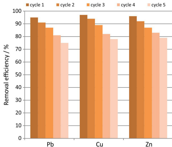
Figure 10. Removal efficiency of Pb 2+ , Cu 2+ and Zn 2+ versus number of reuse cycles.
