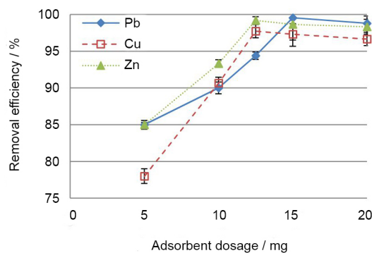
Figure 7. Effects of adsorbent dosage on removal of Pb 2+ , Cu 2+ and Zn 2+ ions by Fe 3 O 4 @MCM-41-NH 2 .
