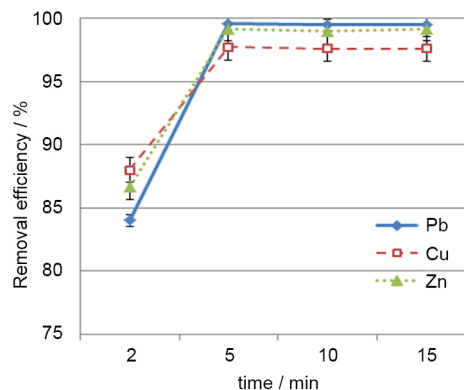
Figure 8. Effects of shaking time on removal of Pb 2+ , Cu 2+ and Zn 2+ ions by Fe 3 O 4 @MCM-41-NH 2 .
