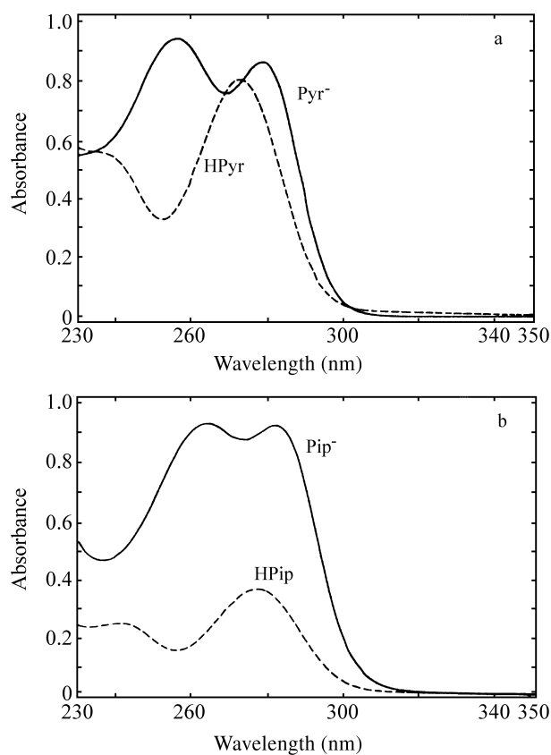
Figure 2. The Pyr(2a) and Pip(2b) spectra in acid (pH = 0.98) and basic (pH = 7.82) media.
