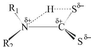
Figure 1. The acid decomposition intermediate, according to Joris et al. 13 .
