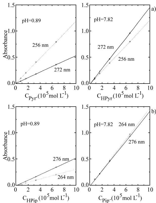
Figure 3. The Lambert-Beer law verification, in the \lambda_{\max} of the acid and basic forms of each DTC (3a - Pyr and 3b - Pip). The angular coefficients of these curves gave the \epsilon_A, \text{RSH} , \epsilon_B, \text{RSH} , \epsilon_A, \text{RS}^- , and \epsilon_B, \text{RS}^- values.
