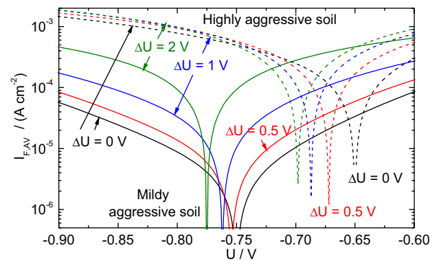
Figure 5. Digitally simulated polarization curves modified by faradaic rectification with various \Delta U values (indicated with arrows). Solid lines for mildly aggressive soil with the corrosion kinetic parameters in Table 2, and dashed lines for highly aggressive soil with the corrosion kinetic parameters in Table 3.
