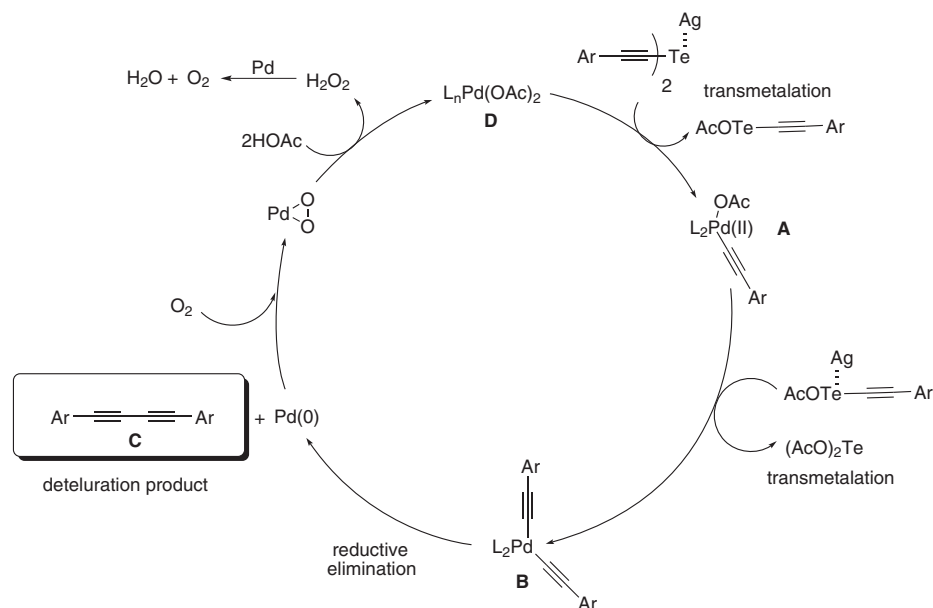
Figure 2. Possible catalytic cycle of the homocoupling reaction of alkyne tellurides.
