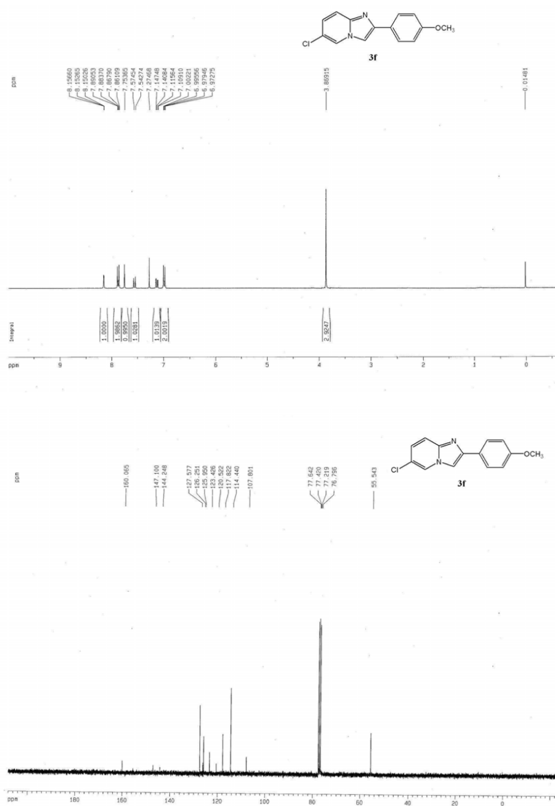
Figure S6. 1 H NMR of 3f (300 MHz, CDCl 3 ) and 13 C NMR of 3f (75 MHz, CDCl 3 ).
