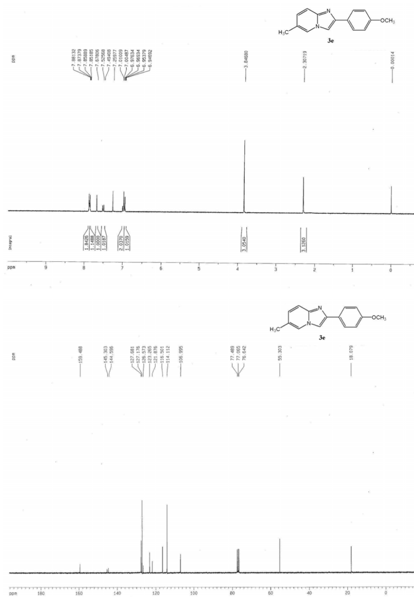
Figure S5. ^1\text{H} NMR of 3e (300 MHz, \text{CDCl}_3 ) and ^{13}\text{C} NMR of 3e (75 MHz, \text{CDCl}_3 ).
