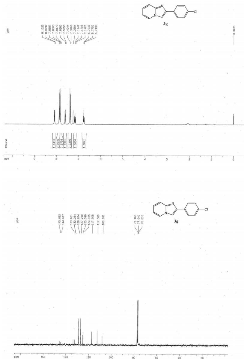
Figure S7. ^1\text{H} NMR of 3g (300 MHz, \text{CDCl}_3 ) and ^{13}\text{C} NMR of 3g (75 MHz, \text{CDCl}_3 ).
