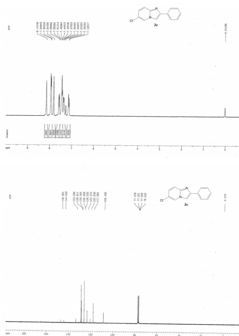
Figure S3. 1 H NMR of 3c (300 MHz, CDCl 3 ) and 13 C NMR of 3c (75 MHz, CDCl 3 ).
