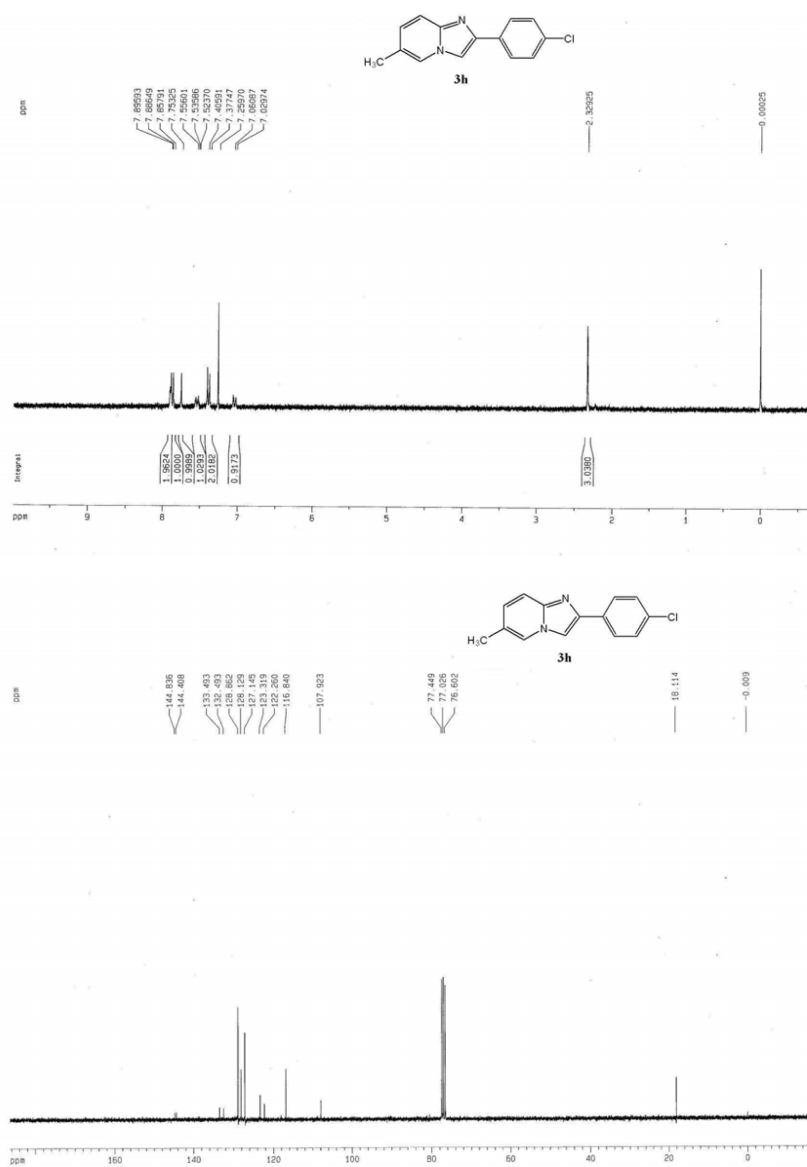
Figure S8. 1 H NMR of 3h (300 MHz, CDCl 3 ) and 13 C NMR of 3h (75 MHz, CDCl 3 ).
