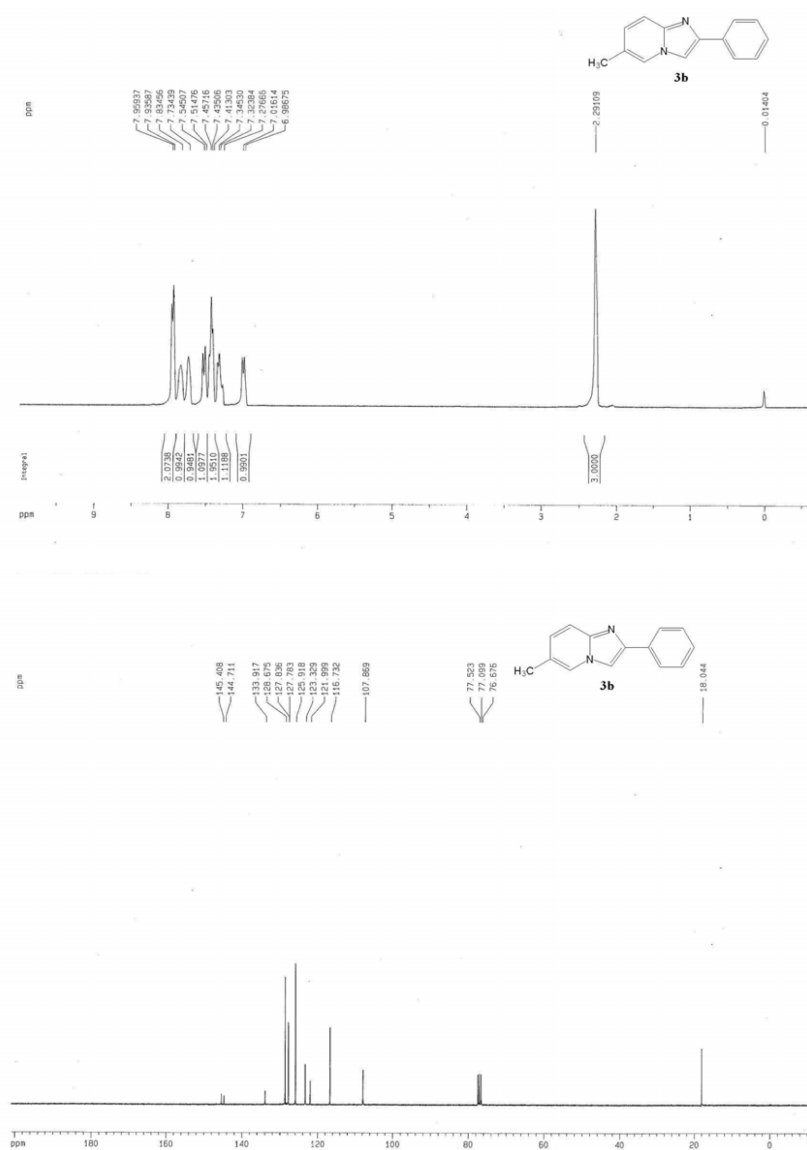
Figure S2. 1 H NMR of 3b (300 MHz, CDCl 3 ) and 13 C NMR of 3b (75 MHz, CDCl 3 ).
