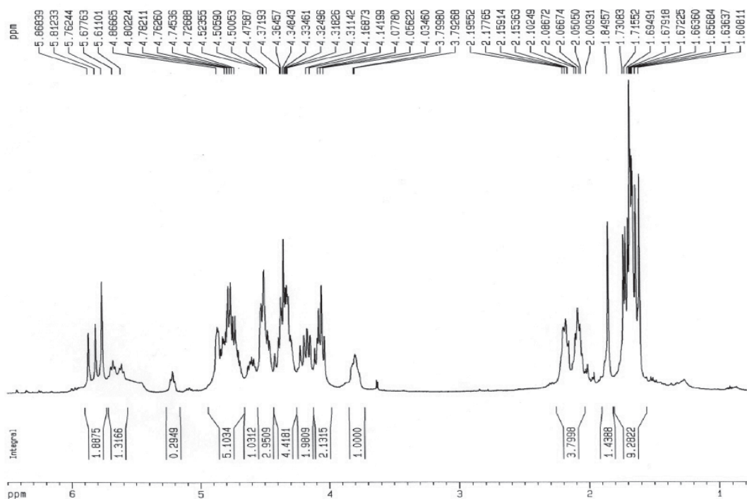
Figure S18. ^1H NMR spectrum (400 MHz, C_5D_5N ;TMS) of OGSA o1.
