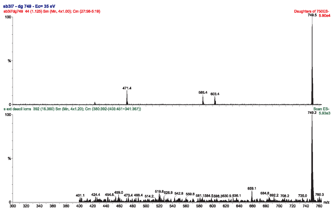
Figure S24. ESI-MS and ESI-MS/MS of s4.
