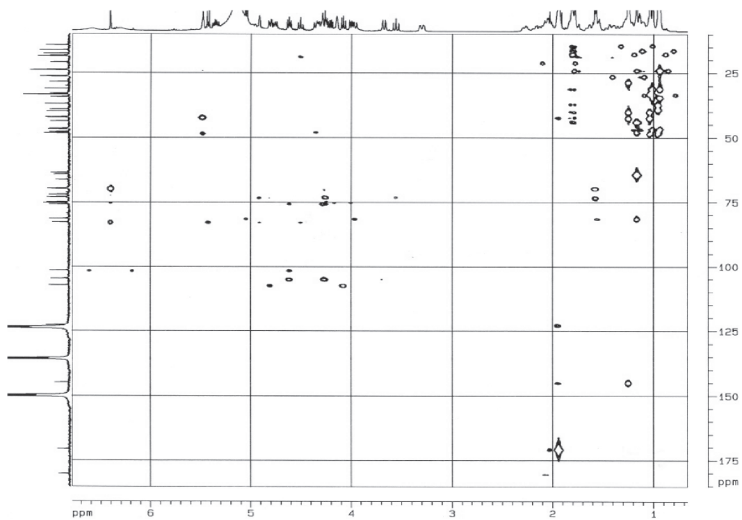
Figure S9. HMBC NMR experiment (400 MHz, C 5 D 5 N;TMS) of SAP s1-1b.
