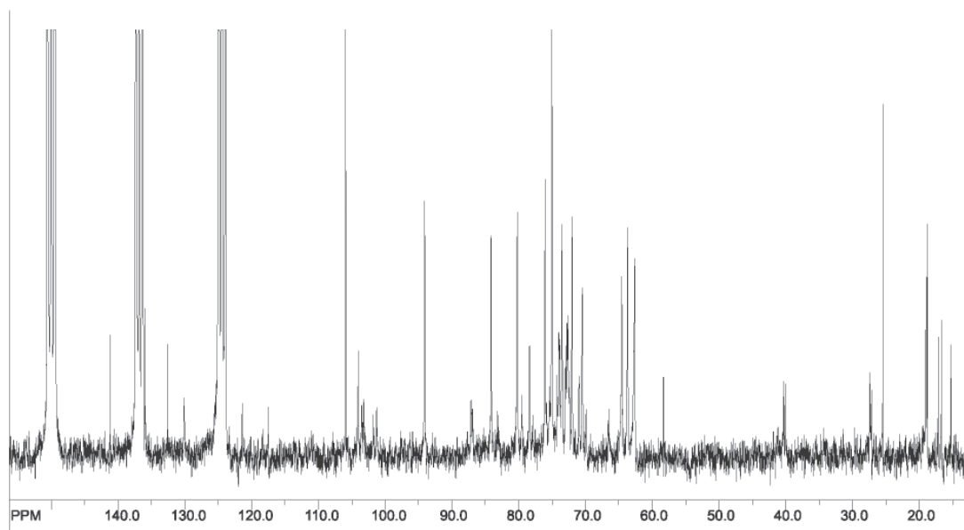
Figure S2. 13 C NMR spectrum (50 MHz, C 5 D 5 N;TMS) of an OGSA mixture.
