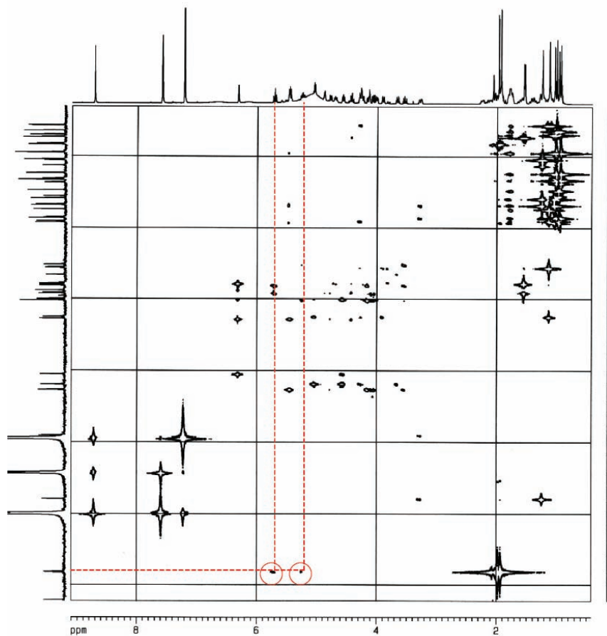
Figure S17. HMBC NMR experiment (400 MHz, C_5D_5N ;TMS) of SAP s1-2a.
