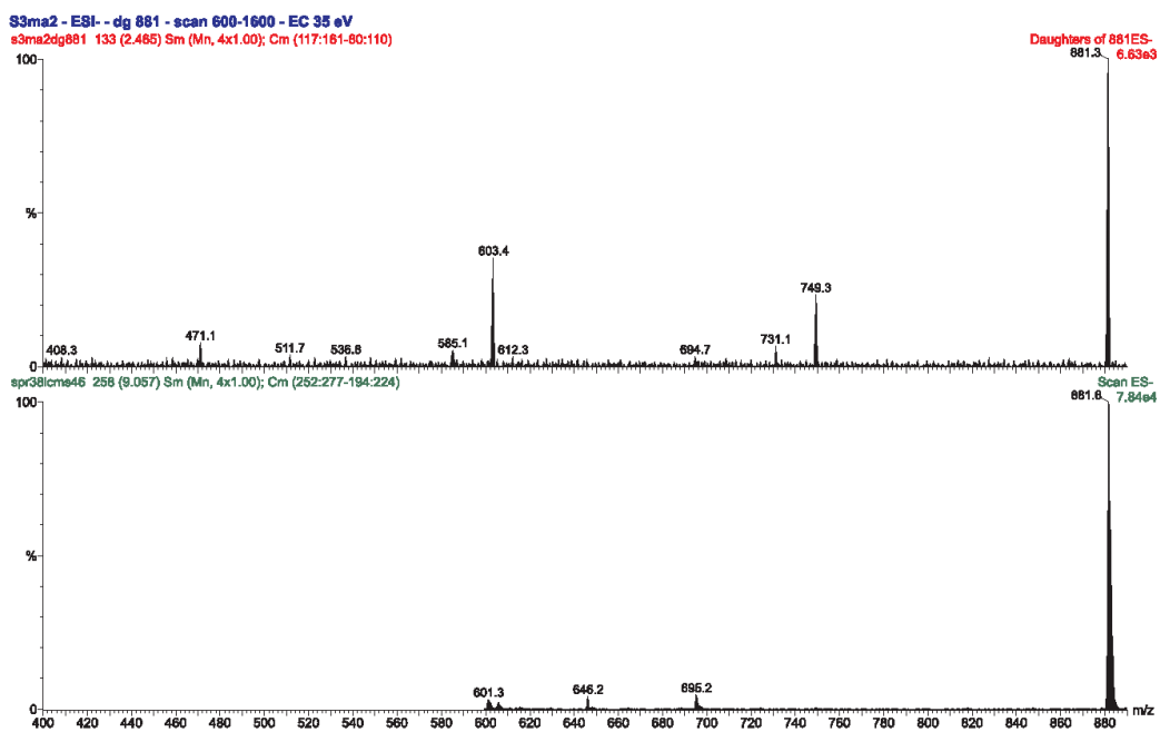
Figure S26. ESI-MS and ESI-MS/MS of s1, s2 and s3.
