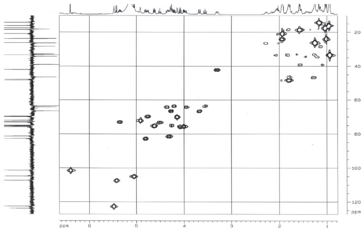
Figure S8. HSQC NMR experiment (400 MHz, \text{C}_5\text{D}_5\text{N} ;TMS) of SAP s1-1b.
