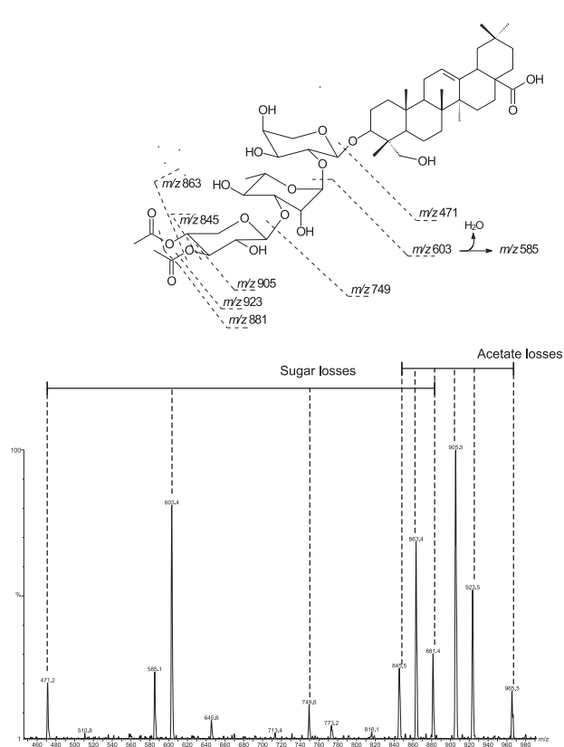
Figure 3. Product ion spectrum obtained by CID (35 eV) of the precursor ion at m/z 965 produced by electrospray ionisation of SAP s1-2a , and suggestion for the origin of the fragments in this spectrum.
