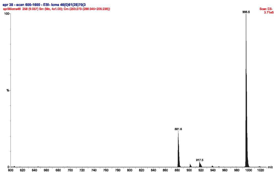
Figure S29. ESI-MS of SAP Hed-ara-rha-glc w/ 2 OAc.
