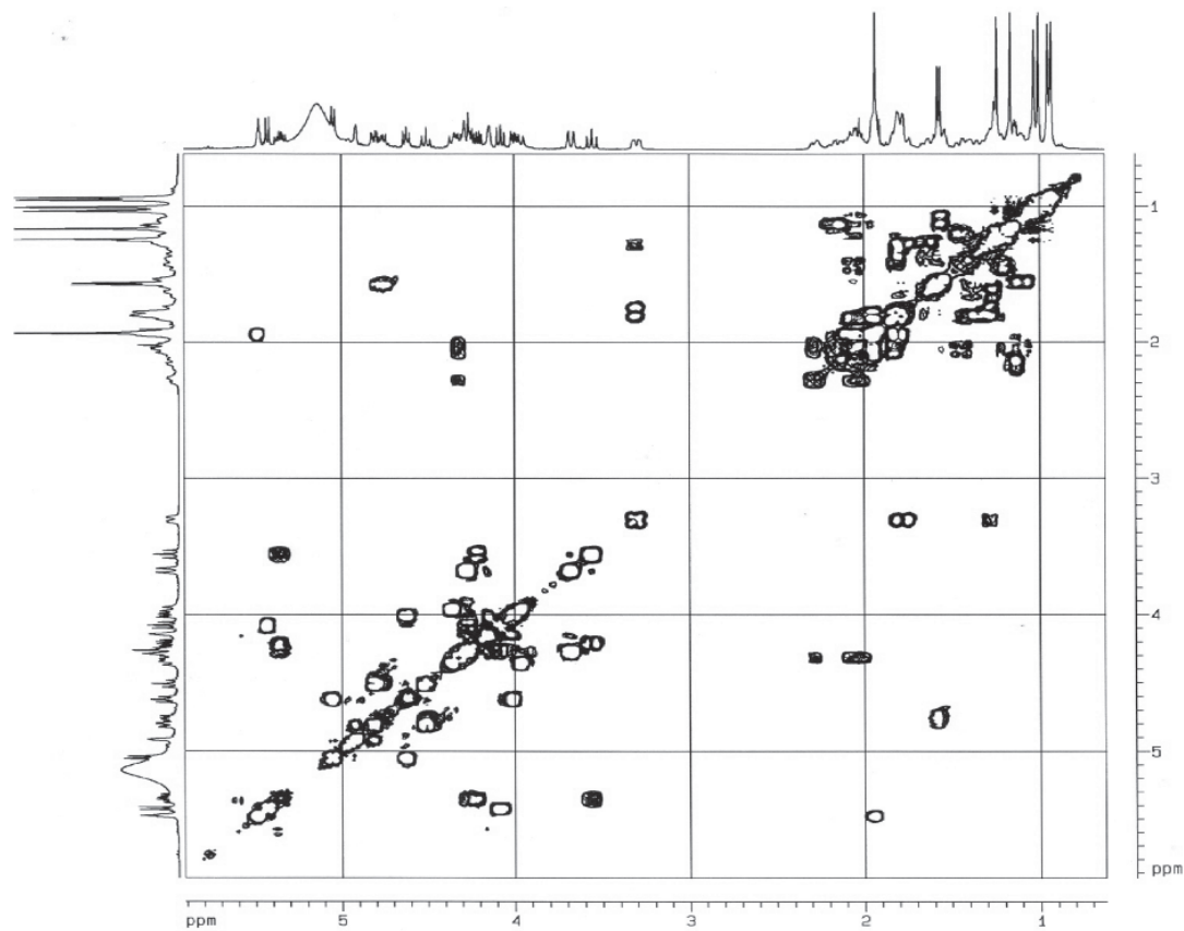
Figure S7. ^1\text{H} - ^1\text{H} COSY NMR experiment (400 MHz, \text{C}_5\text{D}_5\text{N} ;TMS) of SAP s1-1b.
