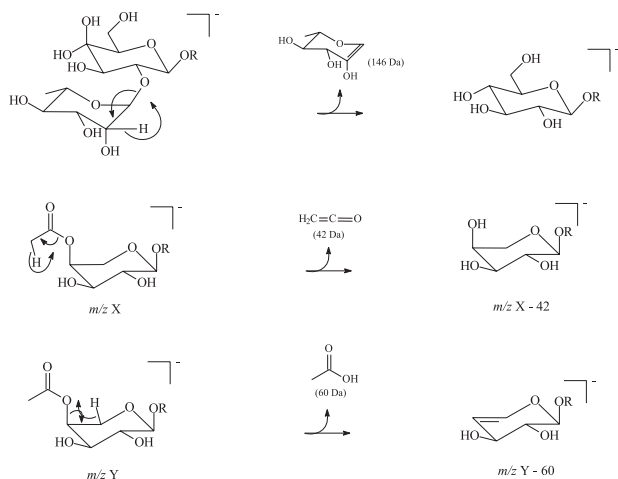
Scheme 1. Suggested general mechanism for the fragmentation of free or acetylated sugar chain in SAPs and ASOGs.
