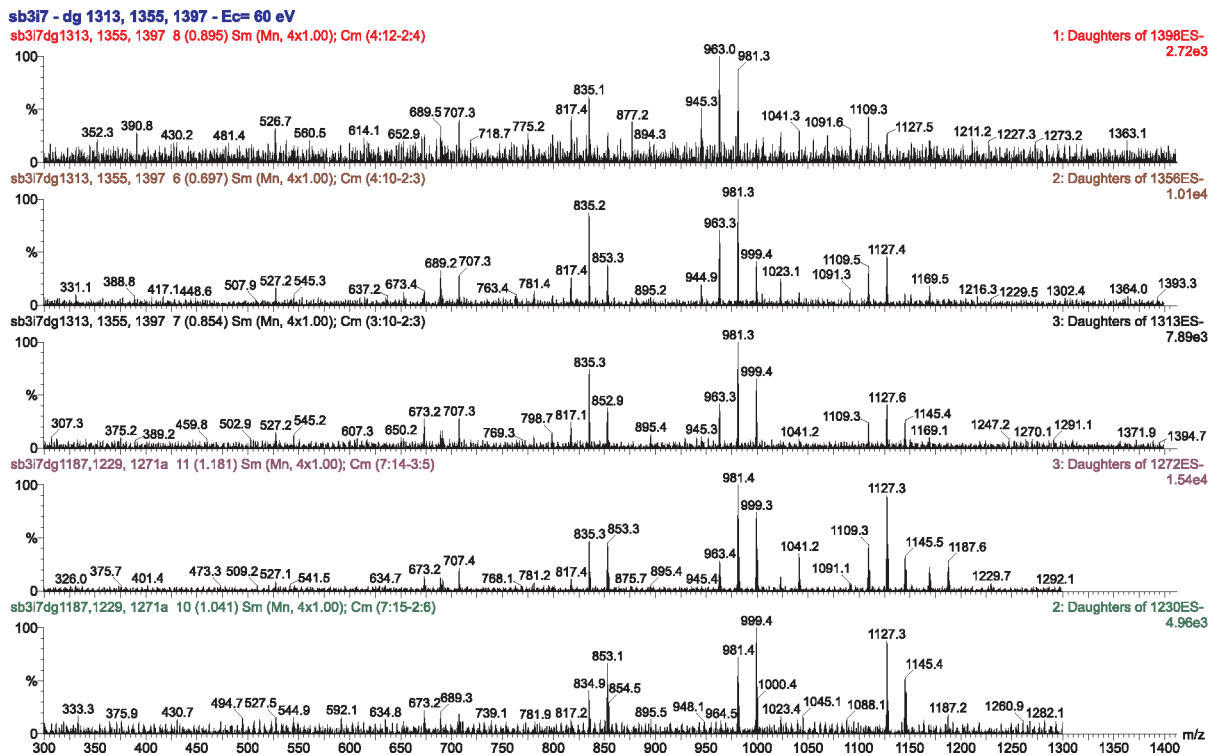
Figure S34. ESI-MS/MS of OGSA a1 w/ 2-6 OAc.
