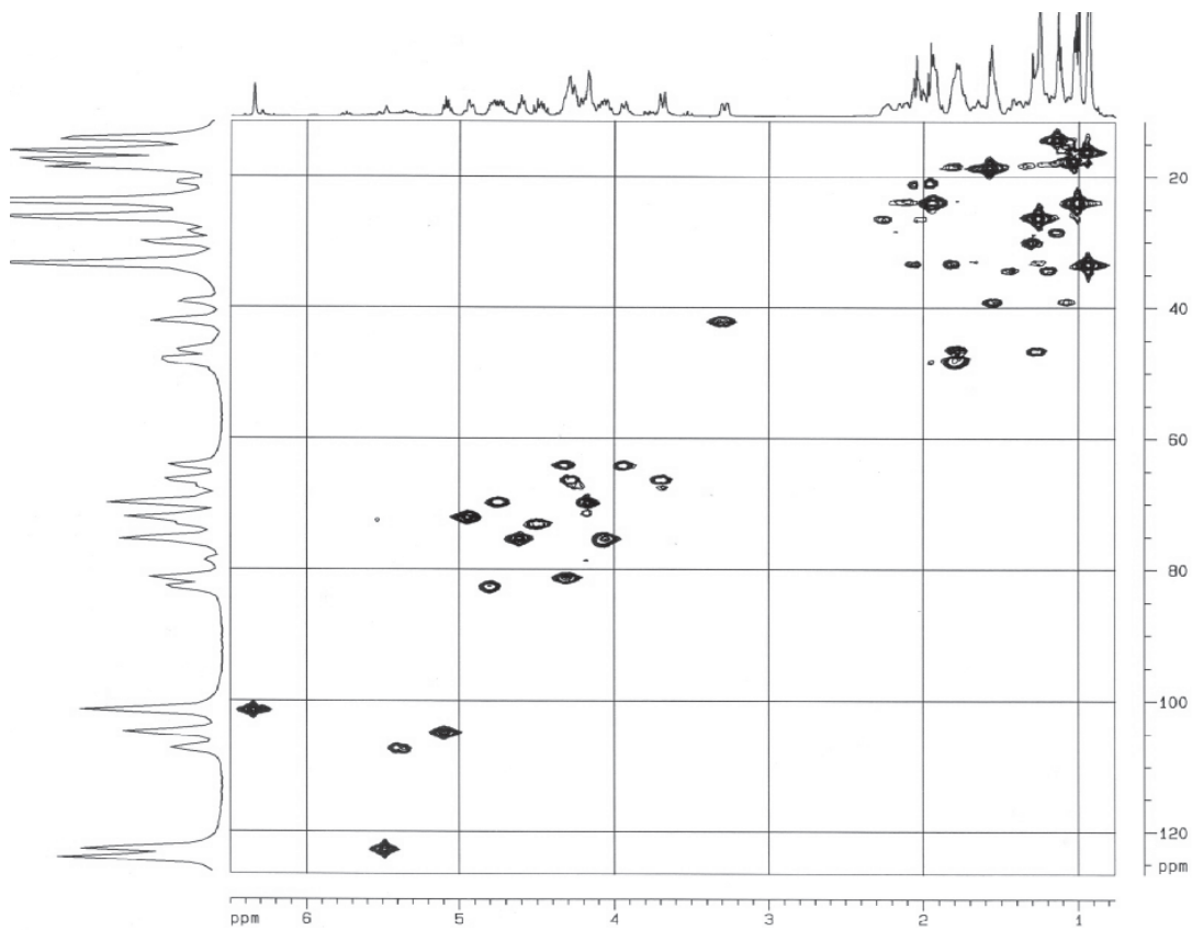
Figure S4. HSQC NMR experiment (400 MHz, \text{C}_5\text{D}_5\text{N} ; TMS) of a SAP mixture (s1, s2 and s3).
