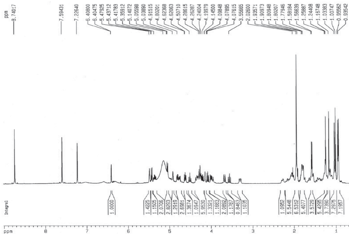
Figure S5. ^1\text{H} NMR spectrum (400 MHz, \text{C}_3\text{D}_3\text{N} ;TMS) of SAP s1-1b.
