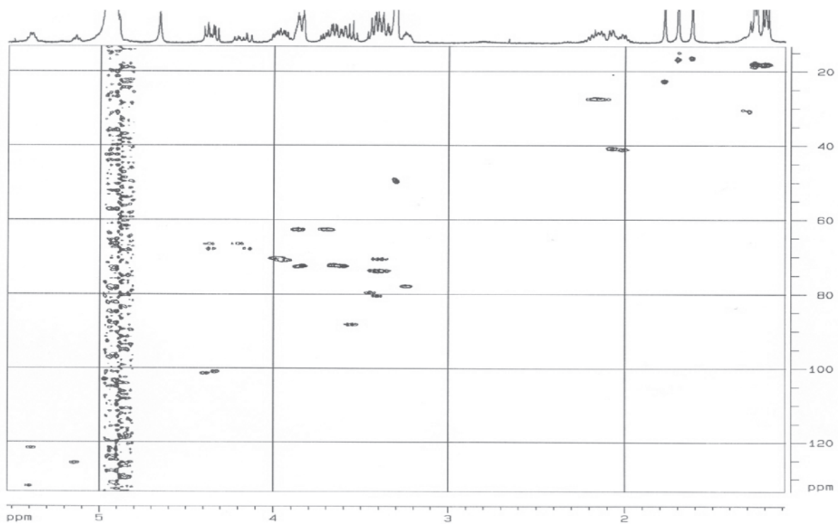
Figure S21. HSQC NMR experiment (400 MHz, CD 3 OD) of OGSA o1.
