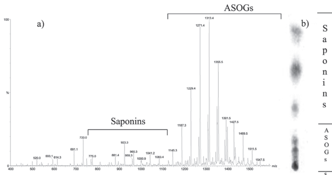
Figure 1. ESI-MS (a) and TLC (b) of an extract obtained from young fruits of S. saponaria .
