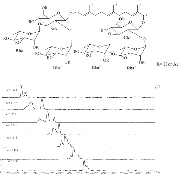
Figure 6. Selected ion recorded chromatograms for acetylated ASOGs obtained by electrospray ionization in the negative ion mode.
