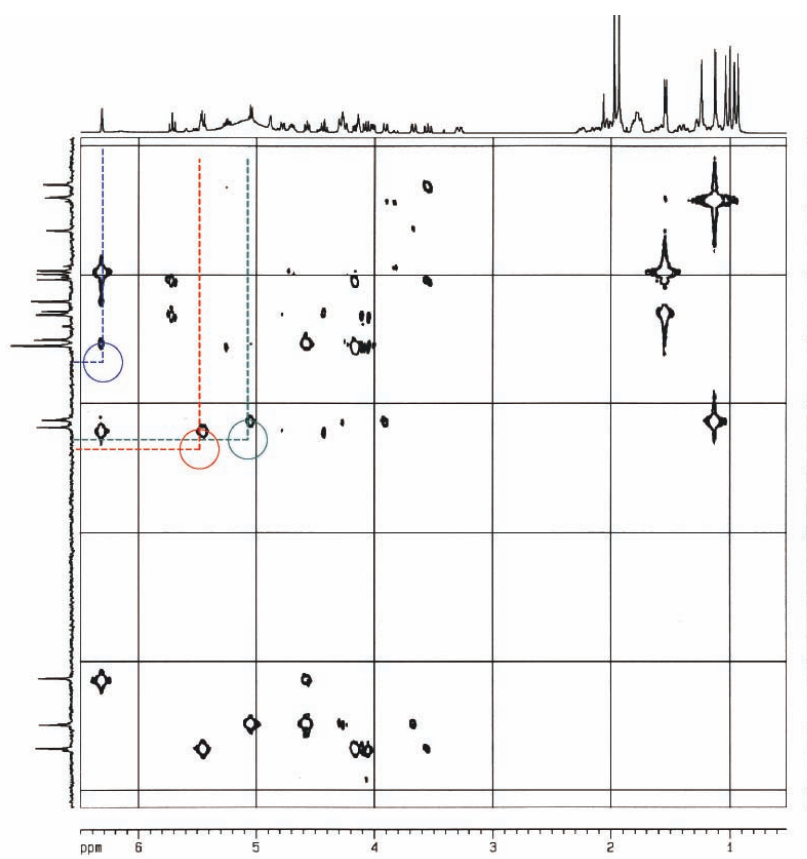
Figure S16. HMBC NMR experiment (400 MHz, \text{C}_3\text{D}_5\text{N} ;TMS) of SAP s1-2a. Expansion.
