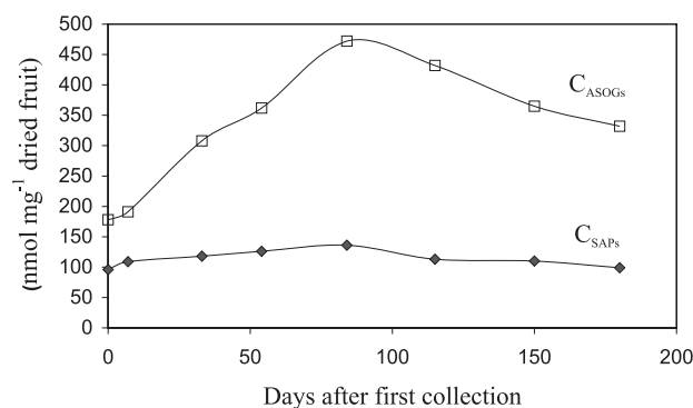
Figure 7. Variation of the concentration of ASOGs and SAPs in dried fruits of S. saponaria , during fruit maturation.
