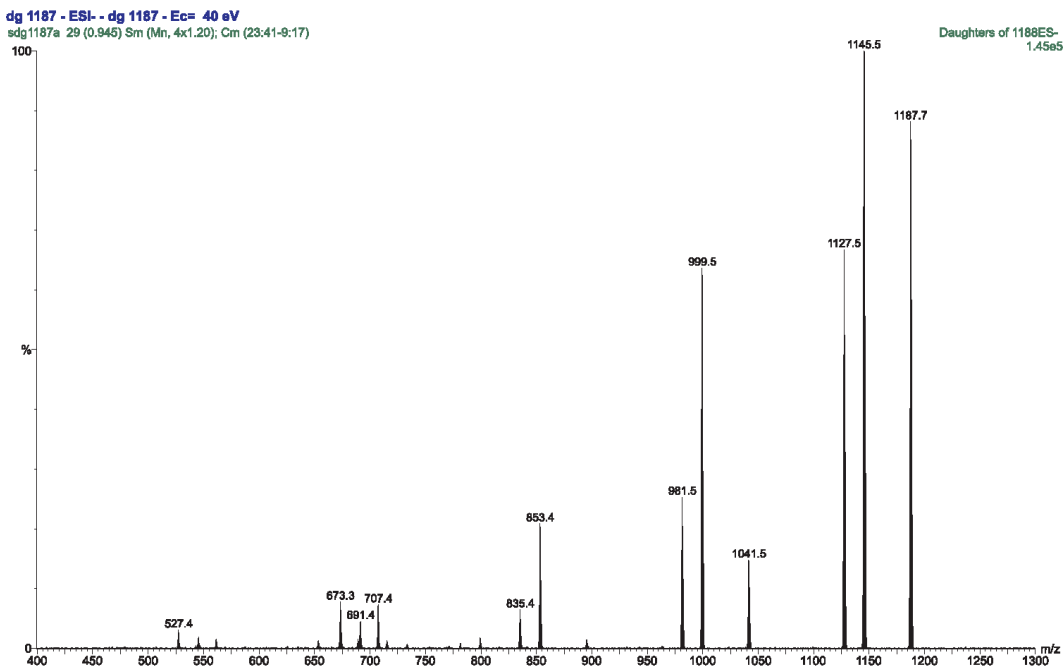
Figure S33. ESI-MS/MS of OGSA a1 w/ 1 OAc.
