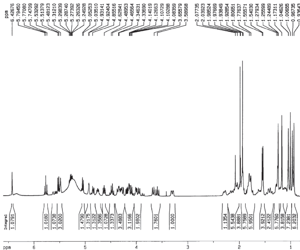
Figure S11. ^1\text{H} NMR spectrum (400 MHz, \text{C}_5\text{D}_5\text{N} ;TMS) of SAP s1-2a.
