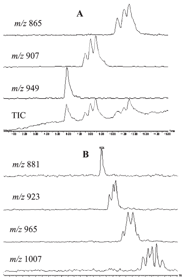
Figure 4. Selected ion recorded chromatograms of acetylated oleanolic acid (A) and hederagenin (B) derived SPAs obtained by electrospray ionization.
