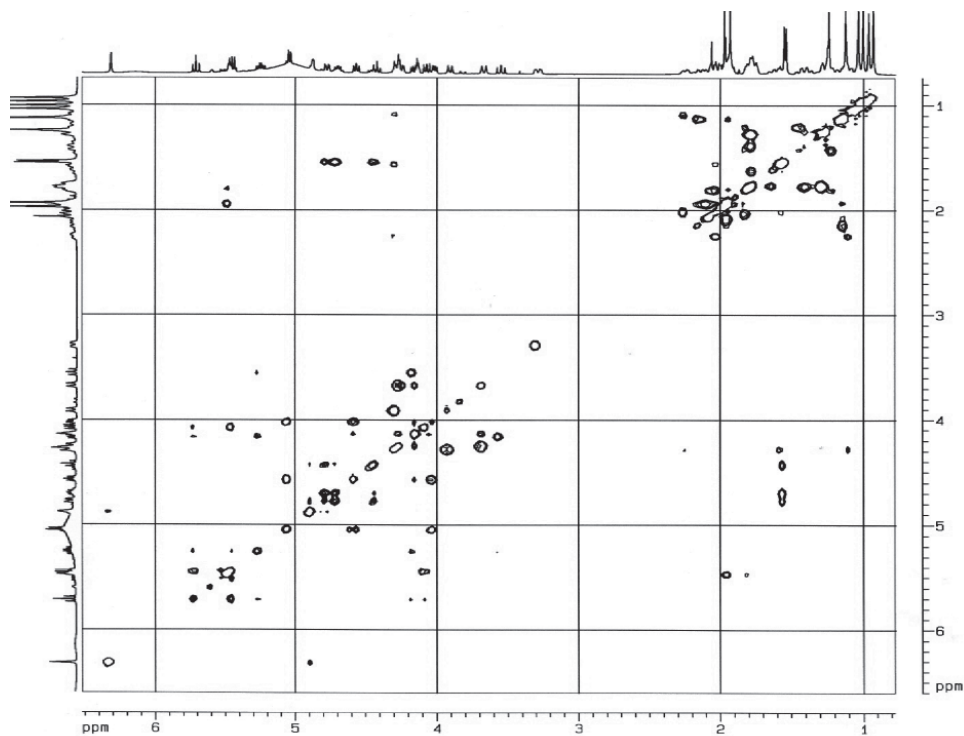
Figure S14. ^1\text{H} – ^1\text{H} TOCSY NMR experiment (400 MHz, mixing time = 55ms, \text{C}_5\text{D}_5\text{N} ;TMS) of SAP s1-2a.
