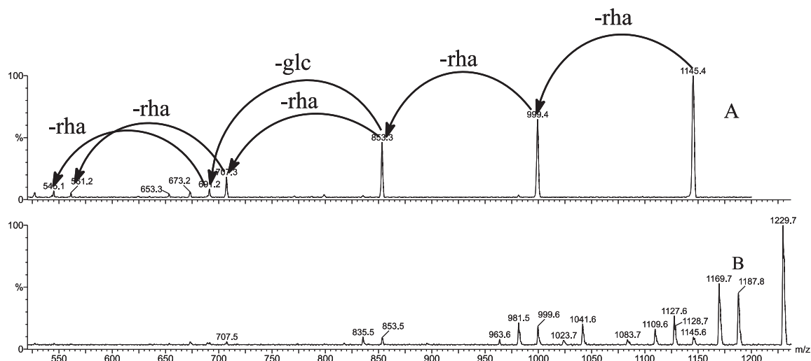
Figure 5. CID spectrum of the precursor ion at m/z 1145 [M-H]^- obtained by electrospray ionization of a1 (A) and ESI-MS of an a1 diacetate (B) showing [M-H]^- at m/z 1229. Structure of a1 is shown in Table 2.
