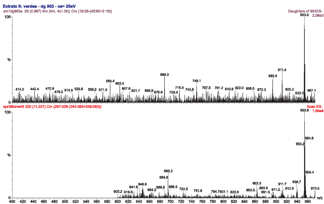
Figure S28. ESI-MS and ESI-MS/MS of SAP Hed-ara-rha-glc w/ 1 OAc.
