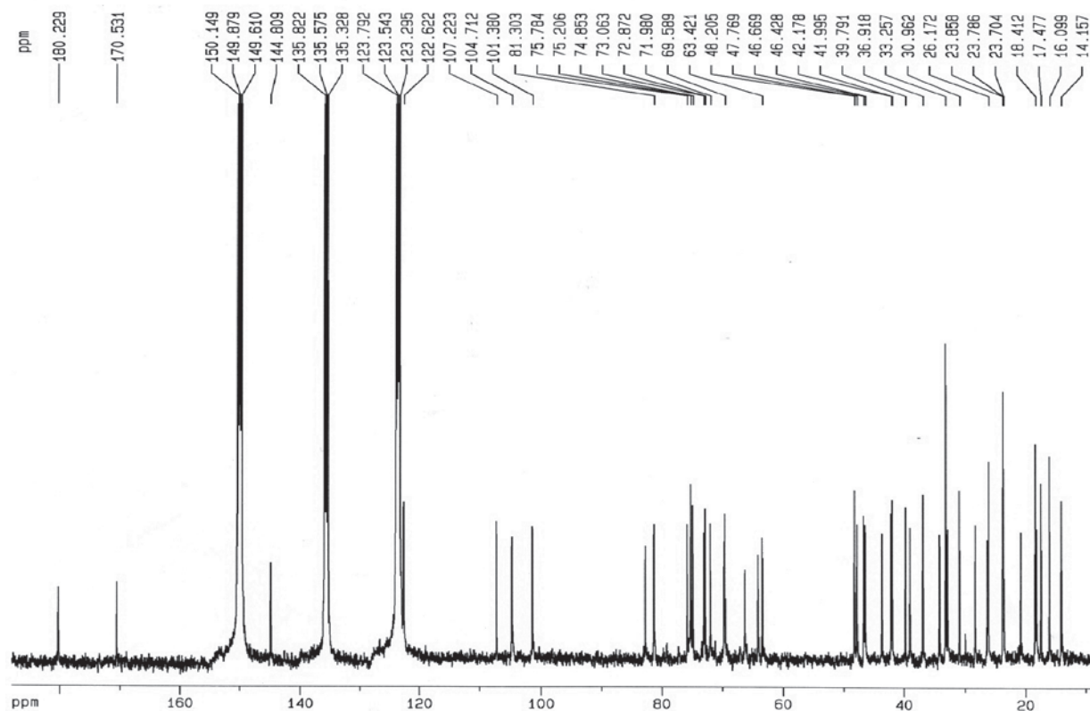
Figure S6. ^{13}\text{C} NMR spectrum (100 MHz, \text{C}_3\text{D}_3\text{N} ;TMS) of SAP s1-1b.
