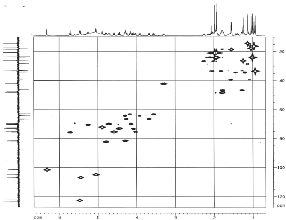
Figure S15. HSQC NMR experiment (400 MHz, \text{C}_3\text{D}_5\text{N} ;TMS) of SAP s1-2a.
