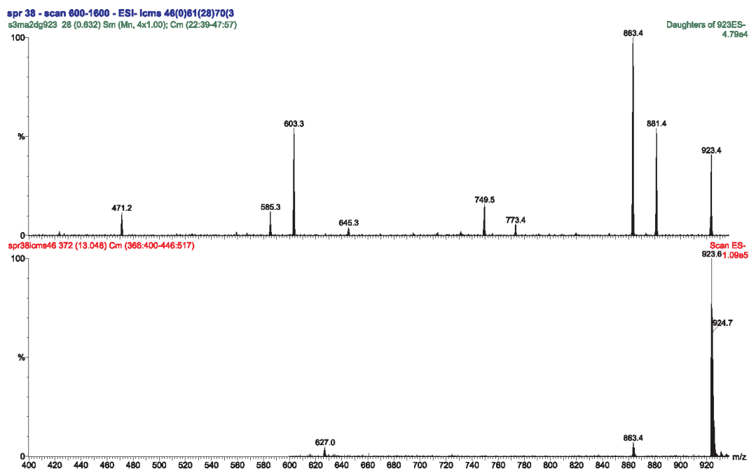
Figure S25. ESI-MS and ESI-MS/MS of s1-1a and s1-1b.
