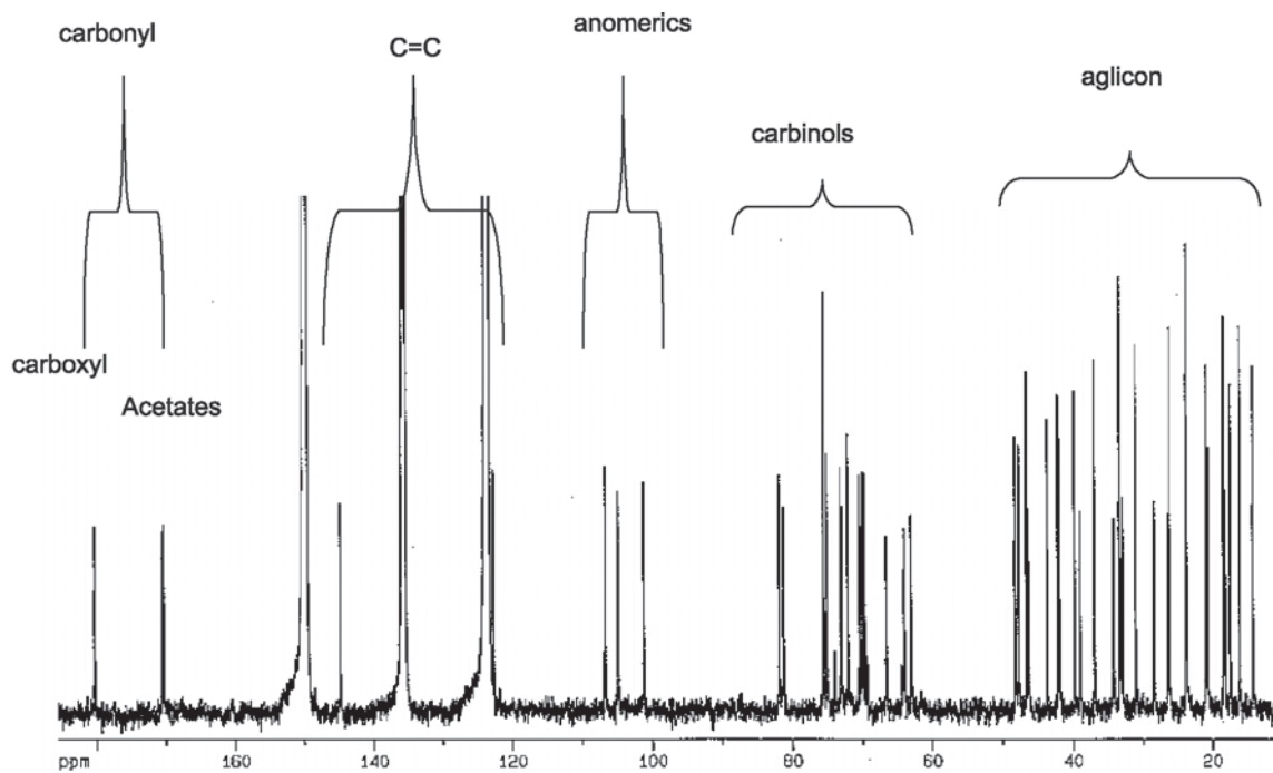
Figure S12. A Typical ^{13}\text{C} NMR spectrum (400 MHz, \text{C}_5\text{D}_5\text{N} ;TMS) of a SAP (s1-2a).
