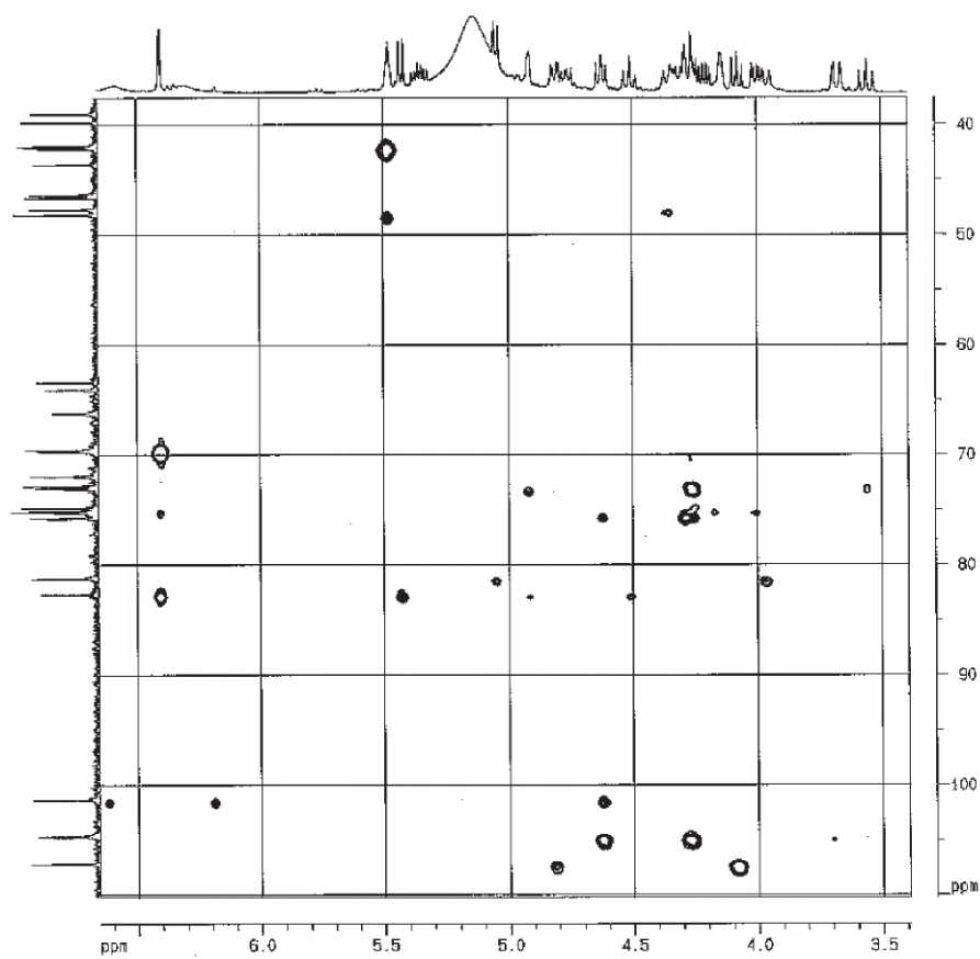
Figure S10. HMBC NMR experiment (400 MHz, C 5 D 5 N;TMS) of SAP s1-1b. Expansion.
