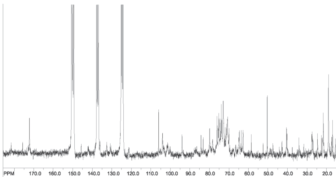
Figure S1. 13 C NMR spectrum (50 MHz, C 5 D 5 N;TMS) of a SAP mixture.
