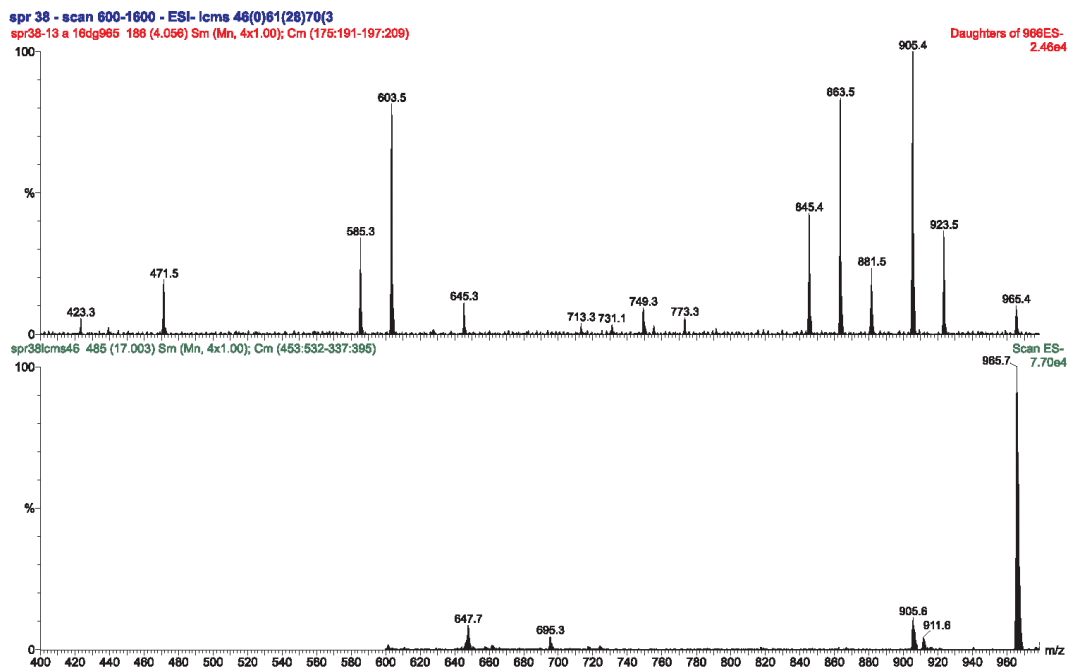
Figure S27. ESI-MS and ESI-MS/MS of s1-2a.
