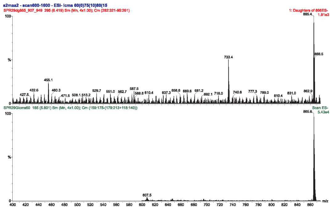
Figure S30. ESI-MS and ESI-MS/MS of s5 or s6.
