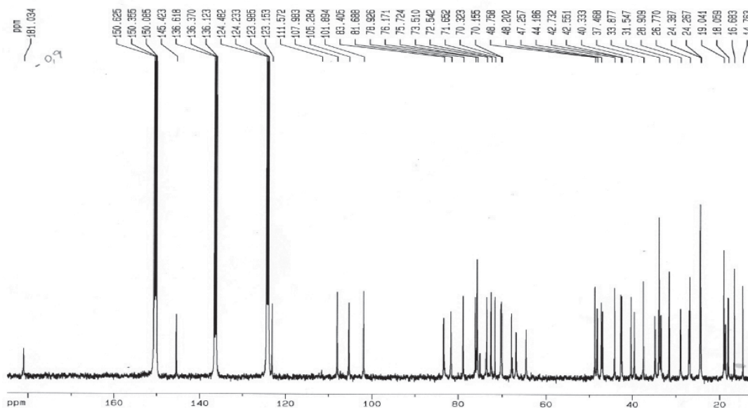
Figure S3. ^{13}\text{C} NMR spectrum (100 MHz, \text{C}_5\text{D}_5\text{N} ; TMS) of a SAP mixture (s1, s2 and s3).
