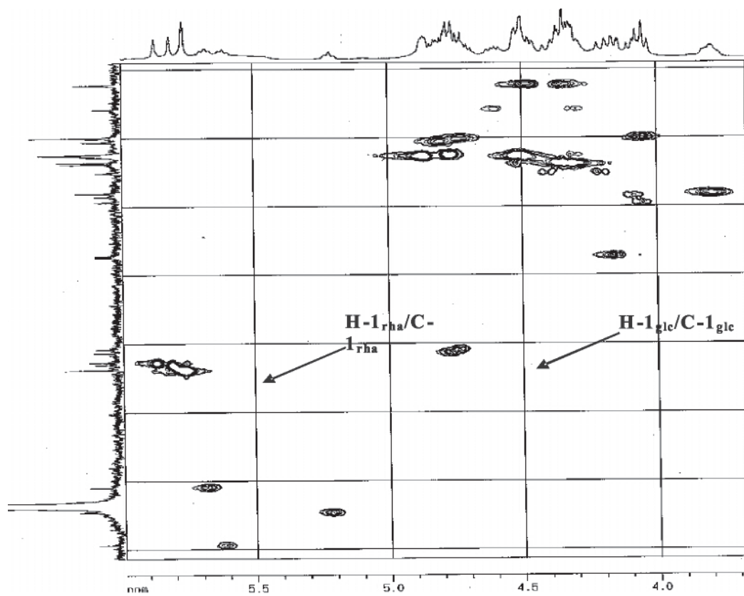
Figure S22. HSQC NMR experiment (400 MHz, C 3 D 5 N) of OGSA o1.
