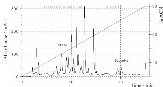
Figure 2. Chromatogram (UV, 205 nm) of a crude methanol extract obtained from fruits of S. saponaria (Same sample used to obtain the mass spectrum shown in Figure 1).
