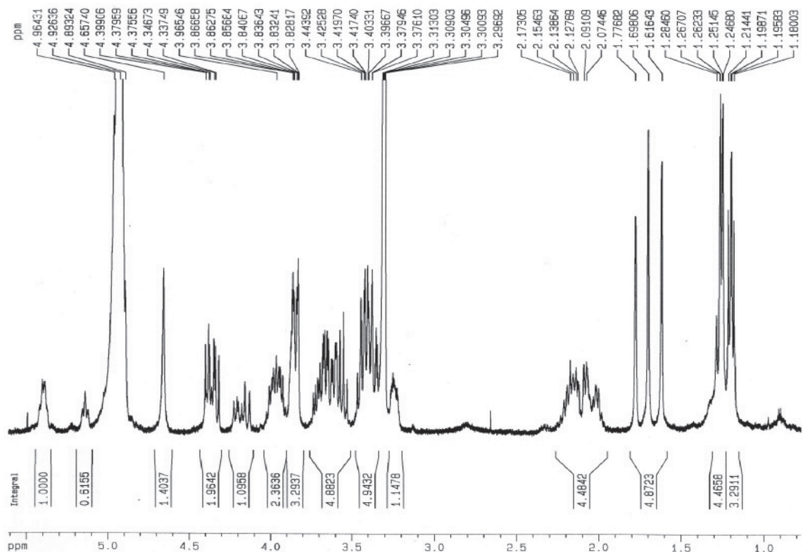
Figure S19. 1 H NMR spectrum (400 MHz, CD 3 OD) of OGSA o1.
