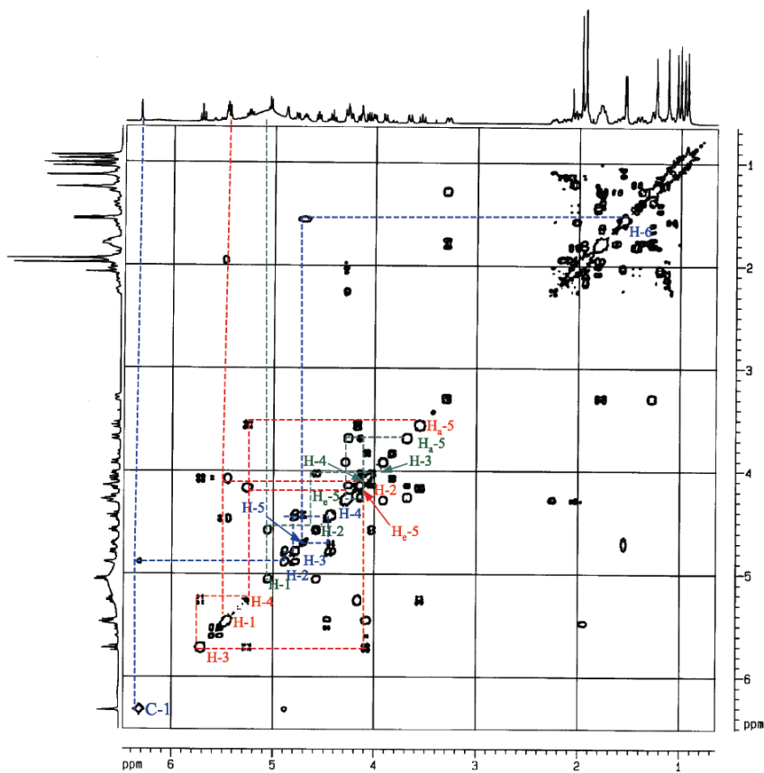
Figure S13. ^1\text{H} – ^1\text{H} COSY NMR experiment (400 MHz, \text{C}_5\text{D}_5\text{N} ;TMS) of SAP s1-2a.
