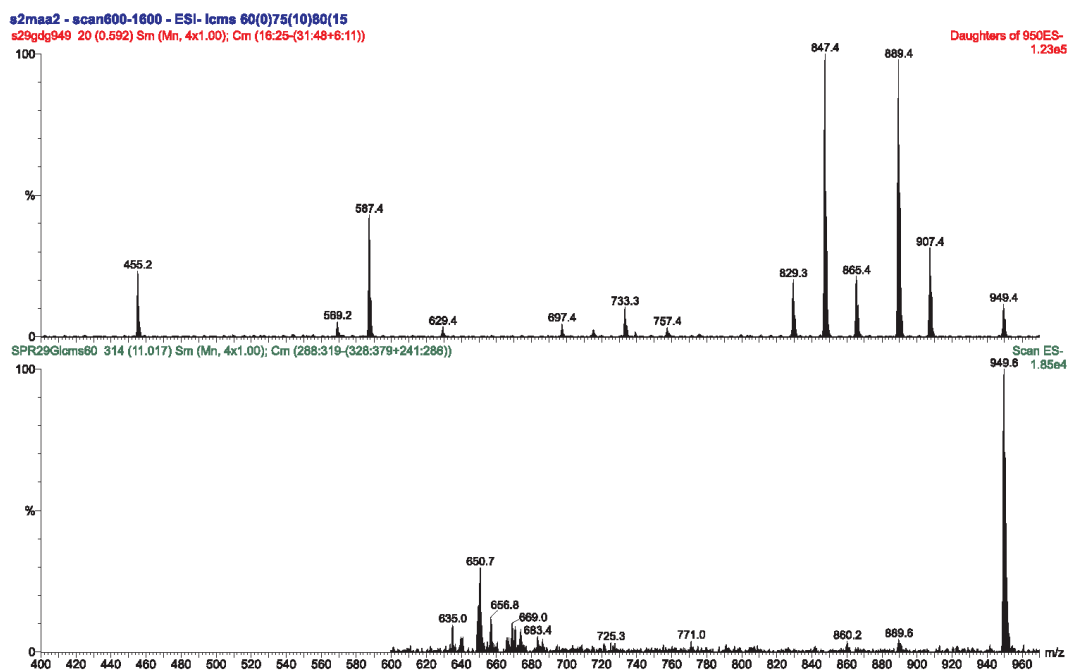
Figure S32. ESI-MS and ESI-MS/MS of SAP Olean-ara-rha-xyl w/ 2 OAc.
