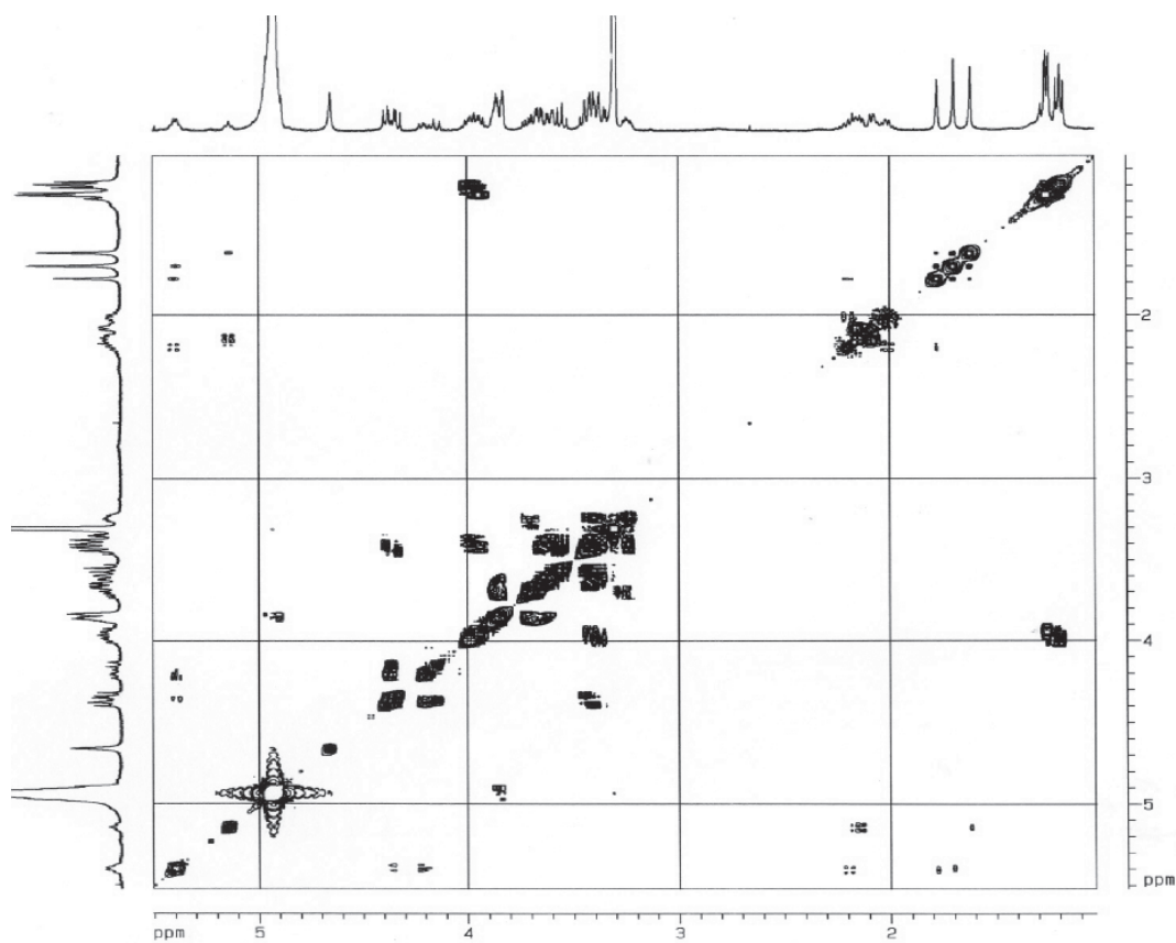
Figure S20. 1 H- 1 H COSY NMR experiment (400 MHz, CD 3 OD) of OGSA o1.
