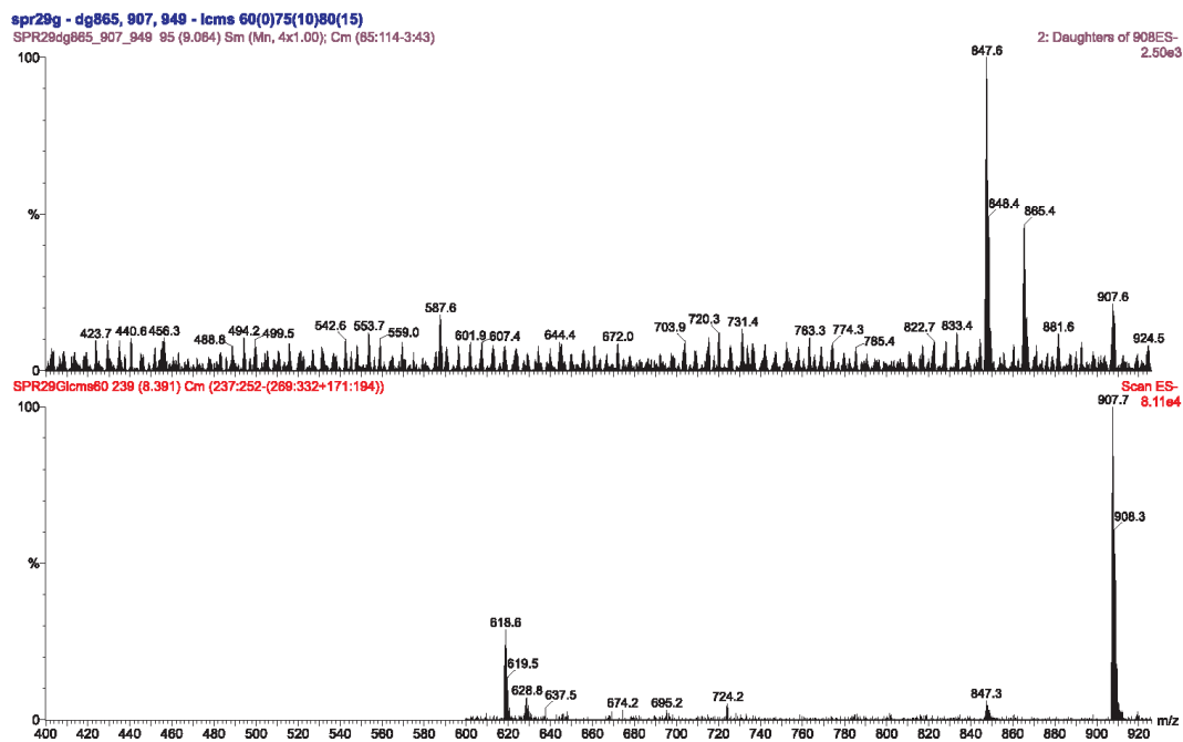
Figure S31. ESI-MS and ESI-MS/MS of SAP Olean-ara-rha-xyl w/ 1 OAc.
