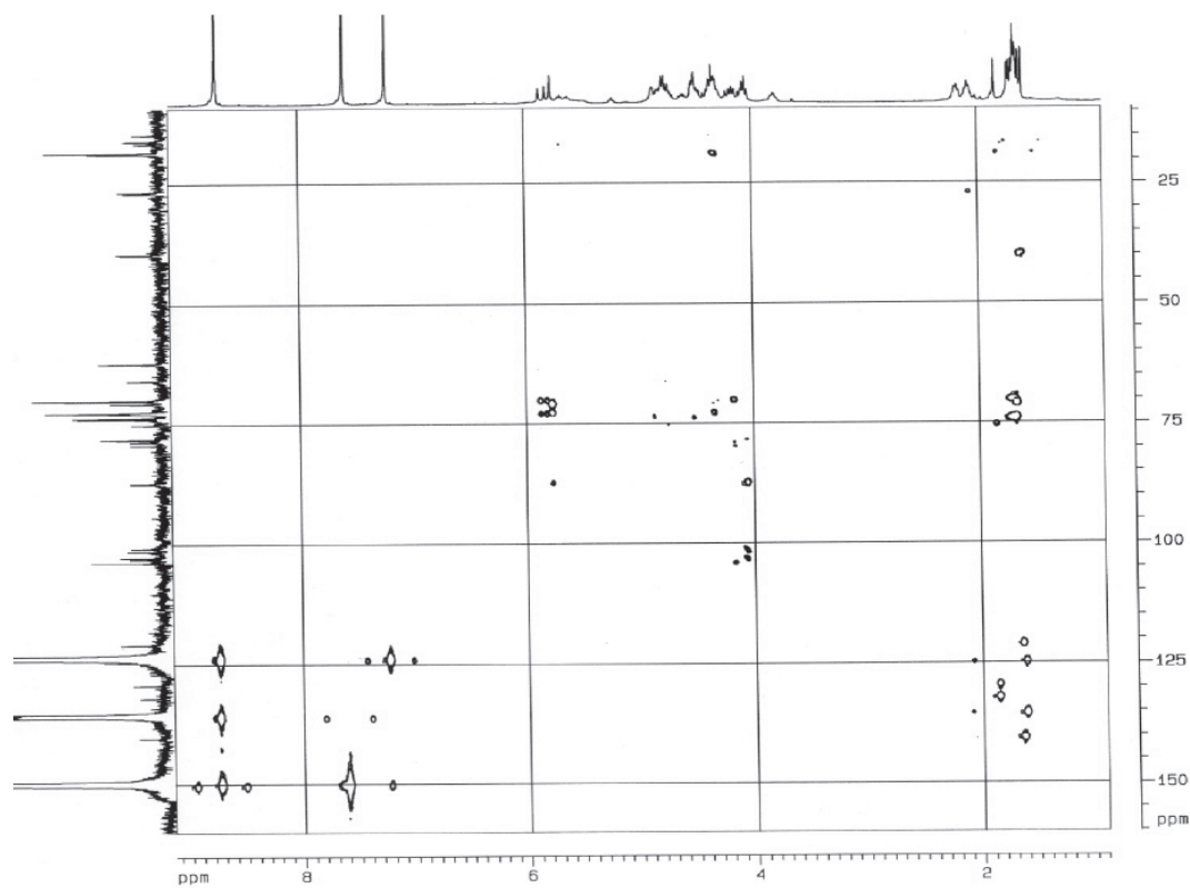
Figure S23. HMBC NMR experiment (400 MHz, C_5D_3N ) of OGSA o1.
