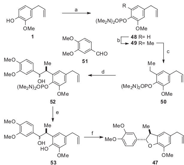
Scheme 7. Reagents and conditions: (a) 1. \text{NaH} , THF; 2. \text{ClPO}(\text{NMe}_2)_2 (97%); (b) 1. ^t\text{BuLi} ; 2. \text{MeI} (96%); (c) 1. ^s\text{BuLi} ; 2. \text{MeI} (96%); (d) ^t\text{BuLi} , tetramethylethylenediamine (TMEDA), 3,4-( \text{MeO} ) _2\text{C}_6\text{H}_3\text{CHO} , -108^\circ\text{C} (71%); (e) \text{LiAlH}_4 (51%); (f) \text{AcOH} (41%).
