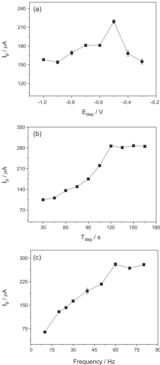
Figure 4. Optimization of the analytical SWASV parameters for \text{Cu}^{2+} ion ( 150 \text{ nmol L}^{-1} ) determination: (a) E_{\text{dep}} using a t_{\text{dep}} = 105 \text{ s} , A_p = 0.025 \text{ V} and f = 60 \text{ Hz} , and (b) t_{\text{dep}} using an E_{\text{dep}} = -0.5 \text{ V} ; and (c) frequency with E_{\text{dep}} = -0.5 \text{ V} , t_{\text{dep}} = 120 \text{ s} .
