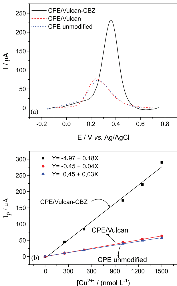
Figure 1. (a) Electrode response: CPE/Vulcan-CBZ (black solid voltammogram); CPE/Vulcan (red dashed voltammogram) and unmodified CPE (blue dotted voltammogram) to 1.0 \mu\text{mol L}^{-1} of \text{Cu}^{2+} ; (b) calibration curves obtained with materials used in (a) (CPE/Vulcan-CBZ, CPE/Vulcan, unmodified CPE) at different concentrations of \text{Cu}^{2+} : 250; 500; 750; 1000; 1250 and 1500 \text{ nmol L}^{-1} . Experiments were performed with the SWASV technique in the following experimental conditions: E_{\text{dep}} = -0.5 \text{ V} , t_{\text{dep}} = 105 \text{ s} , f = 60 \text{ Hz} and A_p = 0.025 \text{ V} .
