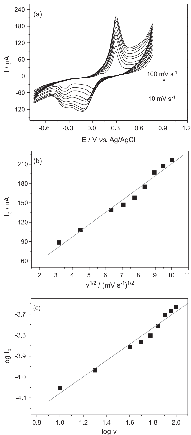
Figure 2. (a) Cyclic voltammograms recorded at scan rates between 10 and 100 \text{ mV s}^{-1} . Relation between (b) anodic peak current ( I_p ) versus v^{1/2} and (c) \log anodic peak current ( I_p ) versus \log v (scan rate). Experiments were carried in 0.1 \text{ mol L}^{-1} (\text{NH}_4)_2\text{SO}_4 , pH 3.5, containing 1 \text{ mmol L}^{-1} \text{ Cu}^{2+} .
