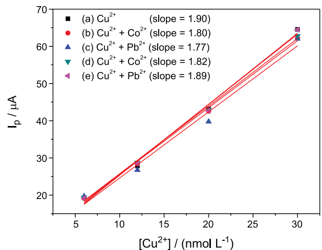
Figure 6. Analytical curves for copper ions in absence (a) and presence of possible interferents (b, c, d, and e). Experiments conducted in 0.2 \text{ mol L}^{-1} of (\text{NH}_4)_2\text{SO}_4 solution, pH 3.5. [\text{foreign specie}] = 0.1 \mu\text{mol L}^{-1} . E_{\text{dep}} = -0.5 \text{ V} ; t_{\text{dep}} = 120 \text{ s} ; f = 60 \text{ Hz} ; A_p = 0.025 \text{ V} and t_{\text{eq}} = 15 \text{ s} ; potential range: -0.2 to 1.0 \text{ V vs. Ag/AgCl} .
