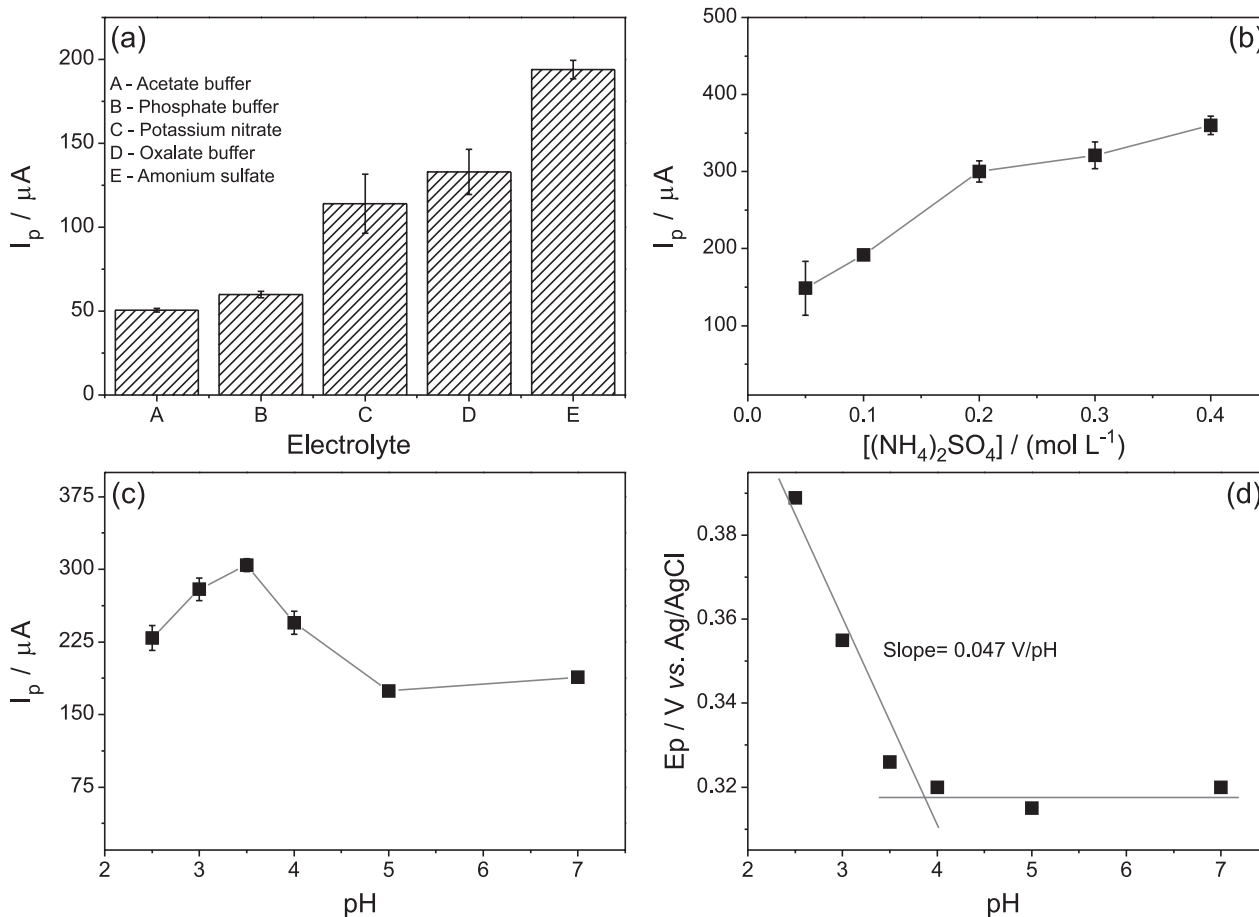
Figure 3. Effect of the: (a) nature of the supporting electrolyte (0.1 mol L -1 , pH 3.5); (b) supporting electrolyte concentration (0.05, 0.1, 0.2, 0.3 and 0.4 mol L -1 (pH 3.5); (c) and (d) pH of the electrolytic solution on the voltammetric Cu 2+ response. Experimental conditions: [Cu 2+ ] = 1.0 \mu\text{mol L}^{-1} . E_{\text{dep}} = -0.5 \text{ V} ; t_{\text{dep}} = 105 \text{ s} , A_p = 0.025 \text{ V} and f = 60 \text{ Hz} .
