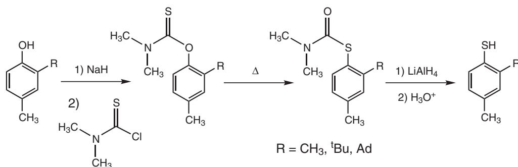
Scheme 1. Synthesis of 2,4-disubstituted thiophenols.
