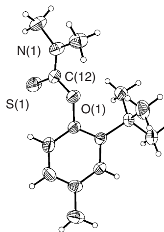
Figure 2. ORTEP view of 5 .
