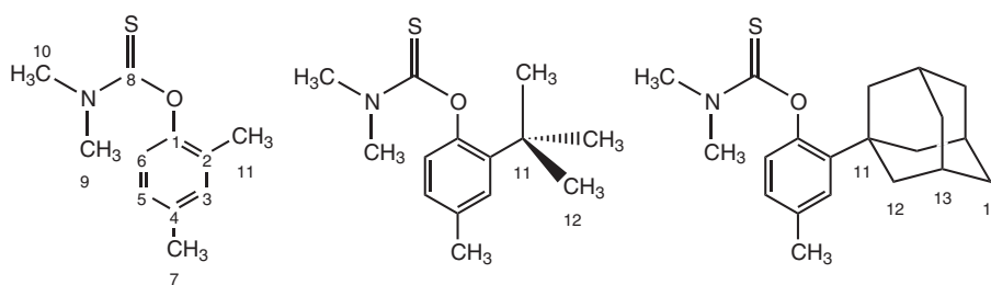
Scheme 2. Numbering scheme employed in NMR assignments.
