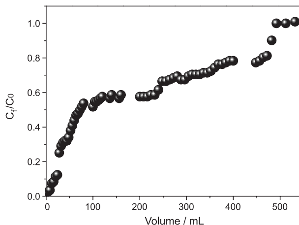
Figure 7. Breakthrough curve of 3-mercaptopropyltrimethoxysilane (3-MPTMS)-grafted carbon black (CB) using 0.3 mg L -1 cadmium at a flow rate 4.0 mL min -1 . C e : Cadmium concentration in the column effluent; C 0 : initial cadmium concentration, 0.3 mg L -1 .
