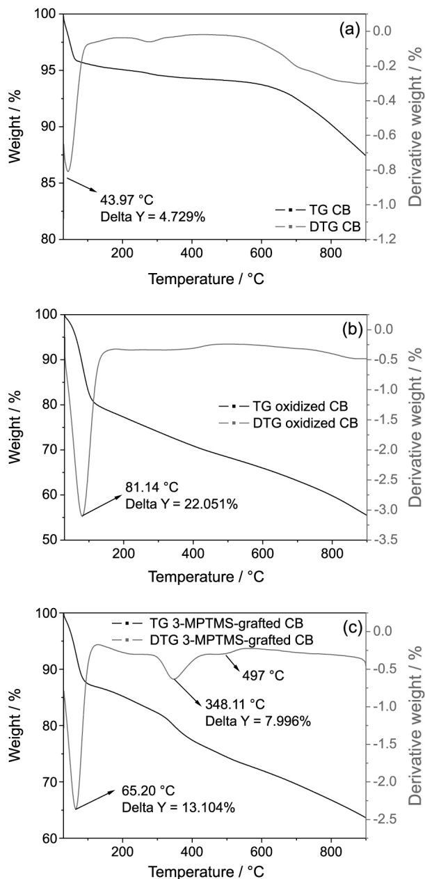
Figure 5. Thermogravimetric curve (TG) and derivative thermogravimetric curve (DTG) from (a) carbon black (CB); (b) oxidized CB; and (c) 3-mercaptopropyltrimethoxysilane (3-MPTMS)-grafted CB.
