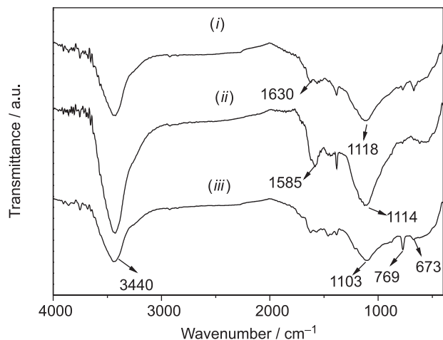
Figure 3. Fourier transform infrared (FTIR) spectrum of (i) carbon black (CB); (ii) oxidized CB; and (iii) 3-mercaptopropyltrimethoxysilane (3-MPTMS)-grafted CB.
