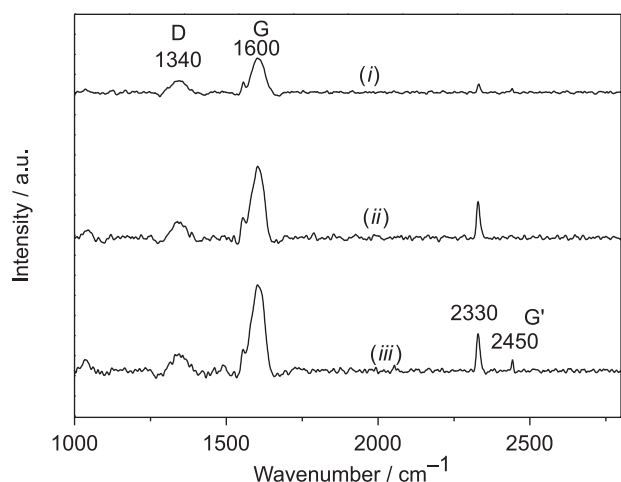
Figure 4. Raman spectra of (i) carbon black (CB); (ii) oxidized CB; and (iii) 3-mercaptopropyltrimethoxysilane (3-MPTMS)-grafted CB. D, G and G' is defect or disorder and graphite bands, respectively.
