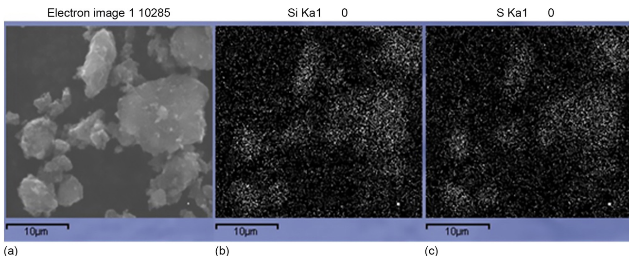
Figure 2. Scanning electron microscope (SEM) image for (a) 3-mercaptopropyltrimethoxysilane (3-MPTMS)-grafted carbon black (CB); and respective elemental mapping for (b) Si and (c) S.
