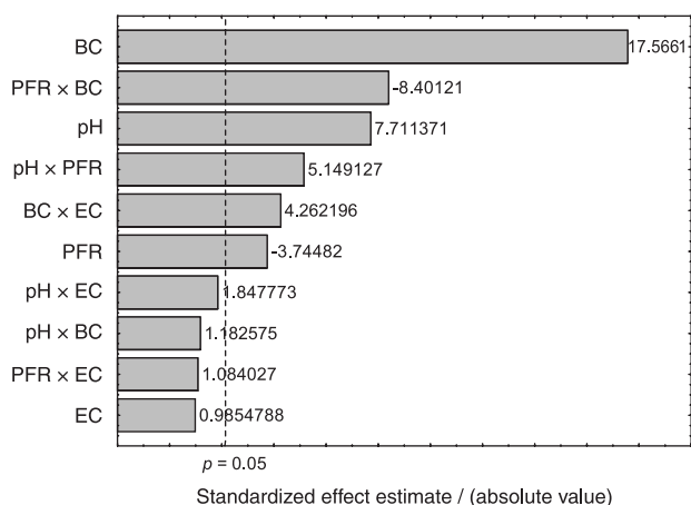
Figure 6. Pareto chart obtained from 2 4 full factorial design. BC: Buffer concentration; PFR: preconcentration flow rate; and EC: eluent concentration.
