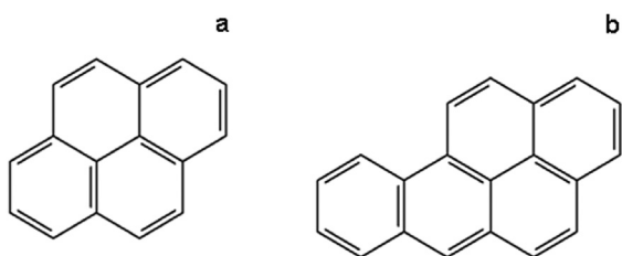
Figure 1. Molecular structure of pyrene (a) and benzo[a]pyrene (b).
