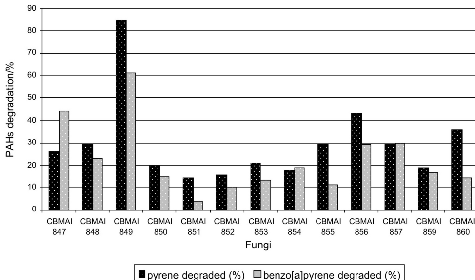
Figure 4. Degradation rate (%) of pyrene and benzo[a]pyrene from thirteen filamentous fungi (see identification in Table 1) isolated from marine cnidarians with the ability to decolorize/tolerate the dye Remazol Brilliant Blue R (RBBR). CBMAI: Brazilian Collection of Environmental and Industrial Microorganisms.
