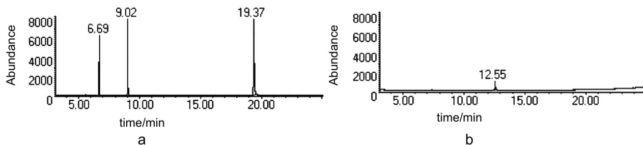
Figure 2. Typical chromatograms obtained in SIM mode for: (a) standard solution containing 4.13 \mu\text{g mL}^{-1} of dibutyl phthalate (RT = 6.69 min), 4.56 \mu\text{g mL}^{-1} of pyrene (RT = 9.02 min), 8.48 \mu\text{g mL}^{-1} of benzo[a]pyrene (RT = 19.37 min); (b) blank sample.
