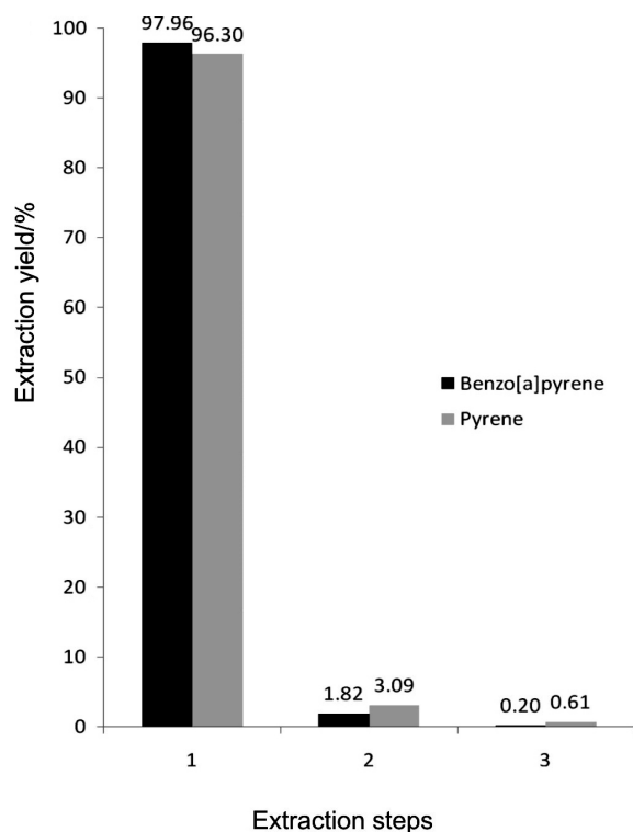
Figure 3. Percentage of PAHs recovered after three extraction procedures.
