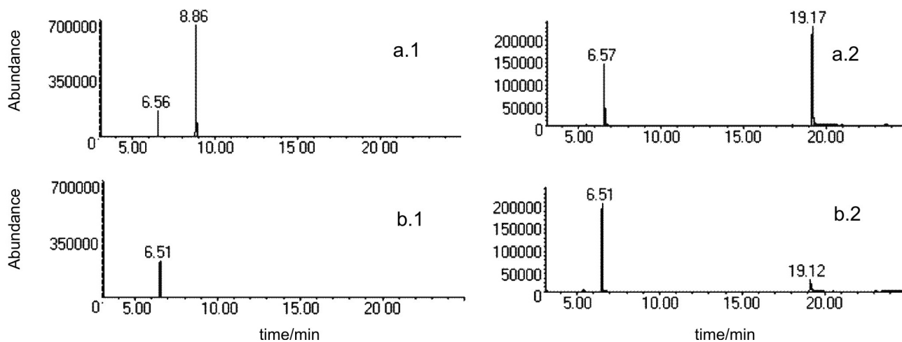
Figure 5. Chromatograms obtained by GC-MS (SIM) of fermentative medium of the fungus Penicillium sp. CBMAI 851 (a) and A. sclerotiorum CBMAI 849 (b) showing the different levels of pyrene and benzo[a]pyrene degradation. (a.1) 14% of pyrene degradation; (a.2) 4.0% of benzo[a]pyrene degradation; (b.1) 85% of pyrene degradation; and (b.2) 61% of benzo[a]pyrene degradation. IS: internal standard.
