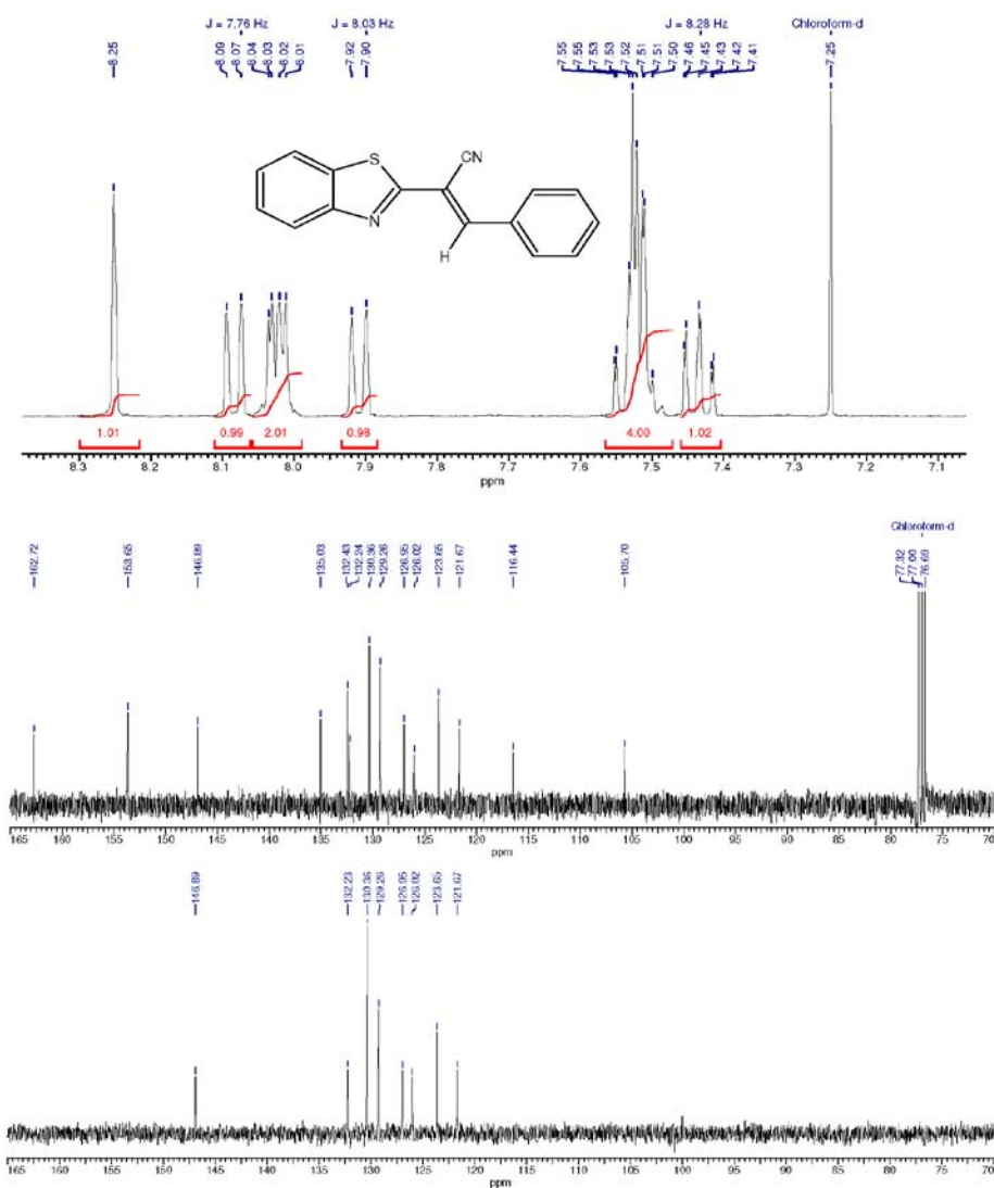
Figure S1. 1 H and 13 C and DEPT-135 NMR spectra for compound 3a.
