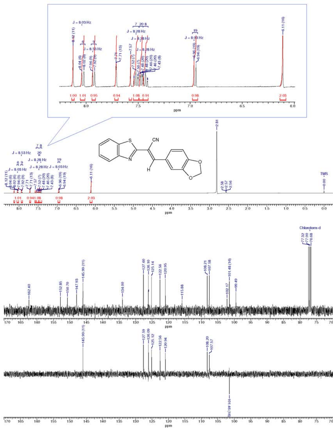
Figure S10. ^1\text{H} , ^{13}\text{C} and DEPT-135 spectra for compound 3j .
