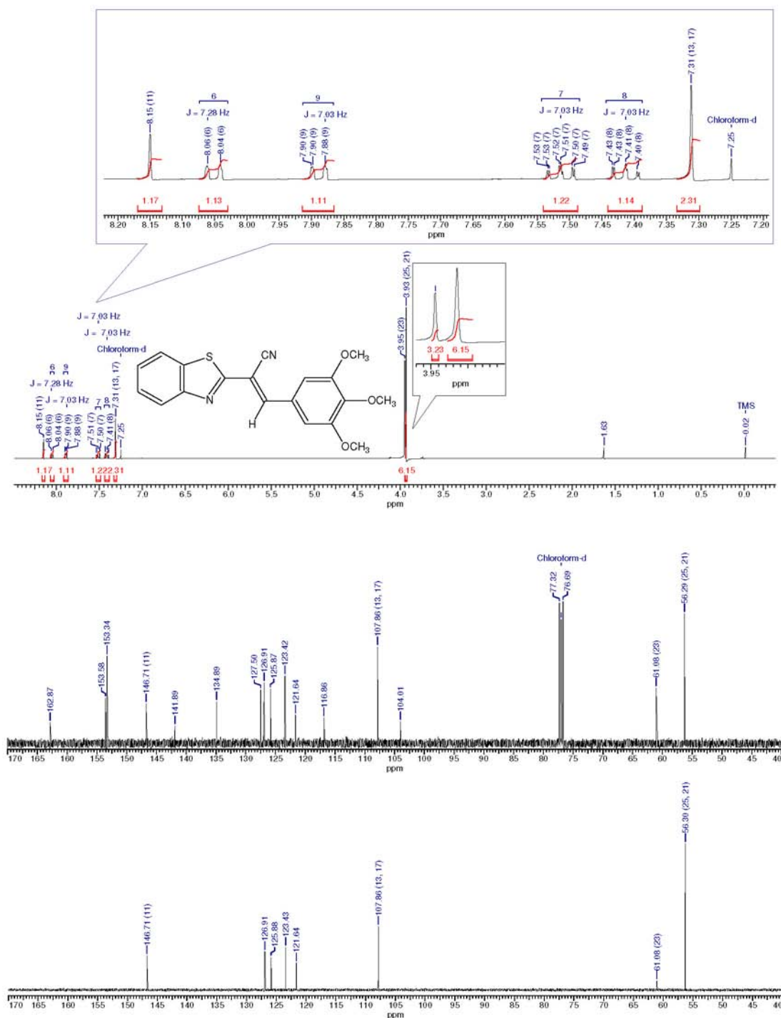
Figure S9. ^1\text{H} , ^{13}\text{C} and DEPT-135 spectra for compound 3i .
