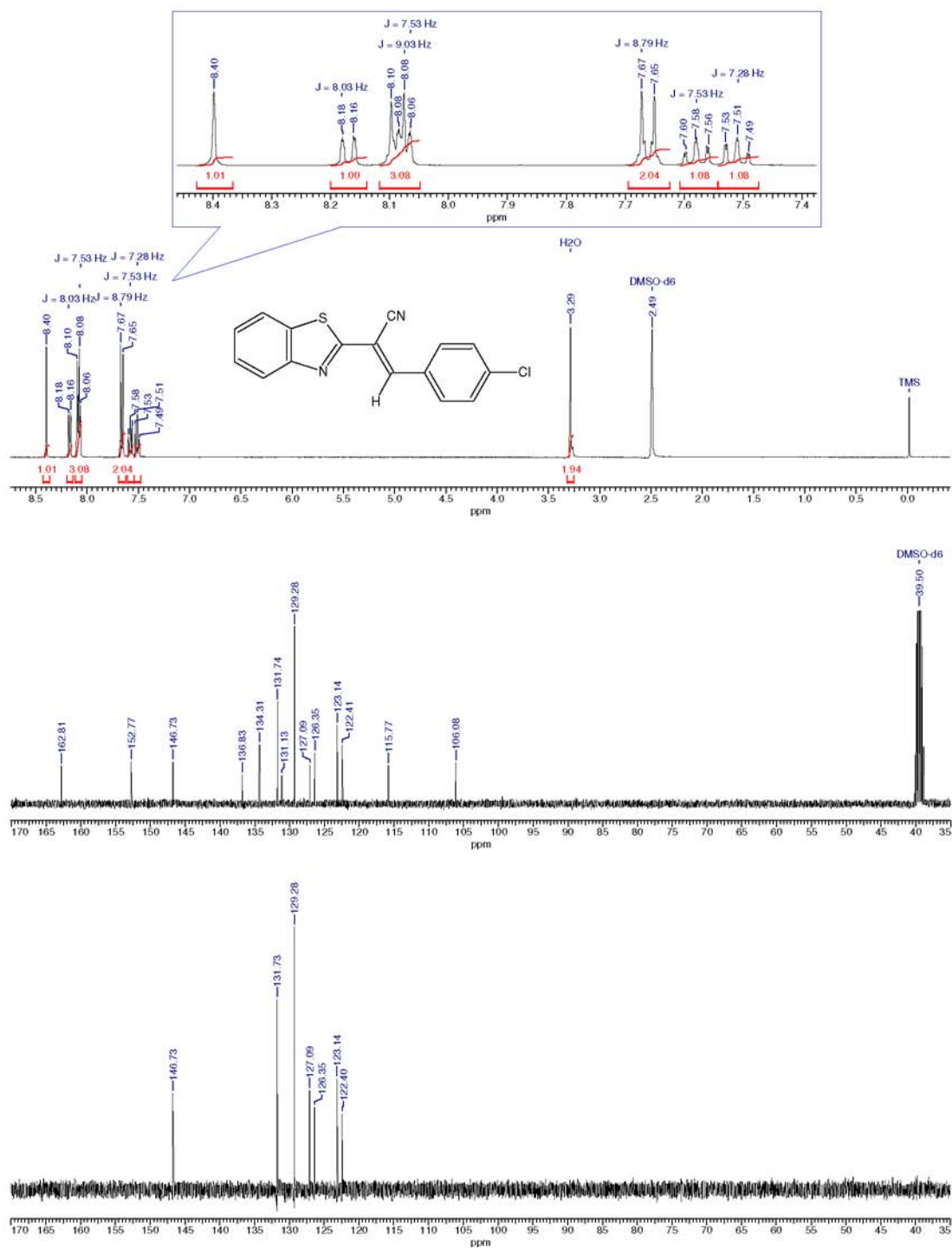
Figure S4. ^1\text{H} , ^{13}\text{C} and DEPT-135 spectra for compound 3d .
