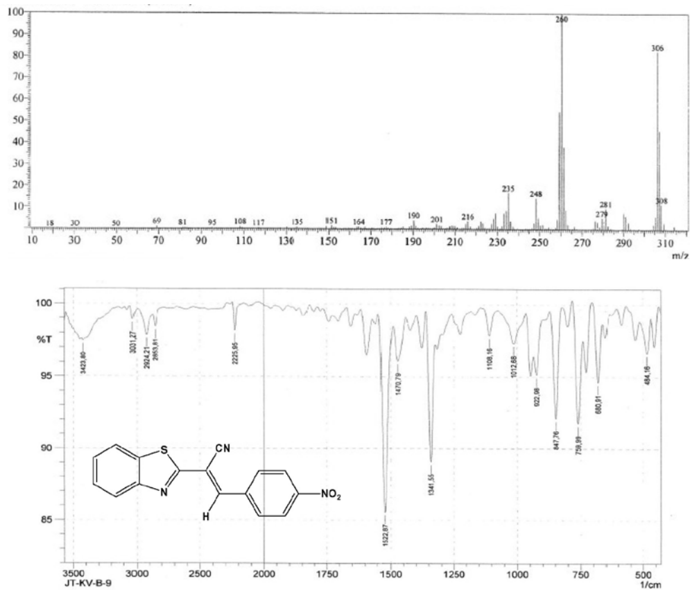
Figure S13. MS and IR spectra for compound 3c.
