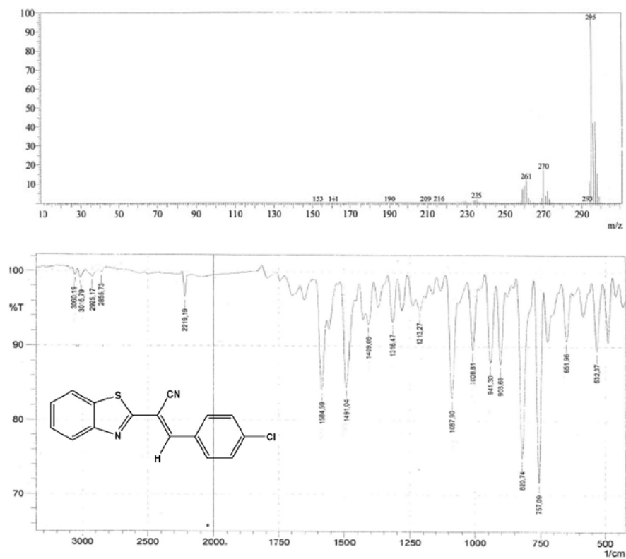
Figure S14. MS and IR spectra for compound 3d.
