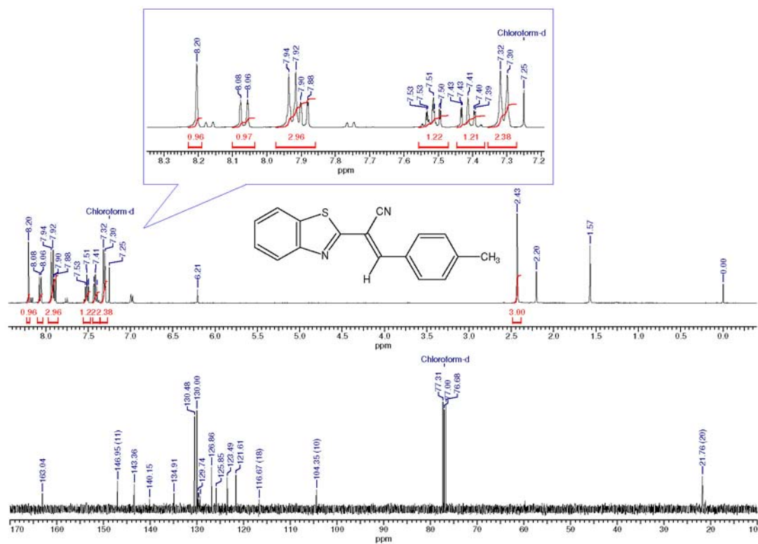
Figure S2. ^1\text{H} and ^{13}\text{C} NMR spectra for compound 3b .
