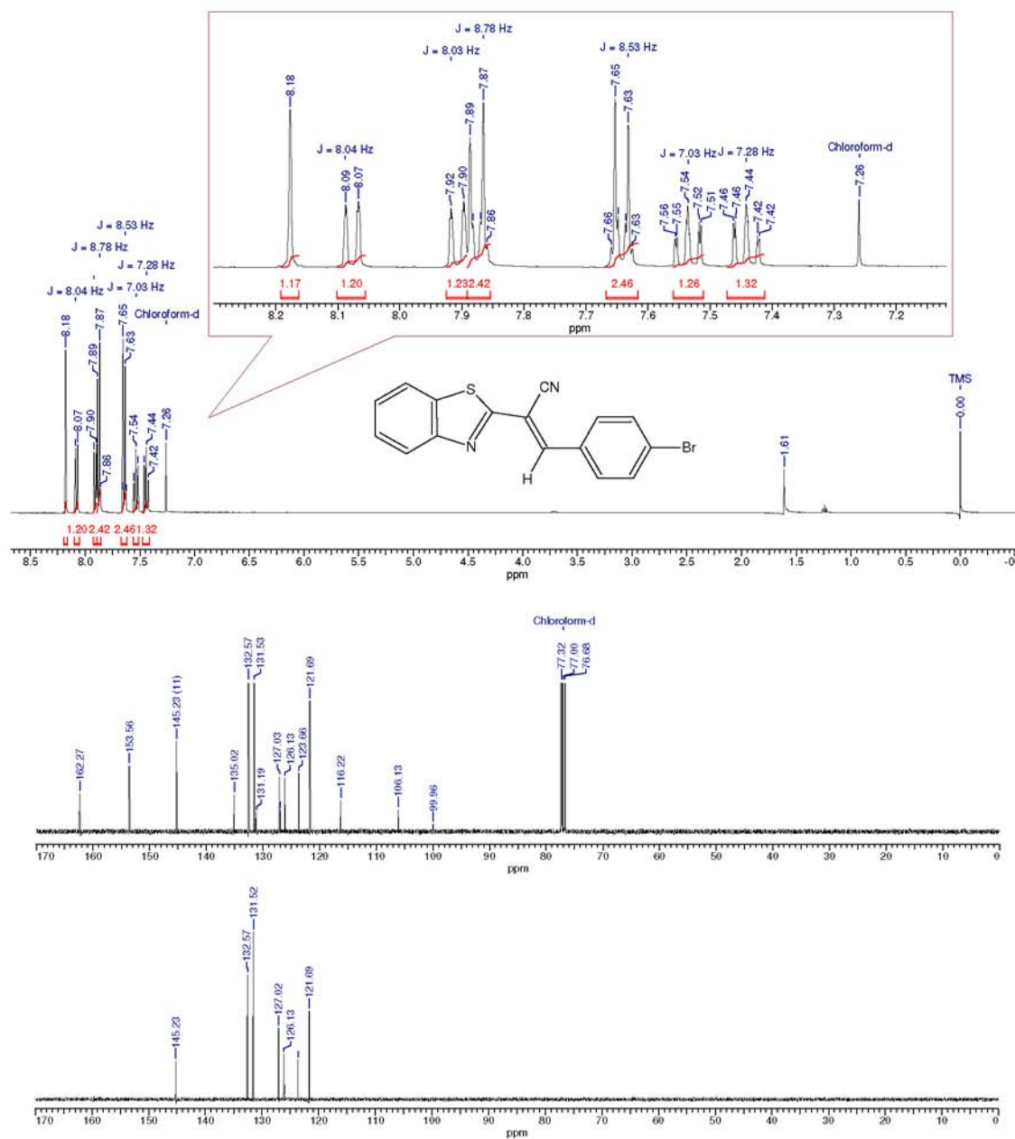
Figure S5. ^1\text{H} , ^{13}\text{C} and DEPT-135 spectra for compound 3e .
