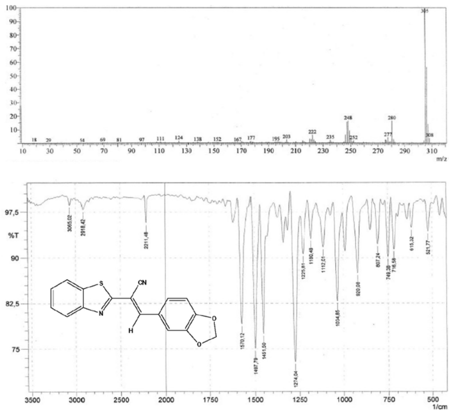
Figure S20. MS and IR spectra for compound 3j.
