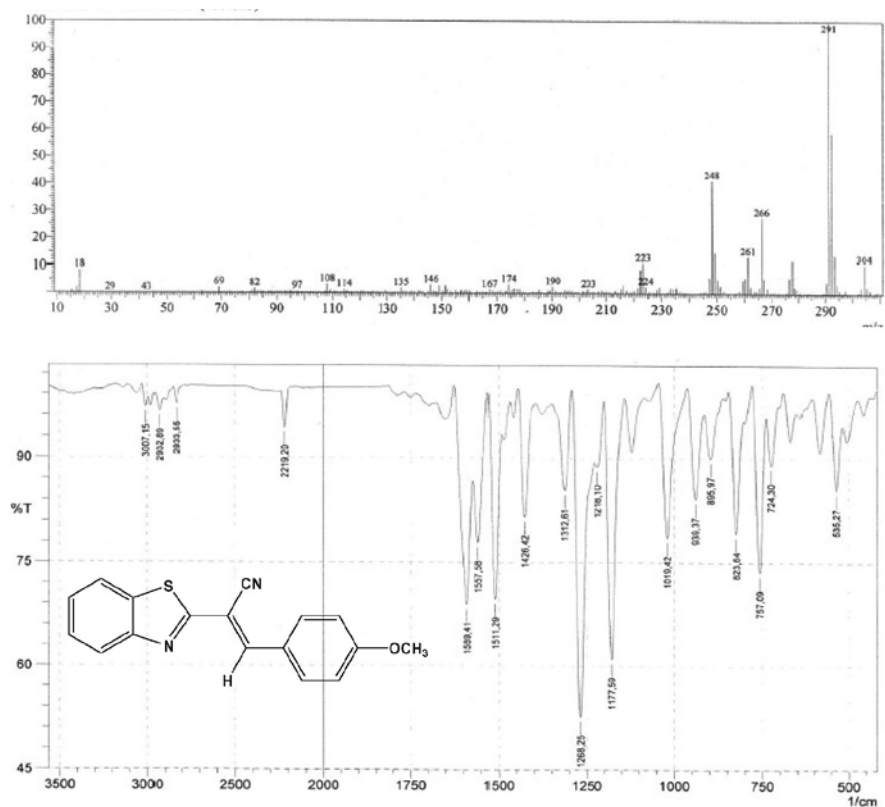
Figure S18. MS and IR spectra for compound 3h .
