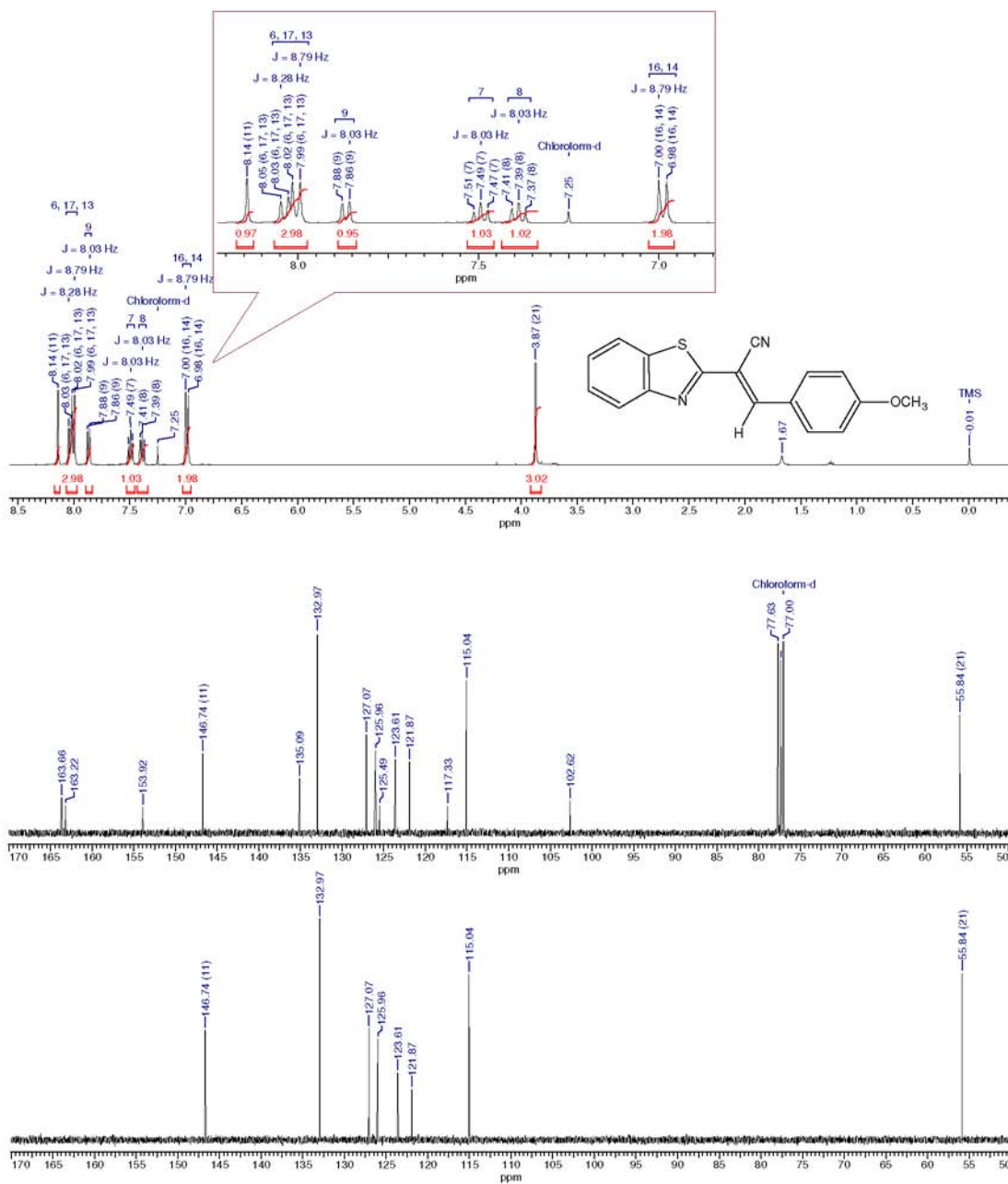
Figure S8. 1 H, 13 C and DEPT-135 spectra for compound 3h .
