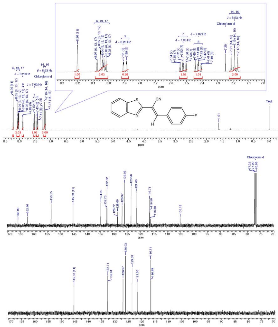
Figure S6. ^1\text{H} , ^{13}\text{C} and DEPT-135 spectra for compound 3f .
