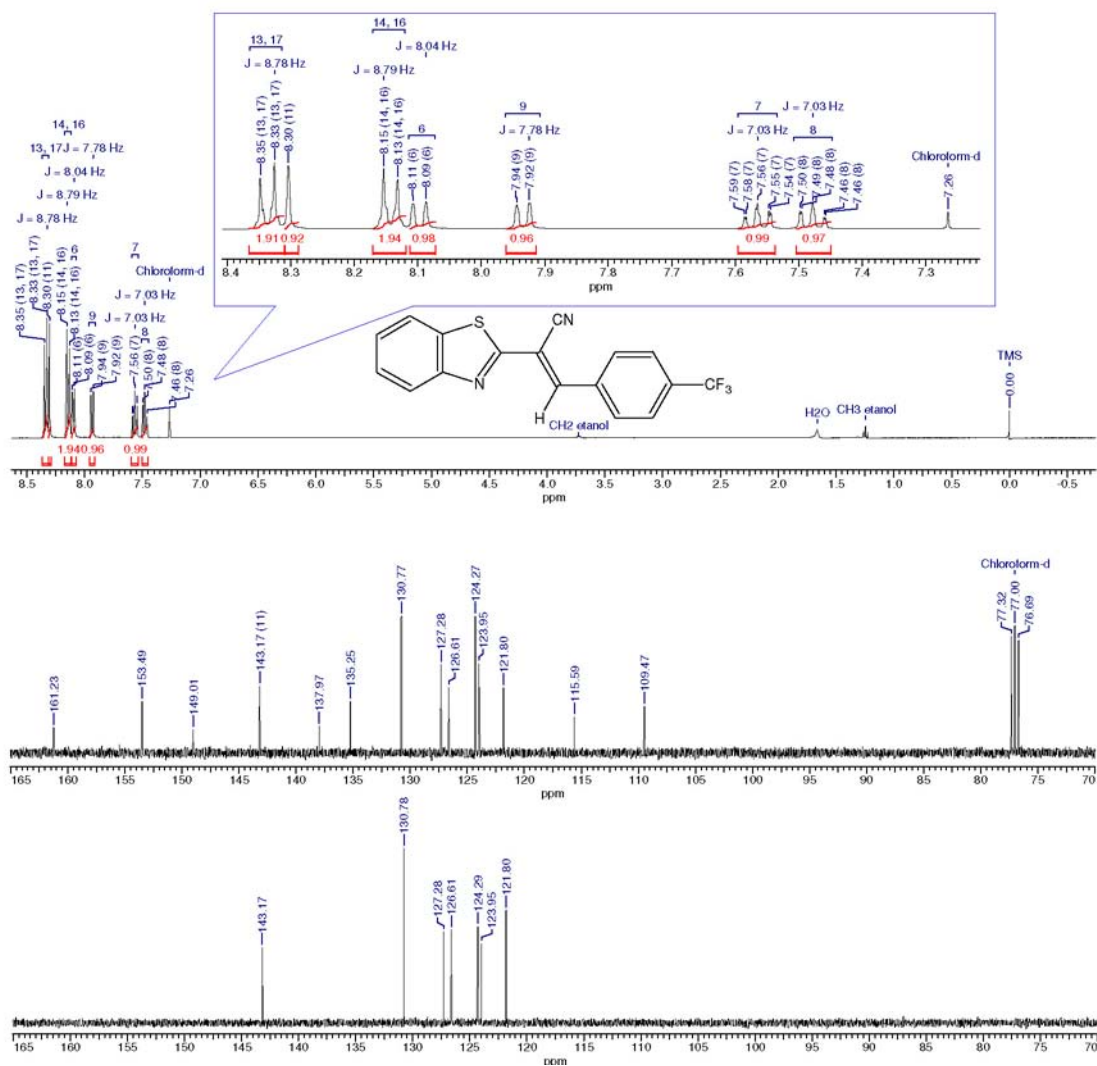
Figure S7. ^1\text{H} , ^{13}\text{C} and DEPT-135 spectra for compound 3g .
