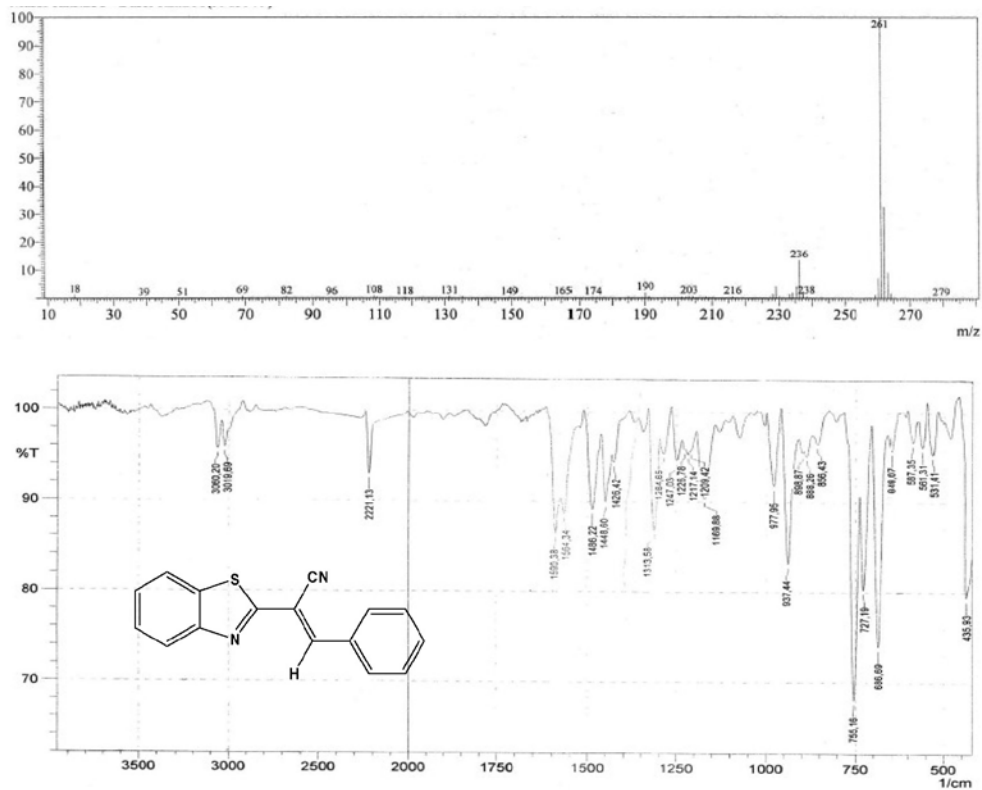
Figure S11. MS and IR spectra for Compound 3a.
