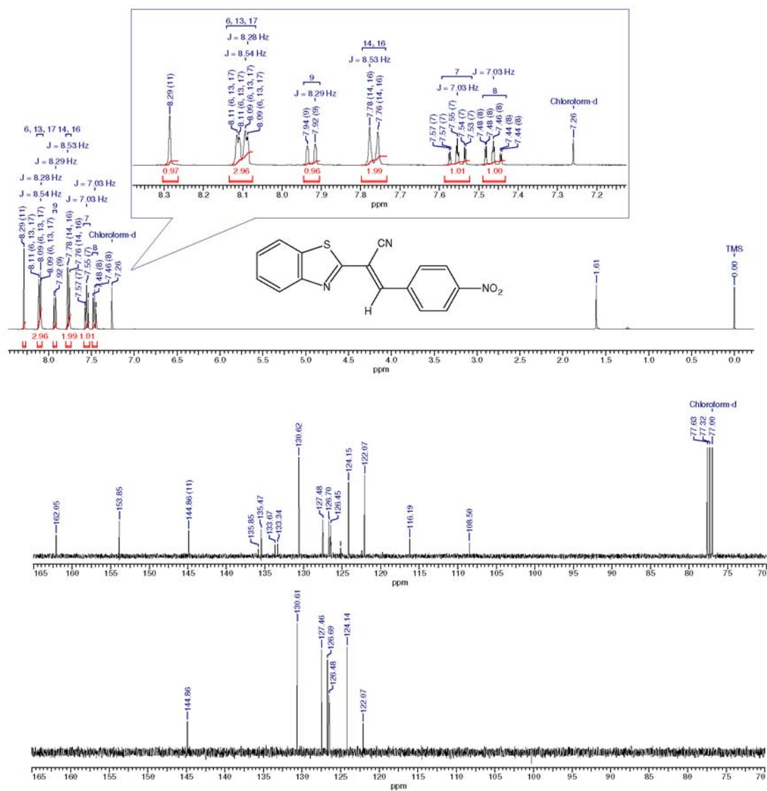
Figure S3. ^1\text{H} , ^{13}\text{C} and DEPT-135 NMR spectra for compound 3c .
