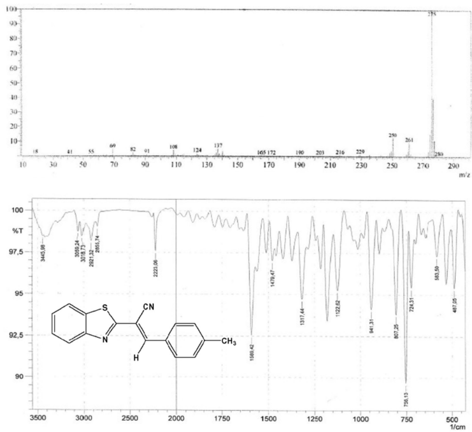
Figure S12. MS and IR spectra for Compound 3b.
