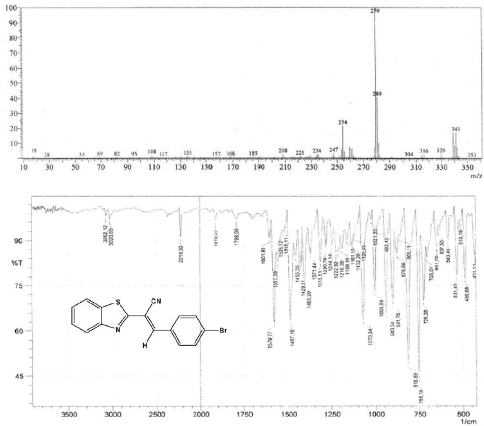
Figure S15. MS and IR spectra for compound 3e.
