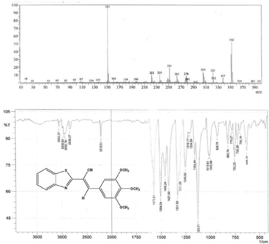
Figure S19. MS and IR spectra for compound 3i.
