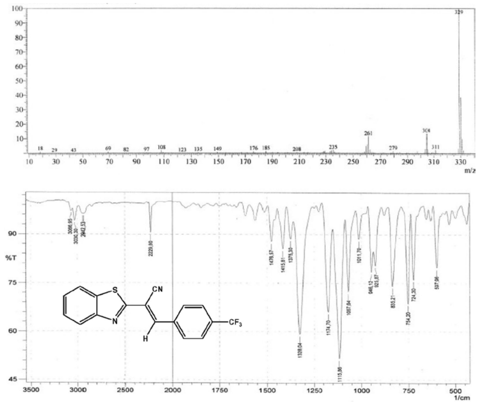
Figure S17. MS and IR spectra for compound 3g .
