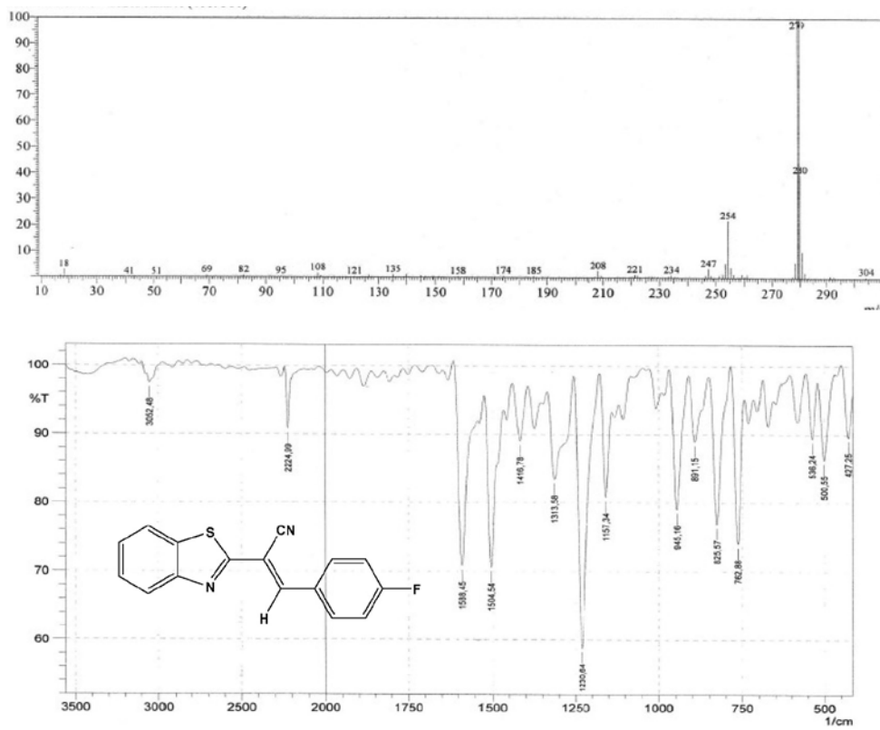
Figure S16. MS and IR spectra for compound 3f.
