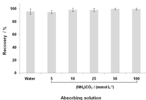
Figure 2. Influence of absorbing solutions for Cl determination in cigarette tobacco samples using H 2 O, (NH 4 ) 2 CO 3 10, 25, 50 or 100 mmol L -1 and reflux step. Determination by ICP OES. (error bars are the standard deviation, n = 3).
