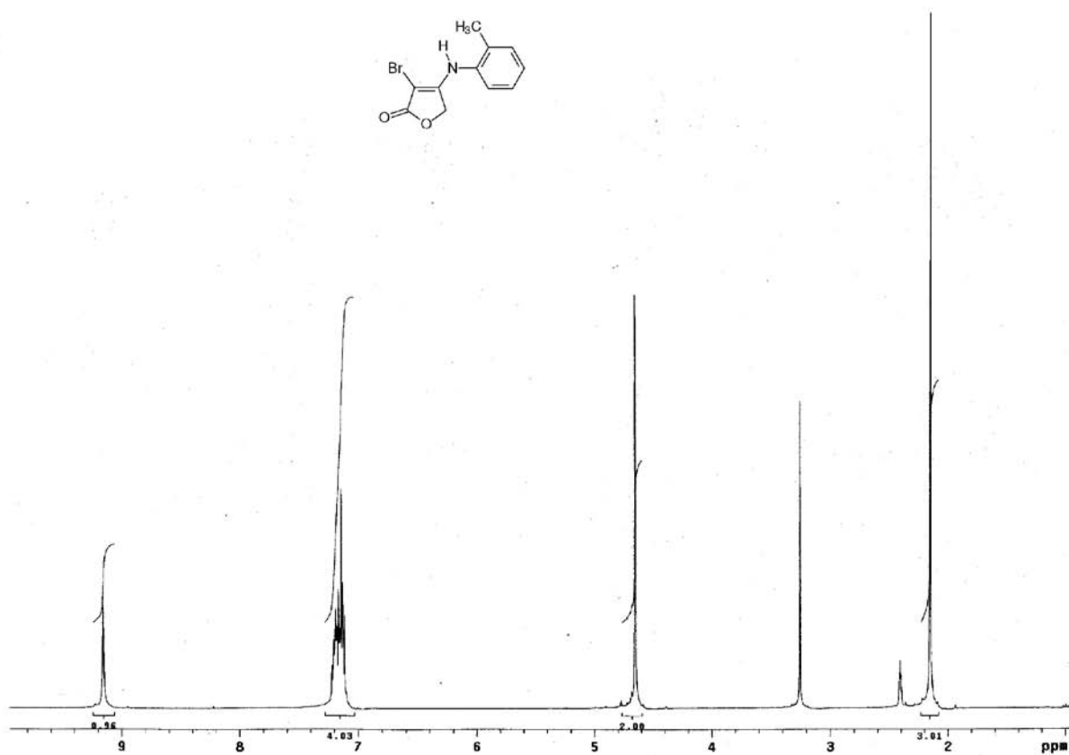
Figure S7. Full 1 H NMR spectrum of compound 3d (DMSO- d 6 ).
