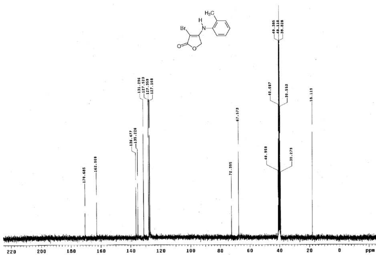
Figure S8. Full 13 C NMR spectrum of compound 3d (DMSO- d 6 ).
