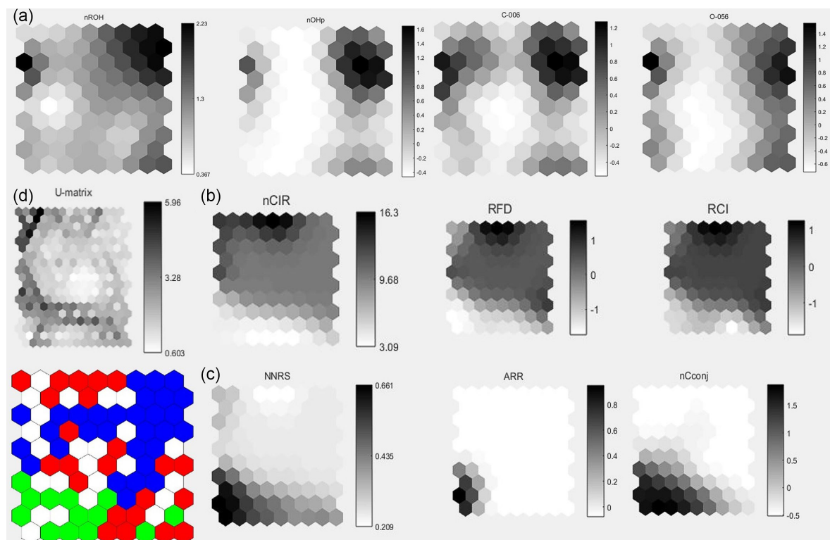
Figure 7. The most significant descriptors for the Annonaceae, Xylopieae and Miliuseae tribes. In (a) we have the U-matrix for the four most significant descriptors in the grouping of the diterpenes of the Annonaceae tribe. In (b), the U-matrix is shown for the three most significant descriptors of the Xylopieae tribe. (c) Shows the U-matrix for the three most significant descriptors of the Miliuseae tribe. Finally, in (d) we have the U-matrix of the self-organizing map generated in the study, with the upper U-matrix not identifying the tribes and the lower U-matrix identifying the tribes by color; Annonaceae is blue, Xylopieae is red, and Miliuseae is green.
