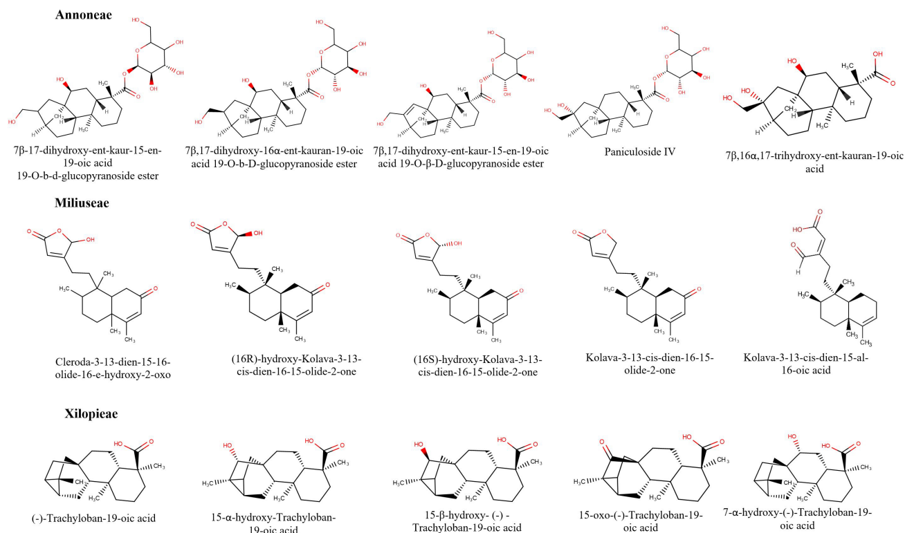
Figure 6. Diterpenes of the most present subtypes in the Annonaceae, Xylopieae, and Miliuseae tribes.
