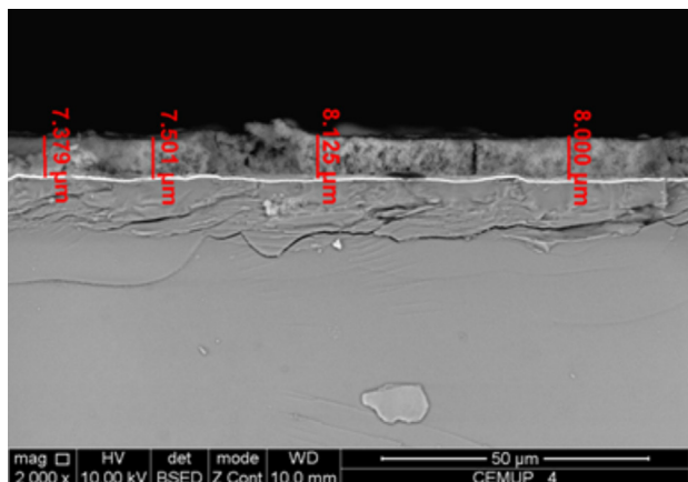
Figure 2. Cross-section field emission scanning electron microscopy (FE-SEM) image of TiO 2 electrode sintered at 450 °C for 30 min.
