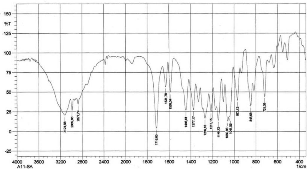
Figure S32. IR spectrum of compound 26.
