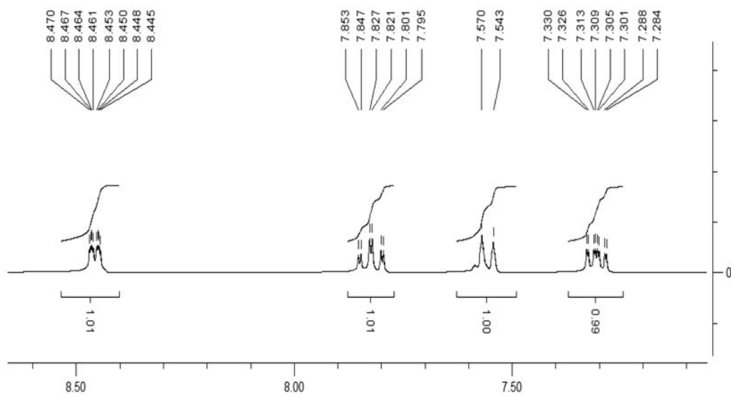
Figure S60. ^1\text{H} NMR spectrum of compound 11 .
