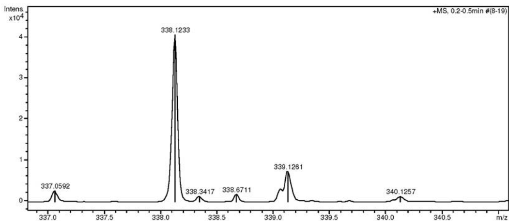
Figure S12. ESI-HRMS spectrum of compound 22 .
