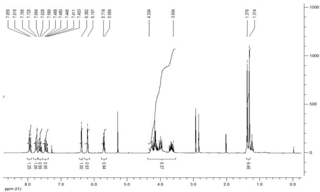
Figure S8. ^1\text{H} NMR spectrum of compound 22.
