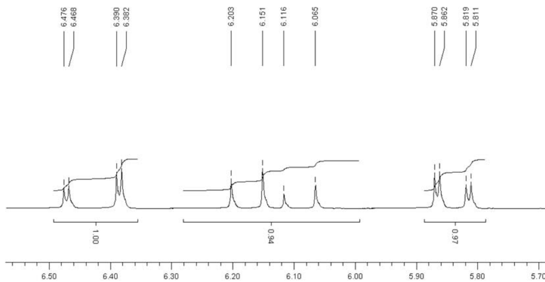
Figure S3. 1 H NMR spectrum of compound 20.
