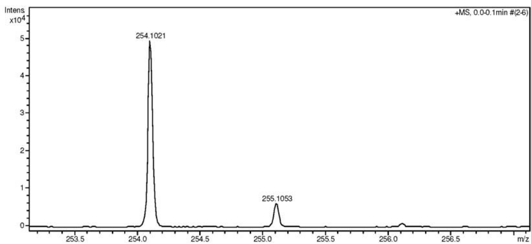
Figure S64. ESI-HRMS spectrum of compound 11.
