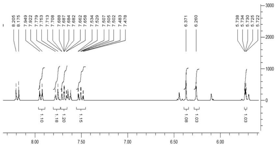
Figure S40. 1 H NMR spectrum of compound 8 .
