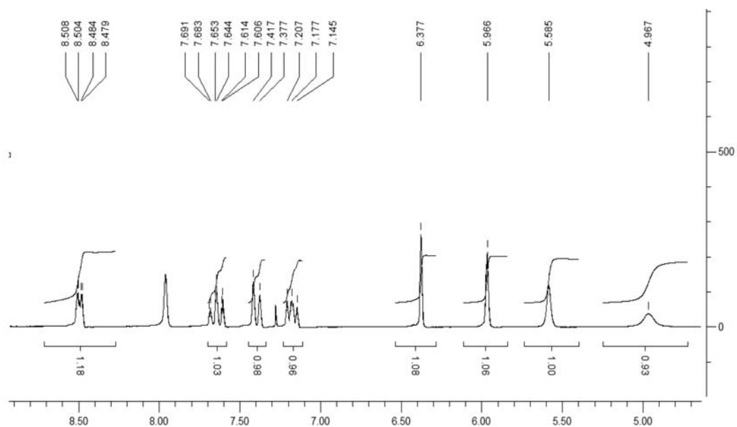
Figure S25. ^1\text{H} NMR spectrum of compound 25.
