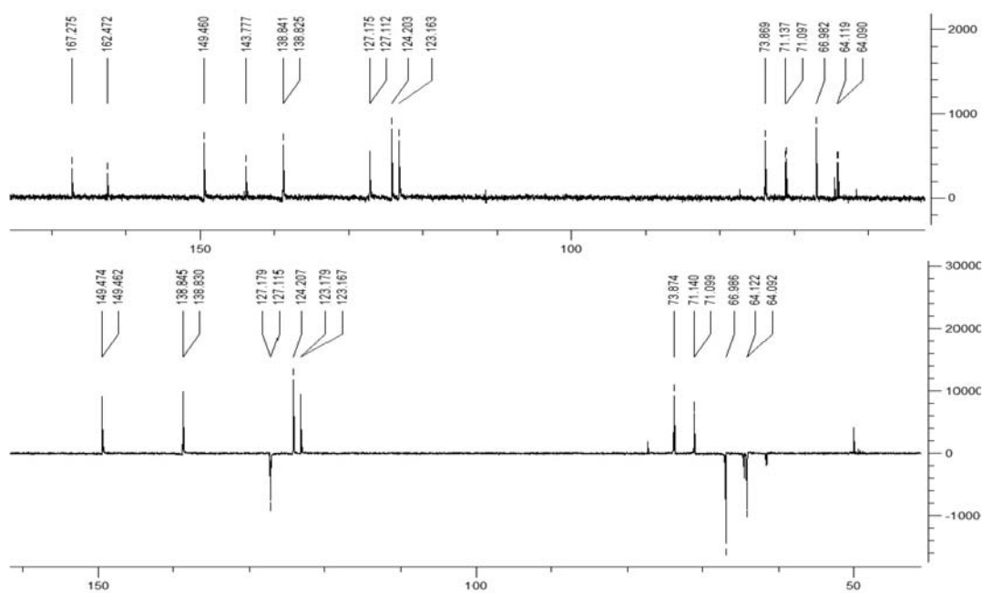
Figure S58. 13 C NMR spectrum of compound 11 .
