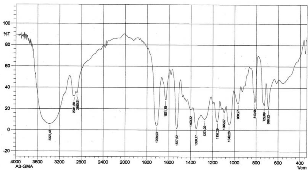
Figure S49. IR spectrum of compound 9 .
