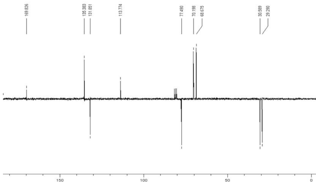
Figure S1. ^{13}C NMR spectrum of compound 20 .
