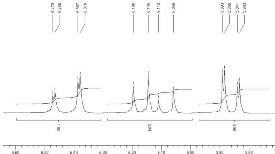
Figure S6. ^1\text{H} NMR spectrum of compound 21 .
