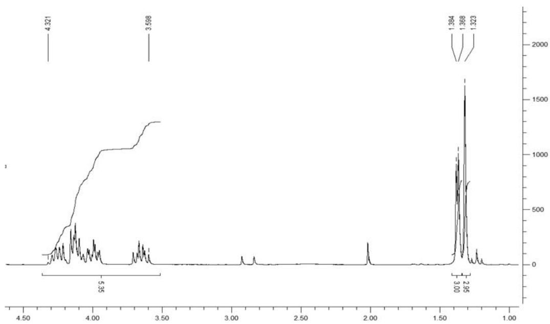
Figure S31. 1 H NMR spectrum of compound 26.
