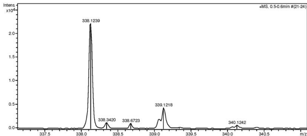
Figure S18. ESI-HRMS spectrum of compound 23.
