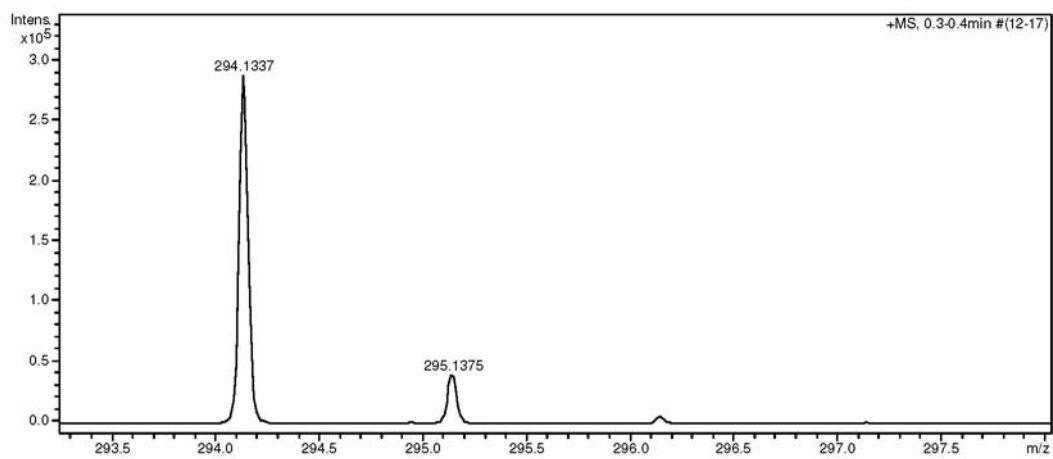
Figure S33. ESI-HRMS spectrum of compound 26.
