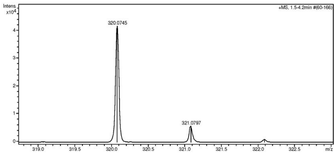
Figure S57. ESI-HRMS spectrum of compound 10.
