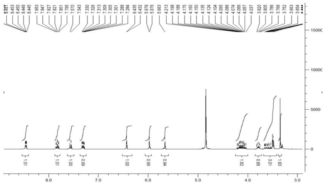
Figure S59. ^1\text{H} NMR spectrum of compound 11 .
