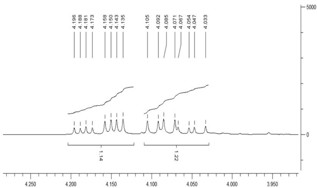
Figure S69. 1 H NMR spectrum of compound 12.
