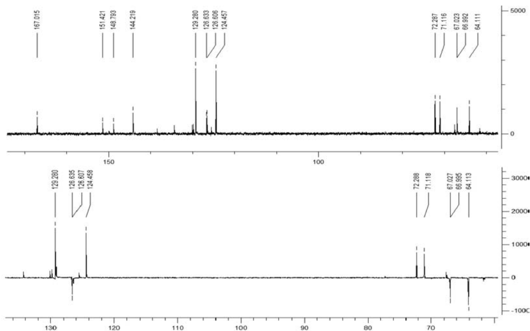
Figure S51. 13 C NMR spectrum of compound 10 .
