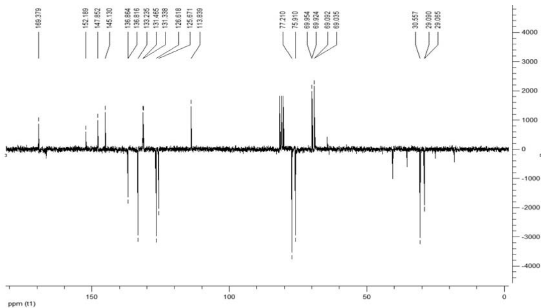
Figure S13. ^{13}C NMR spectrum of compound 23 .
