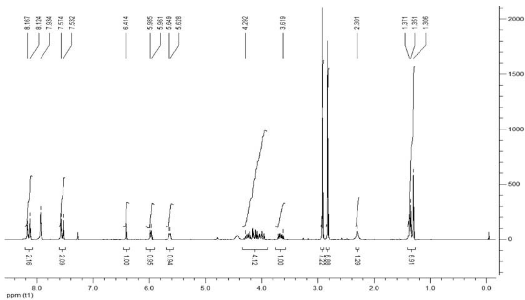
Figure S20. ^1\text{H} NMR spectrum of compound 24.
