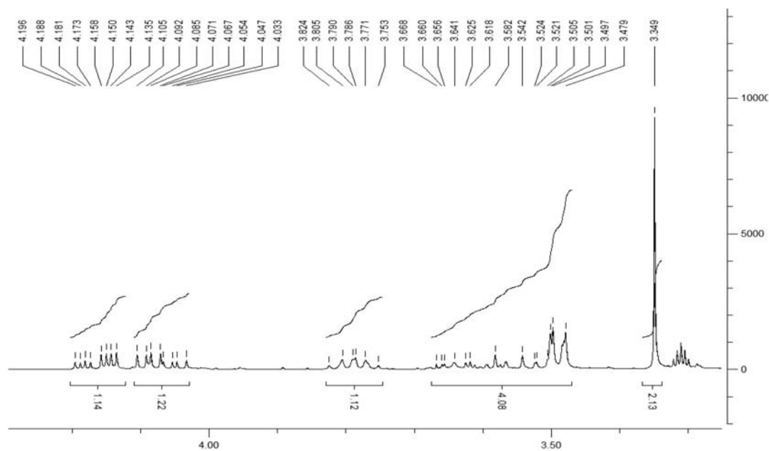
Figure S68. 1 H NMR spectrum of compound 12.
