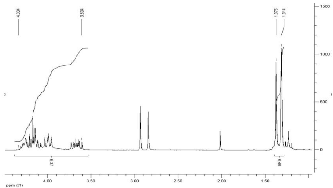
Figure S10. 1 H NMR spectrum of compound 22.
