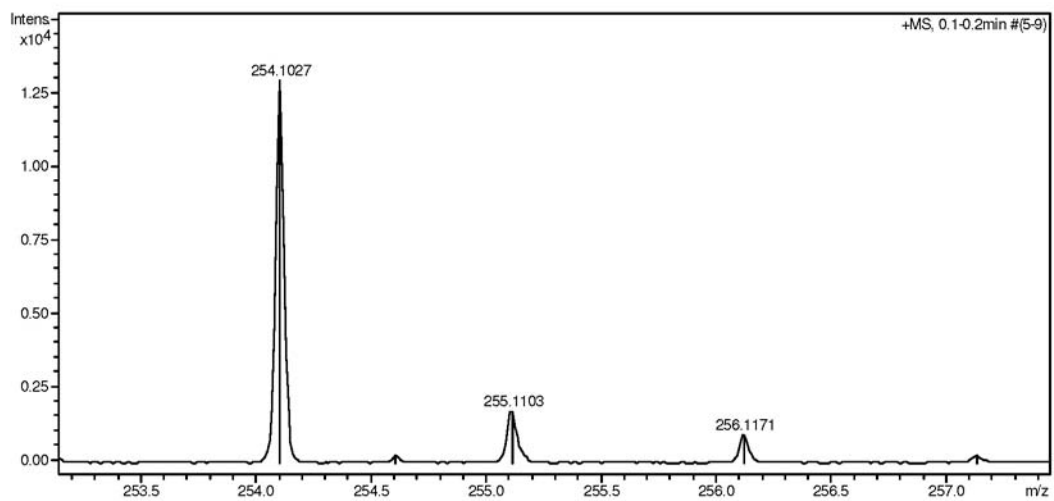
Figure S77. ESI-HRMS spectrum of compound 13 .
