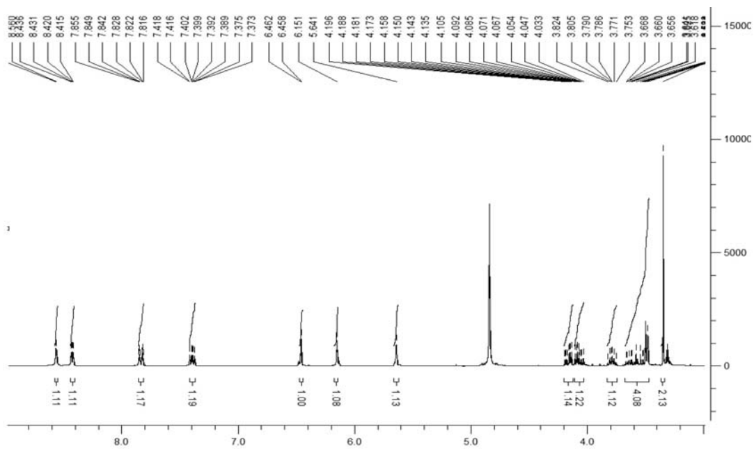
Figure S66. ^1\text{H} NMR spectrum of compound 12.
