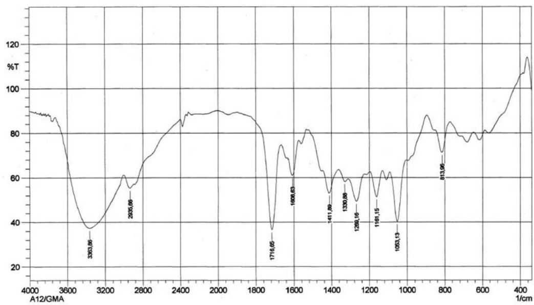
Figure S76. IR spectrum of compound 13.
