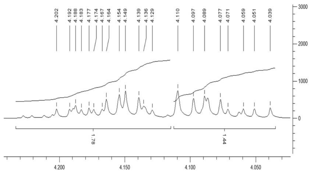
Figure S55. ^1\text{H} NMR spectrum of compound 10.
