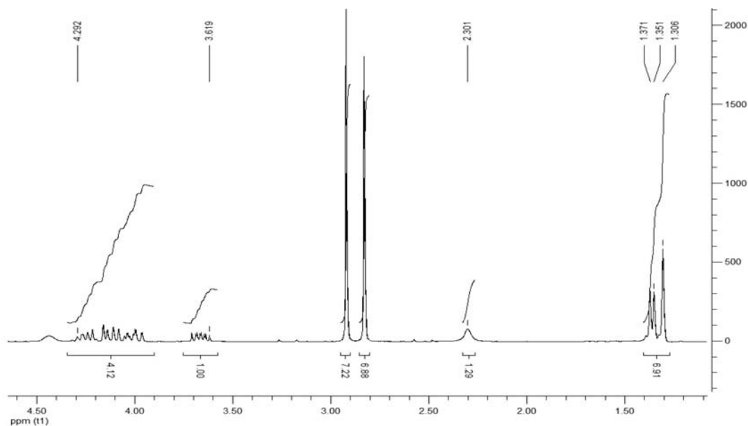
Figure S22. ^1\text{H} NMR spectrum of compound 24 .
