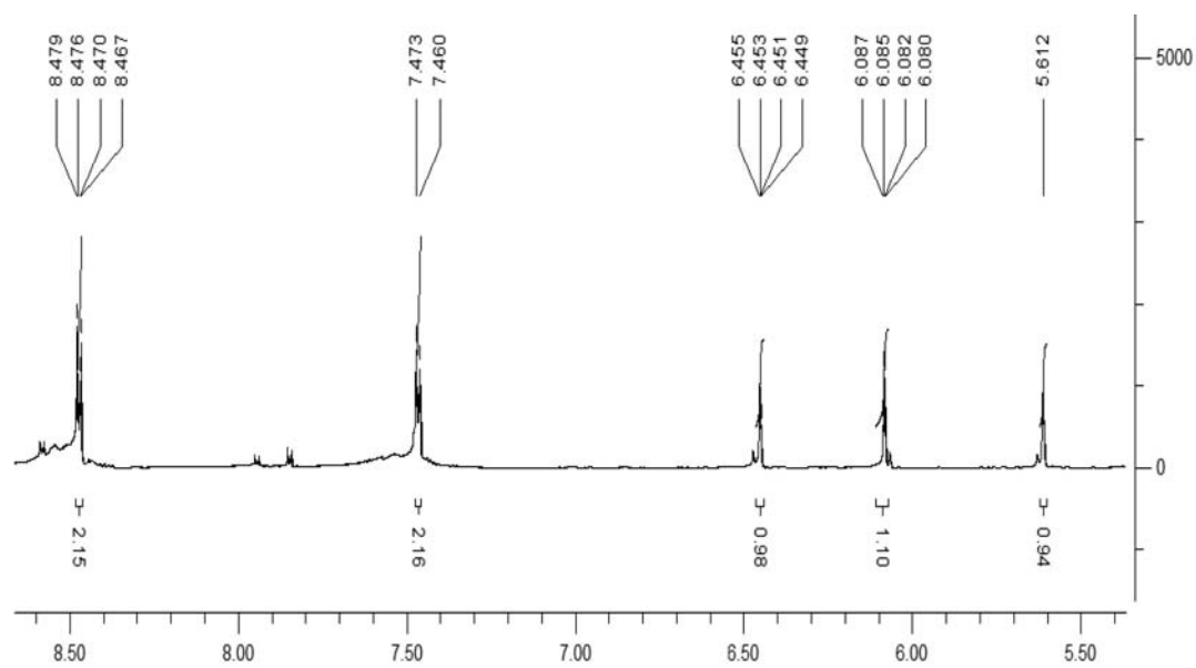
Figure S74. ^1\text{H} NMR spectrum of compound 13.
