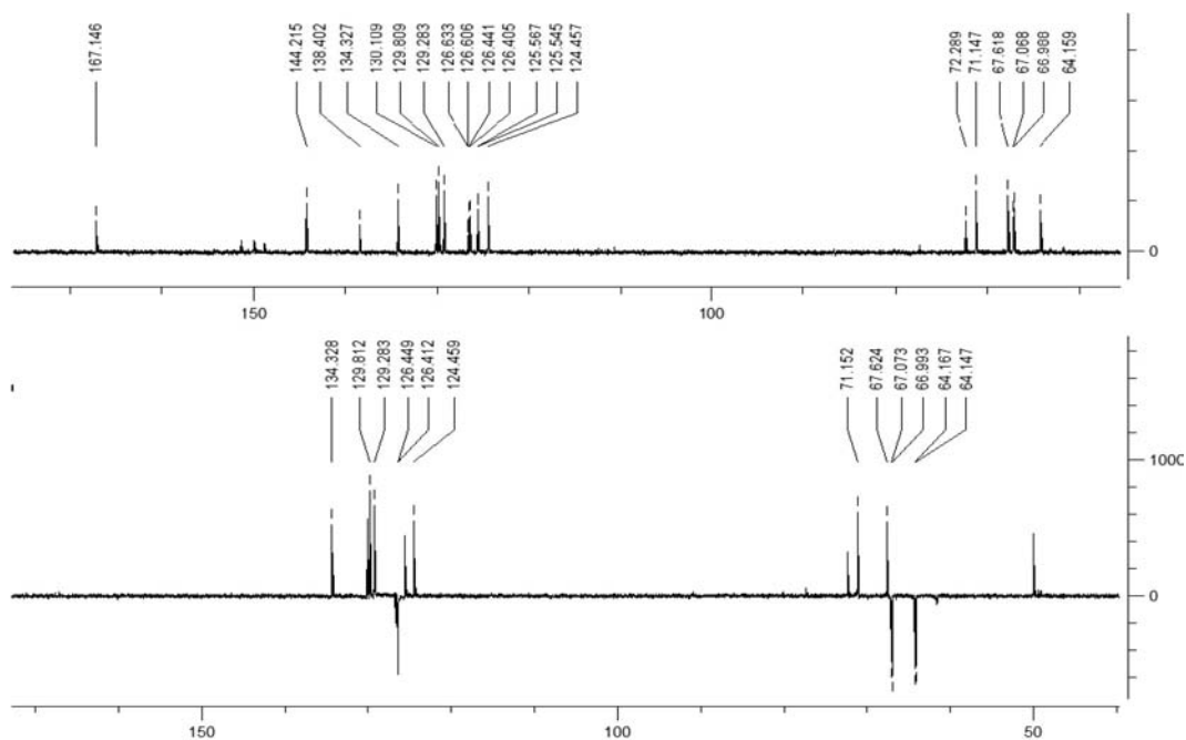
Figure S39. 13 C NMR spectrum of compound 8.
