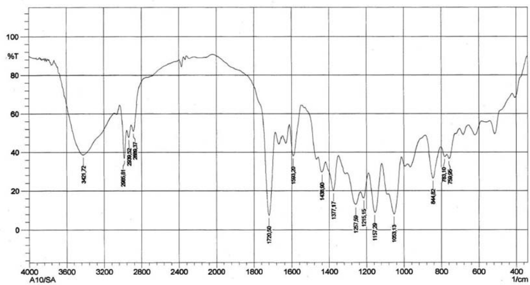
Figure S27. IR spectrum of compound 25.
