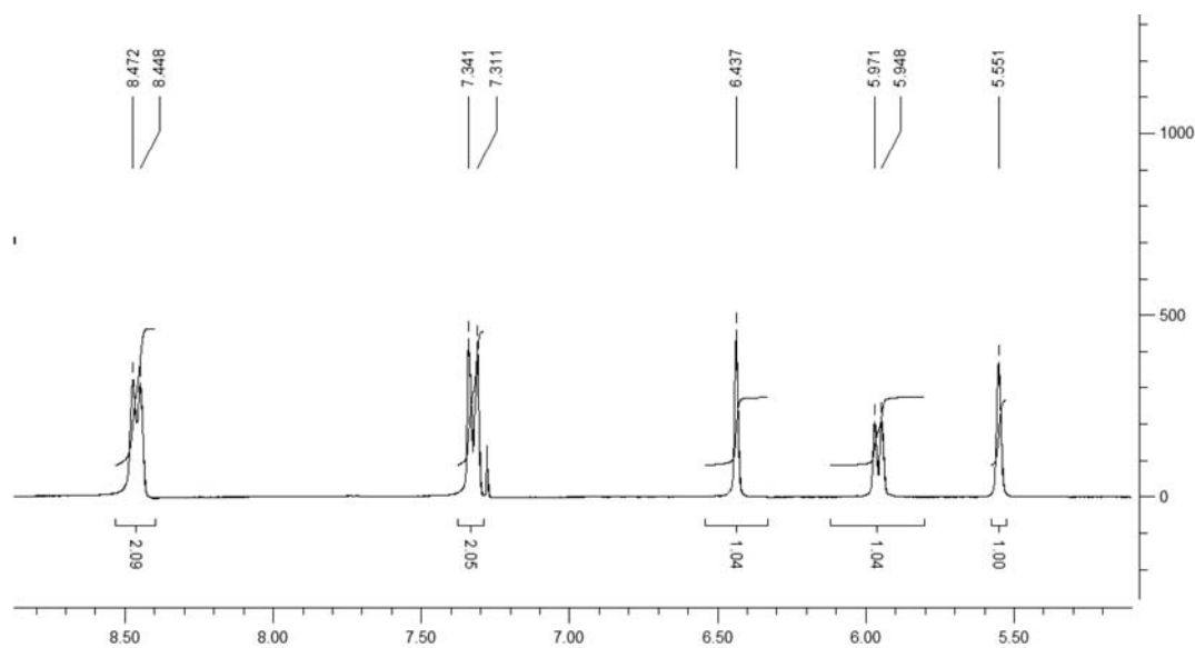
Figure S35. ^1H NMR spectrum of compound 27 .
