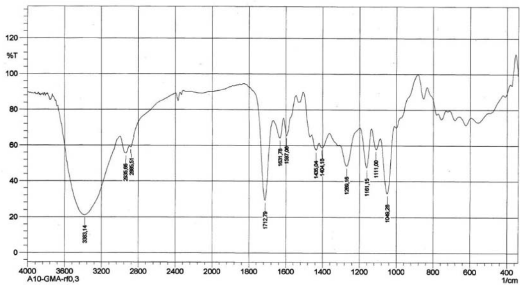
Figure S63. IR spectrum of compound 11.
