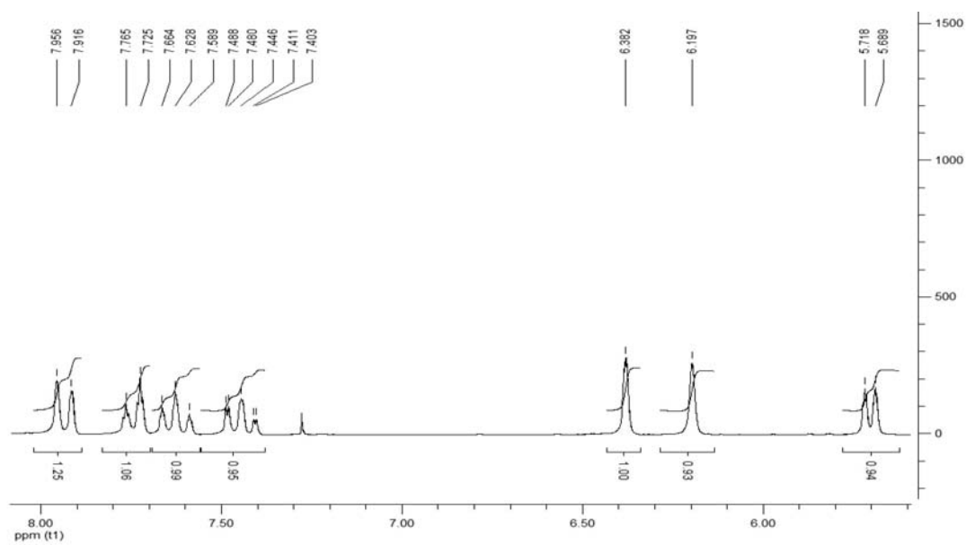
Figure S9. ^1\text{H} NMR spectrum of compound 22.
