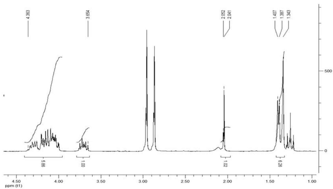
Figure S17. 1 H NMR spectrum of compound 23 .
