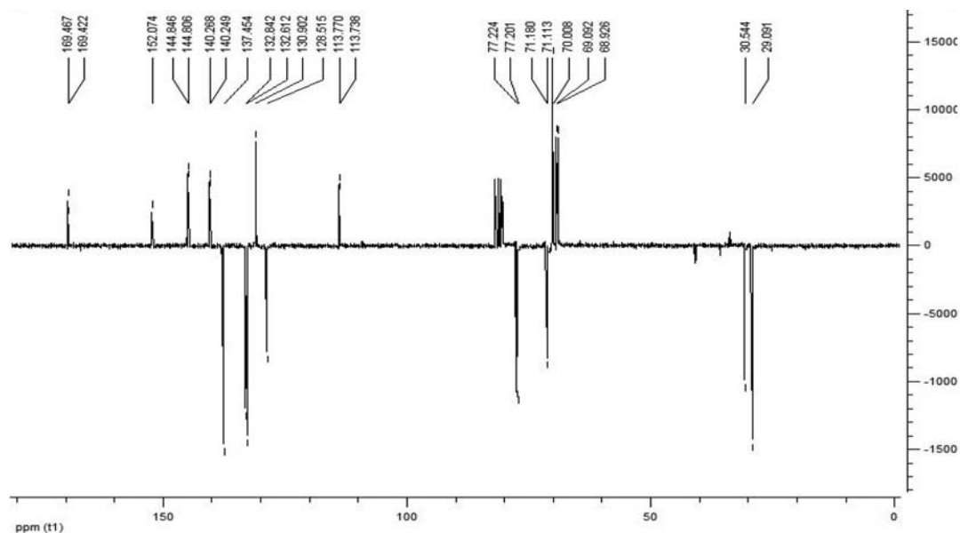
Figure S7. ^{13}\text{C} NMR spectrum of compound 22 .
