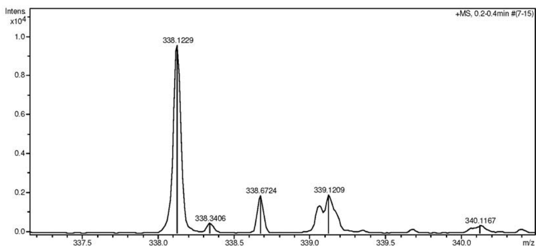
Figure S23. ESI-HRMS spectrum of compound 24 .
