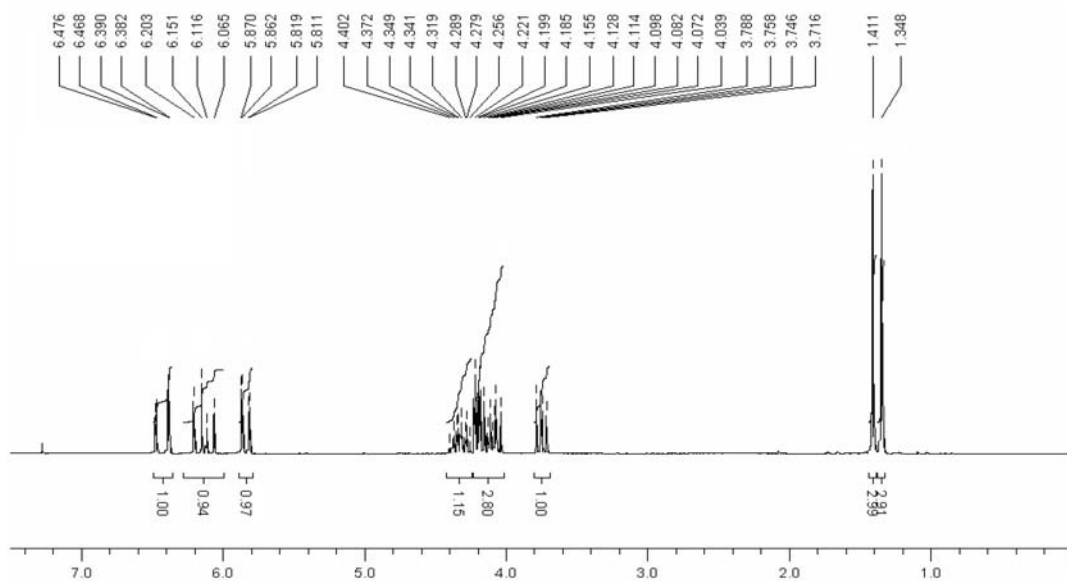
Figure S2. 1 H NMR spectrum of compound 20.
