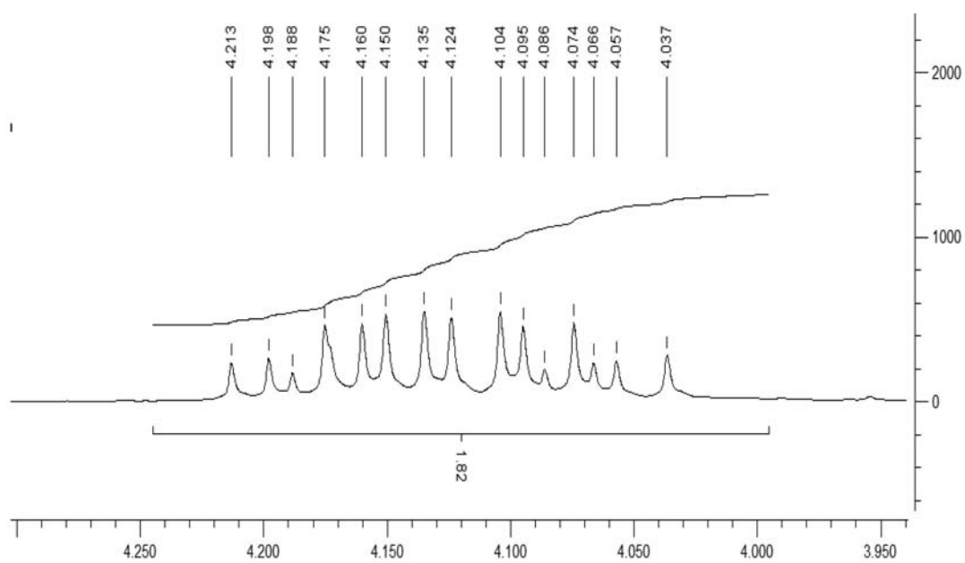
Figure S62. 1 H NMR spectrum of compound 11.
