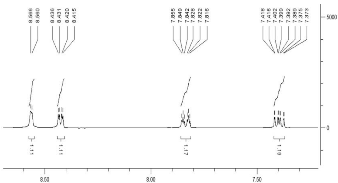
Figure S67. ^1\text{H} NMR spectrum of compound 12.
