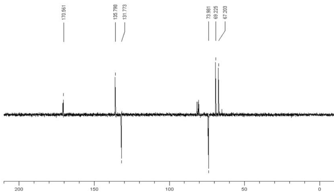
Figure S4. ^{13}\text{C} NMR spectrum of compound 21 .
