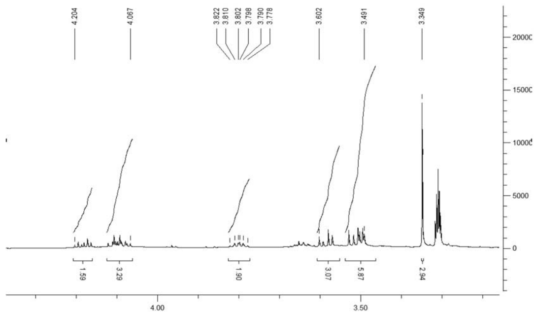
Figure S75. 1 H NMR spectrum of compound 13.
