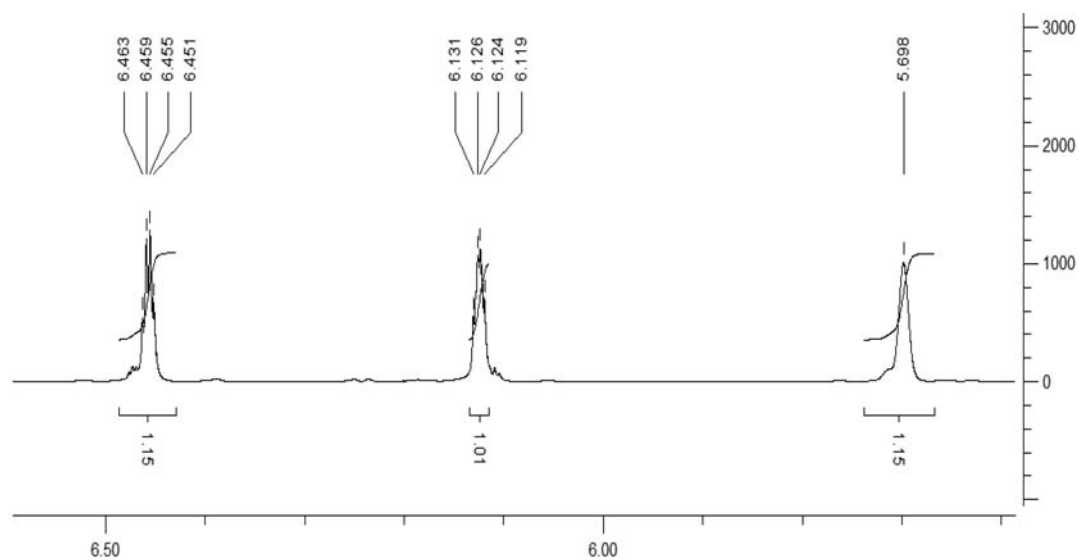
Figure S47. 1 H NMR spectrum of compound 9.
