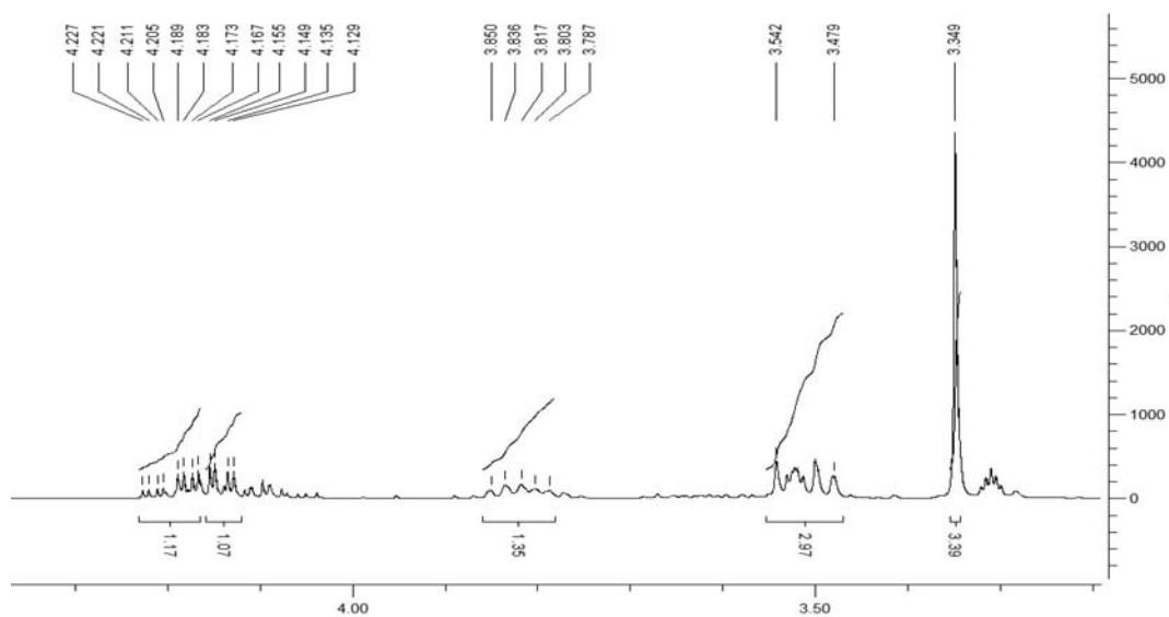
Figure S41. 1 H NMR spectrum of compound 8 .
