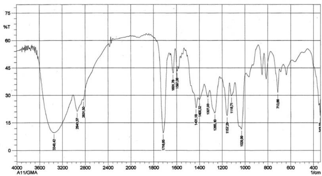
Figure S70. IR spectrum of compound 12.
