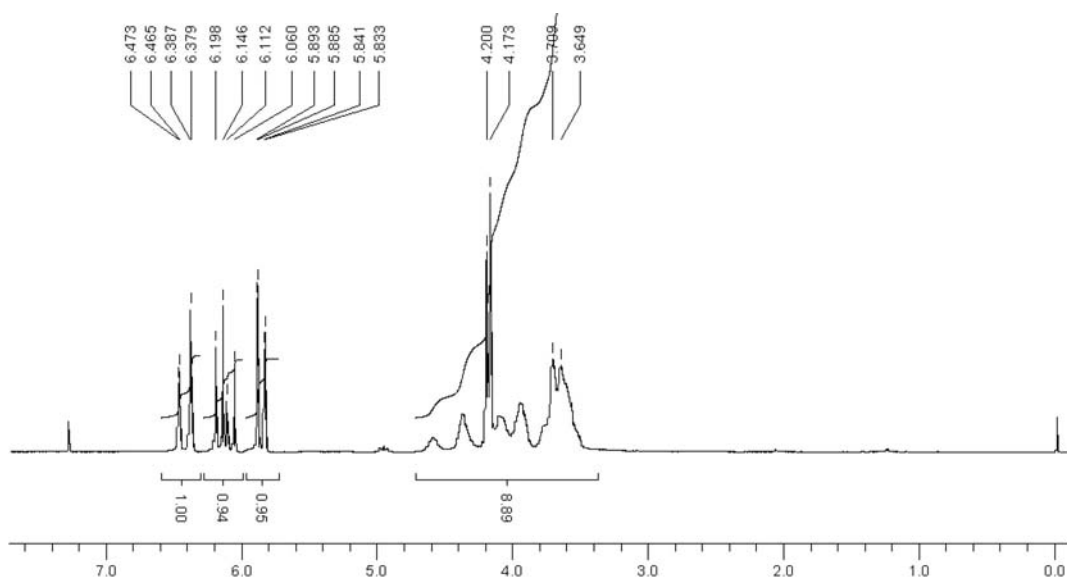
Figure S5. ^1\text{H} NMR spectrum of compound 21 .
