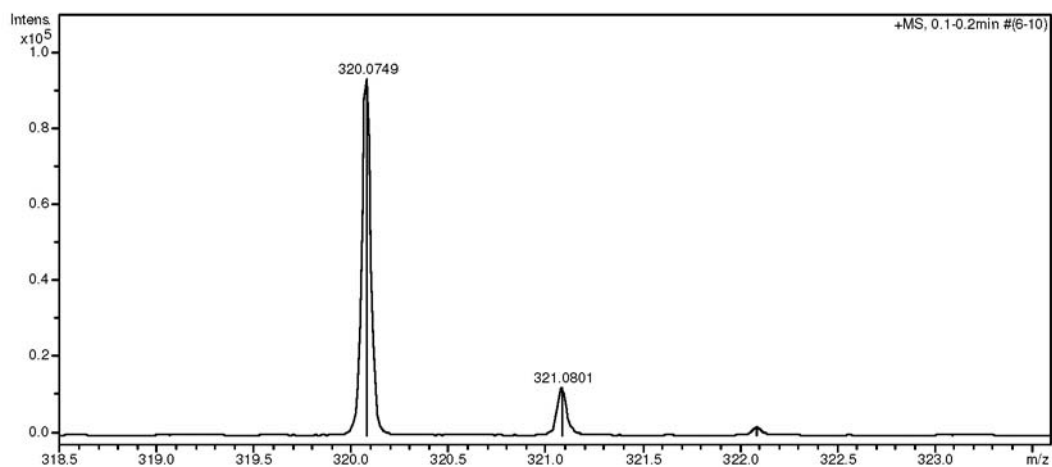
Figure S50. ESI-HRMS spectrum of compound 9 .
