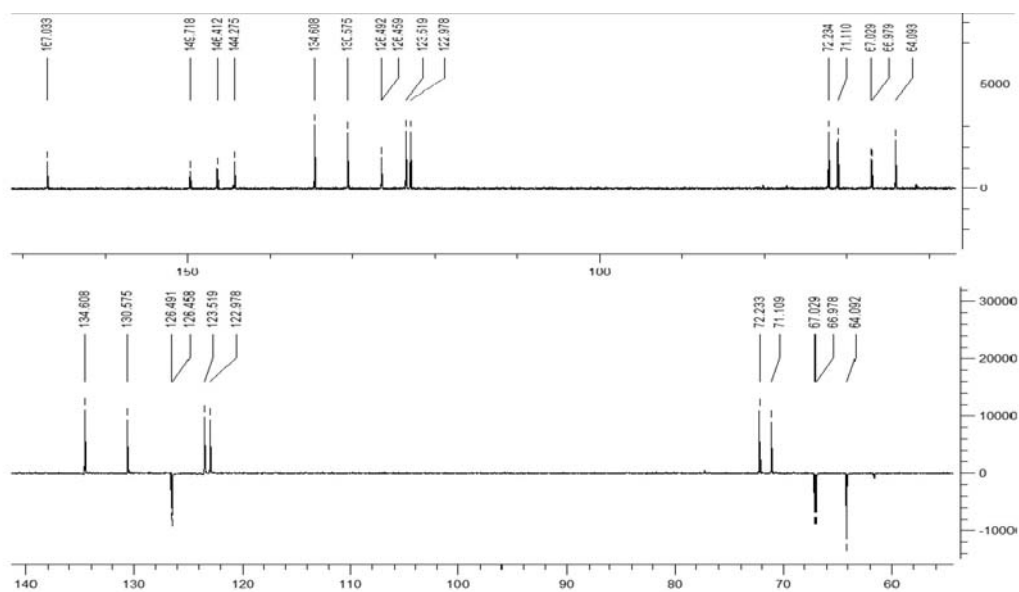
Figure S44. 13 C NMR spectrum of compound 9 .
