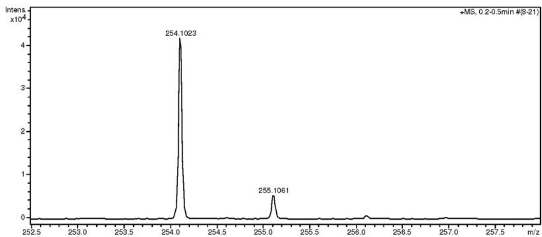
Figure S71. ESI-HRMS spectrum of compound 12.
