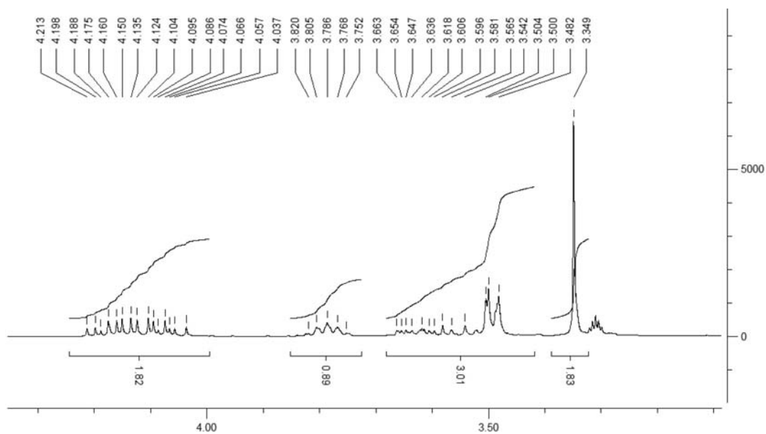
Figure S61. 1 H NMR spectrum of compound 11.
