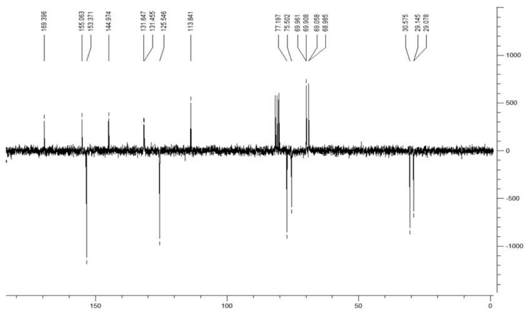
Figure S34. ^{13}C NMR spectrum of compound 27 .
