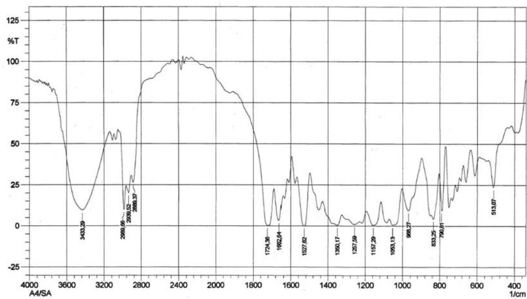
Figure S11. IR spectrum of compound 22.
