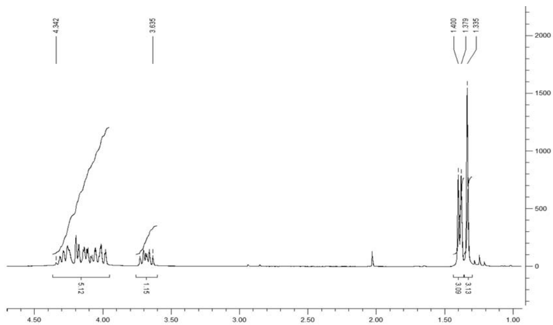
Figure S36. ^1\text{H} NMR spectrum of compound 27.
