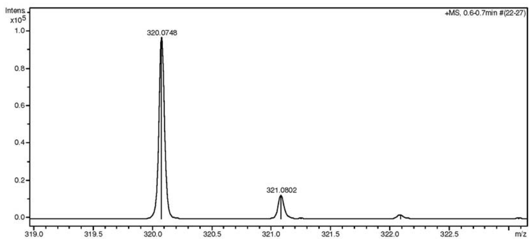
Figure S43. ESI-HRMS spectrum of compound 8 .
