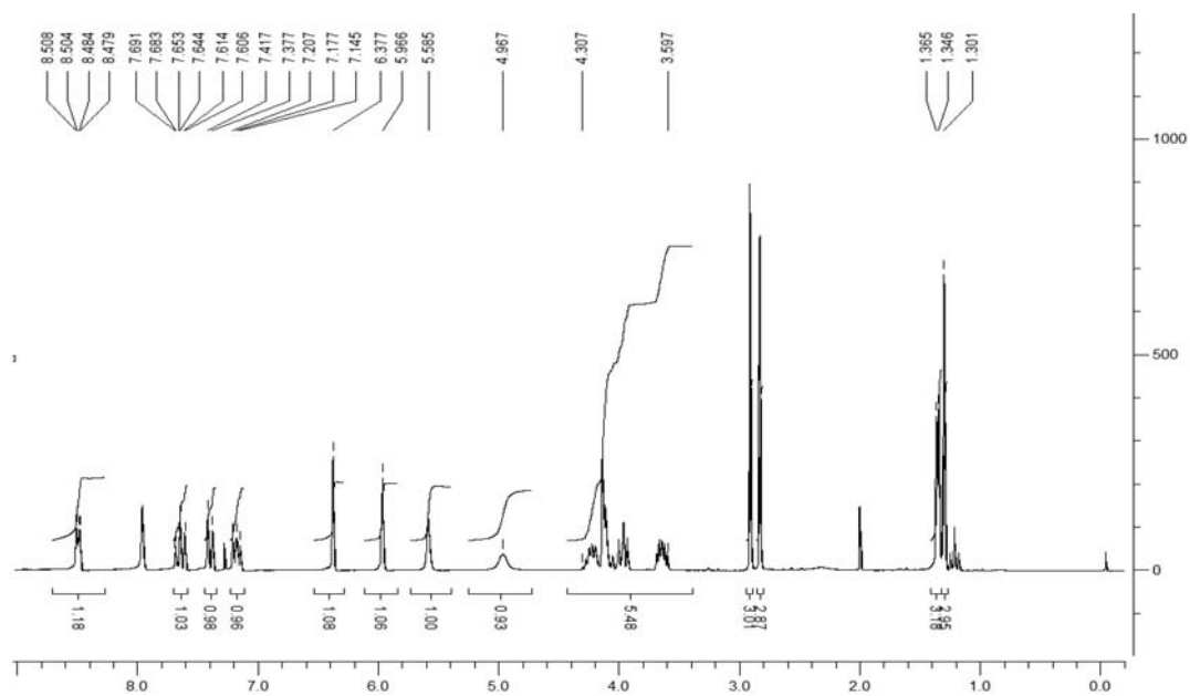
Figure S24. ^1\text{H} NMR spectrum of compound 25.
