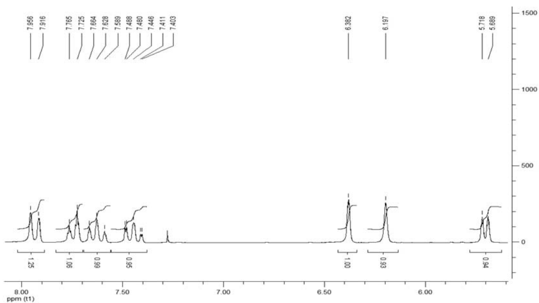
Figure S15. 1 H NMR spectrum of compound 23.
