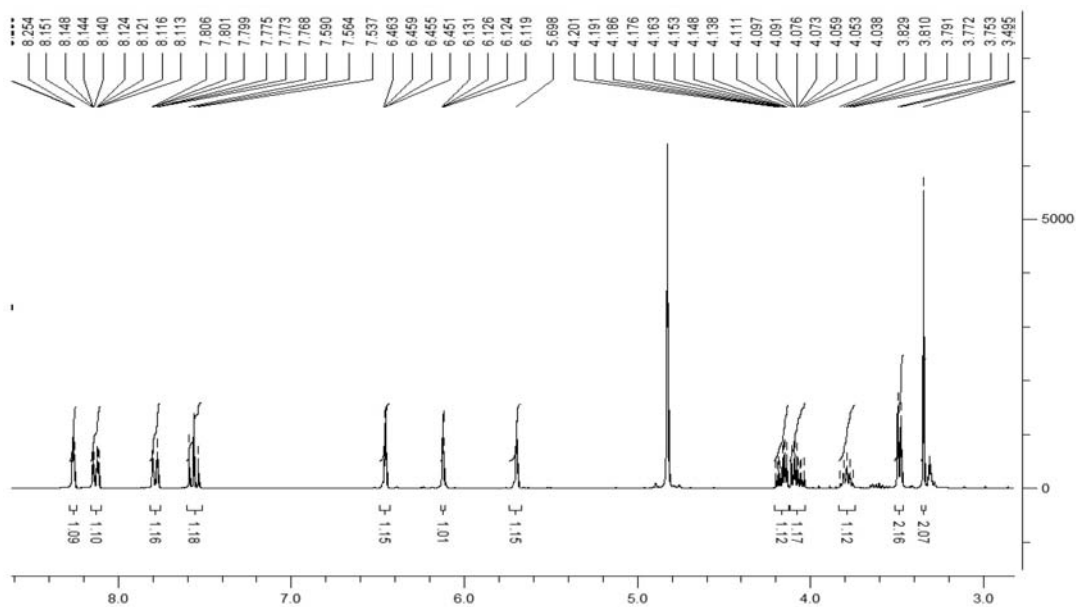
Figure S45. 1 H NMR spectrum of compound 9 .
