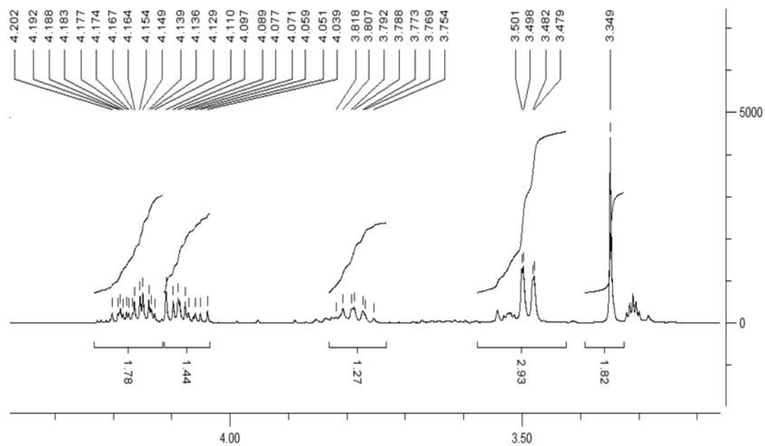
Figure S54. ^1\text{H} NMR spectrum of compound 10.
