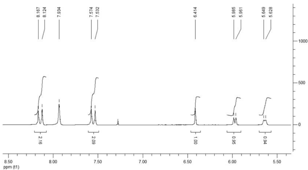
Figure S21. ^1\text{H} NMR spectrum of compound 24.
