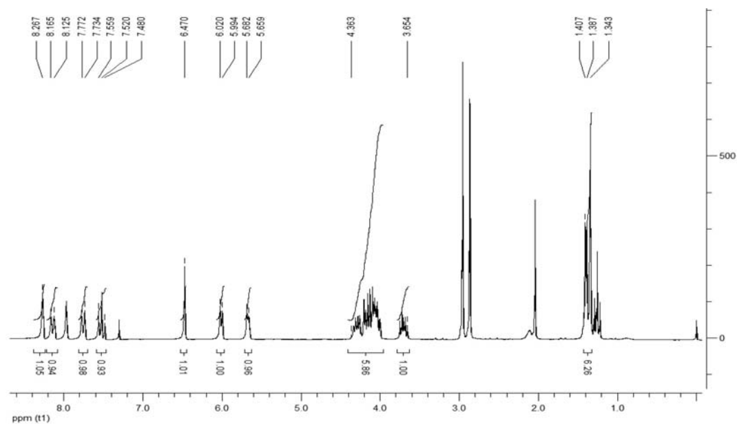
Figure S14. 1 H NMR spectrum of compound 23.
