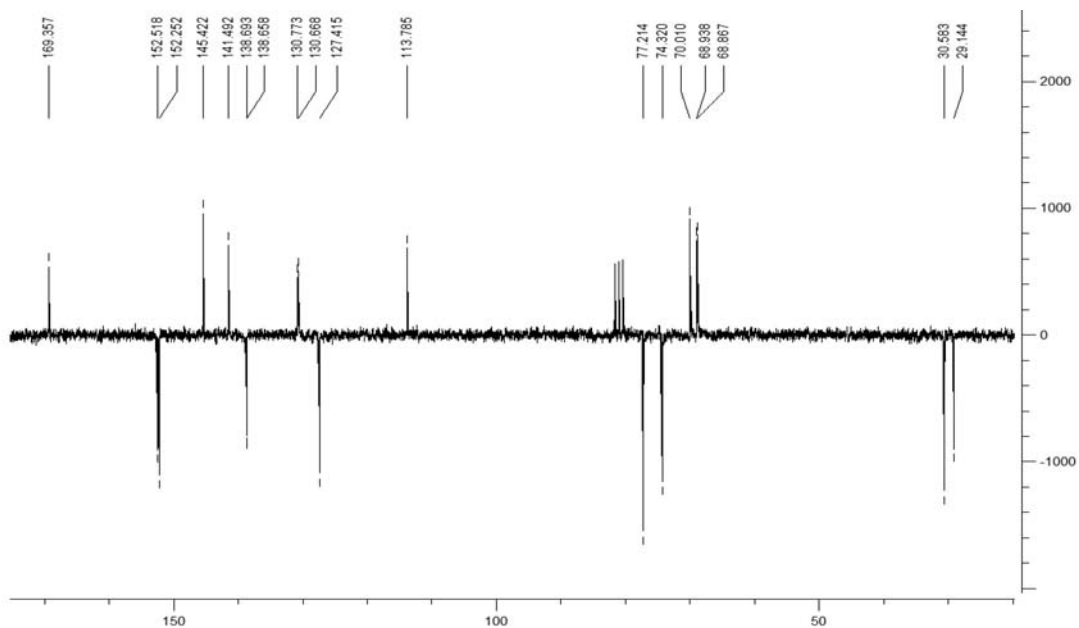
Figure S29. 13 C NMR spectrum of compound 26.
