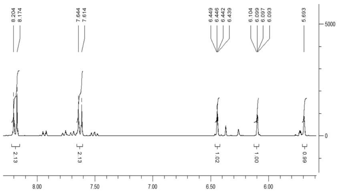
Figure S53. ^1\text{H} NMR spectrum of compound 10 .
