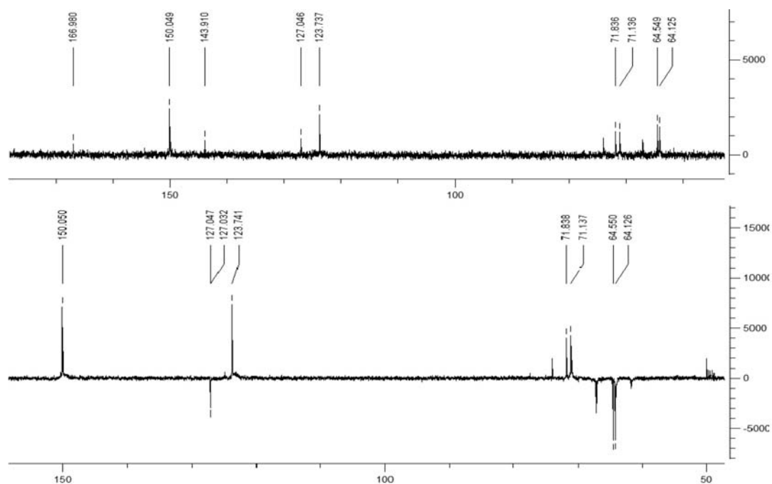
Figure S72. 13 C NMR spectrum of compound 13 .
