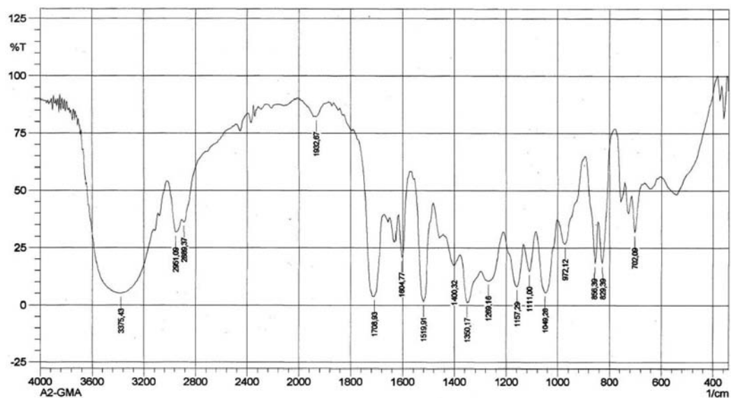
Figure S56. IR spectrum of compound 10.
