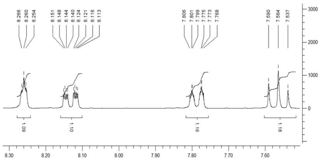
Figure S46. 1 H NMR spectrum of compound 9.
