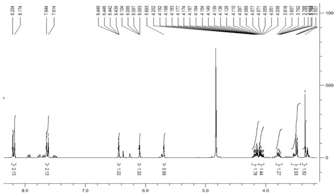
Figure S52. ^1\text{H} NMR spectrum of compound 10 .
