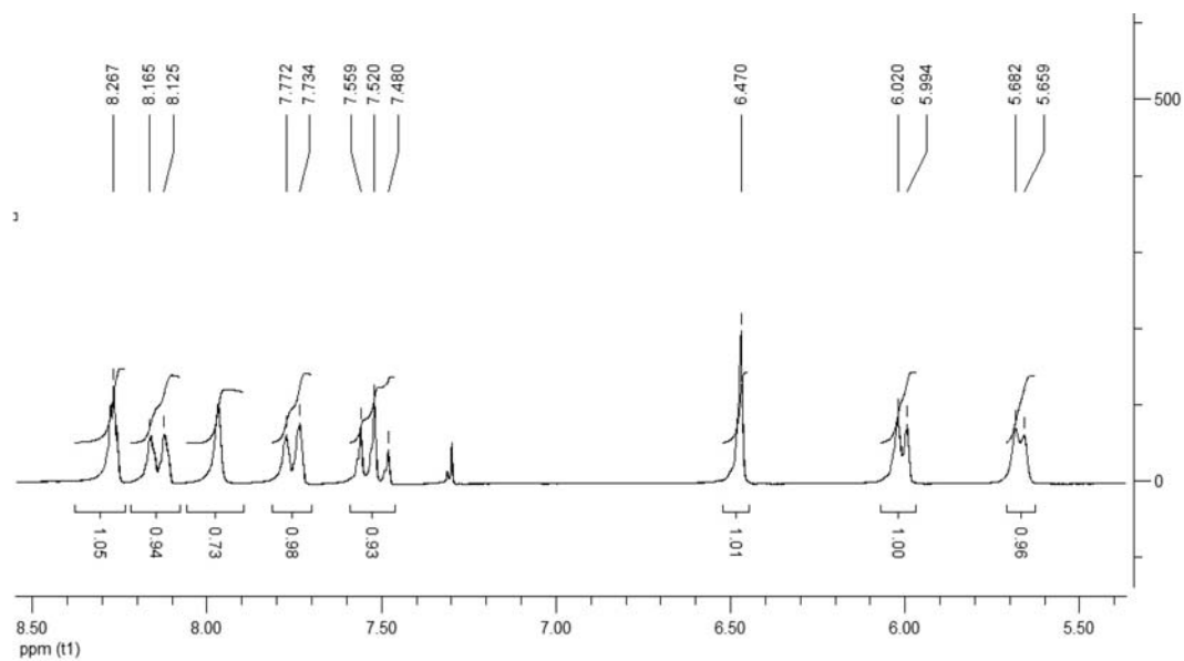
Figure S16. 1 H NMR spectrum of compound 23 .
