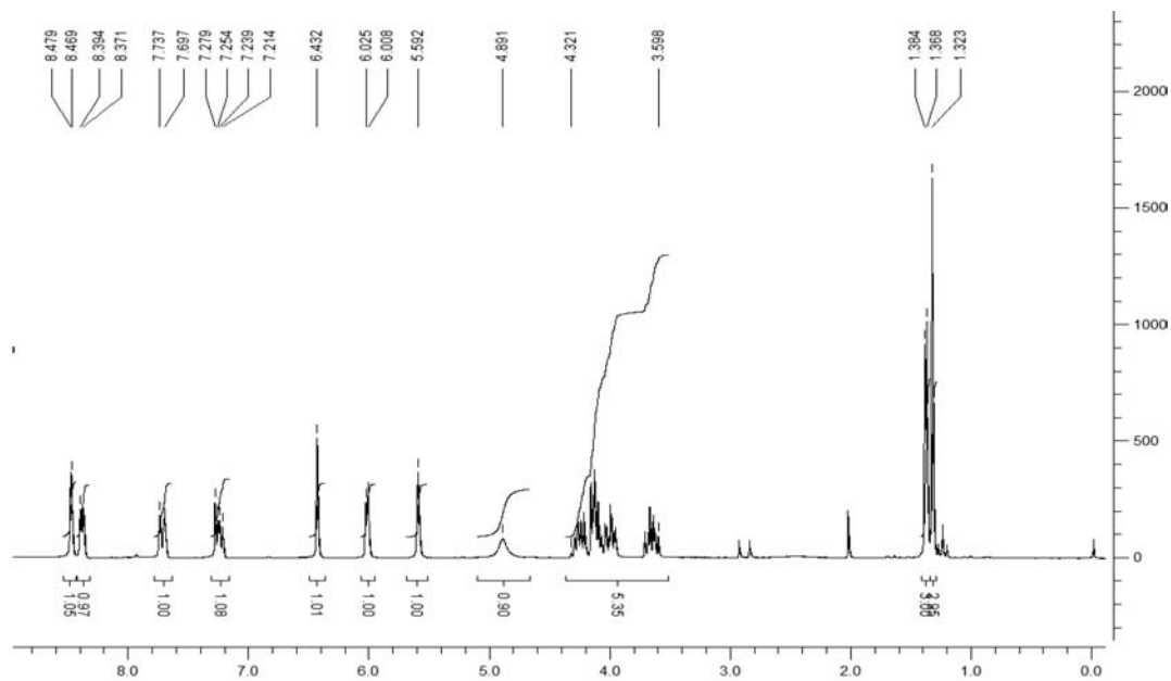
Figure S30. 1 H NMR spectrum of compound 26.
