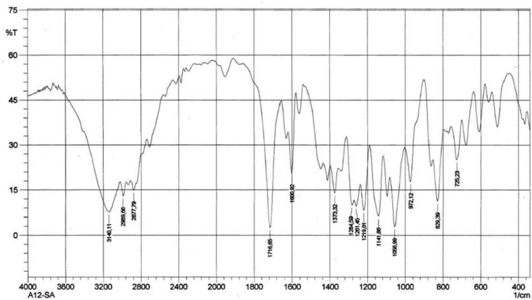
Figure S37. IR spectrum of compound 27.
