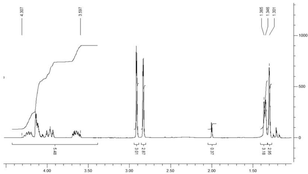
Figure S26. ^1\text{H} NMR spectrum of compound 25.
