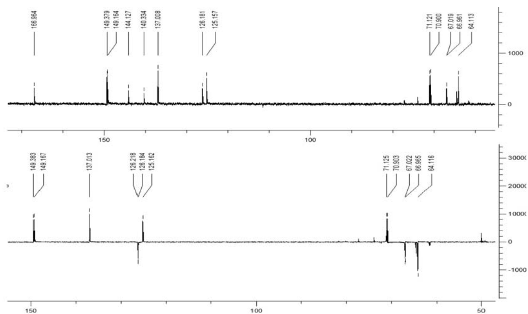
Figure S65. 13 C NMR spectrum of compound 12 .
