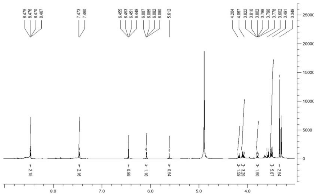
Figure S73. ^1\text{H} NMR spectrum of compound 13.
