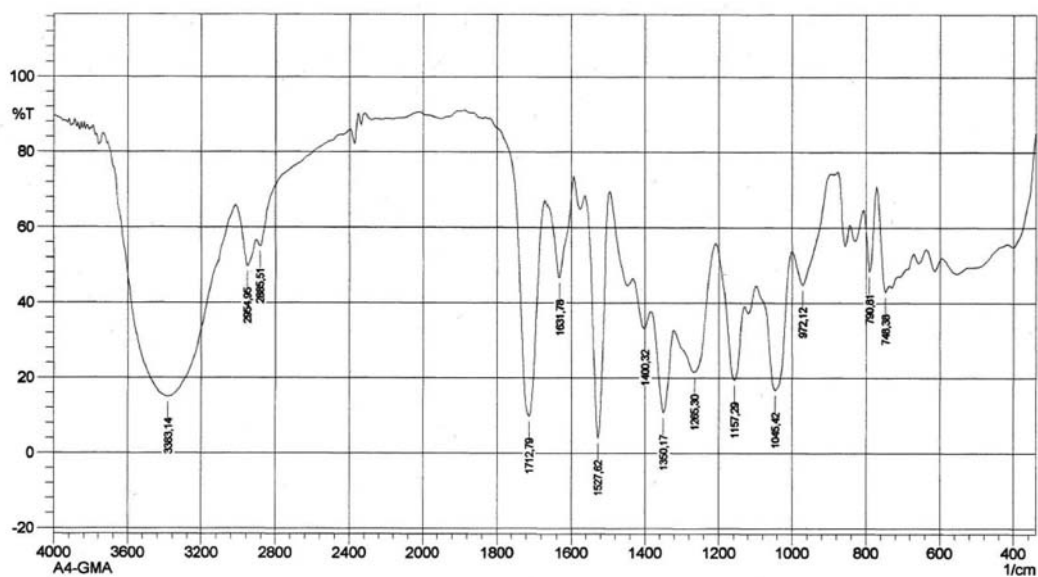
Figure S42. IR spectrum of compound 8 .
