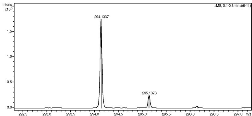
Figure S38. ESI-HRMS spectrum of compound 27.
