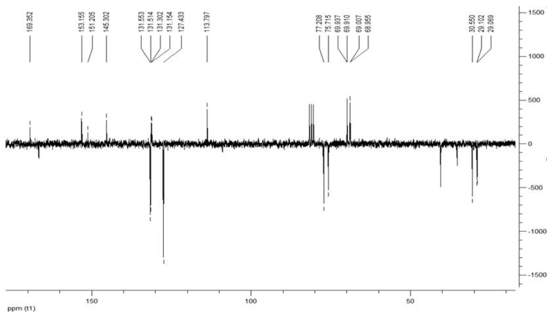
Figure S19. ^{13}C NMR spectrum of compound 24.
