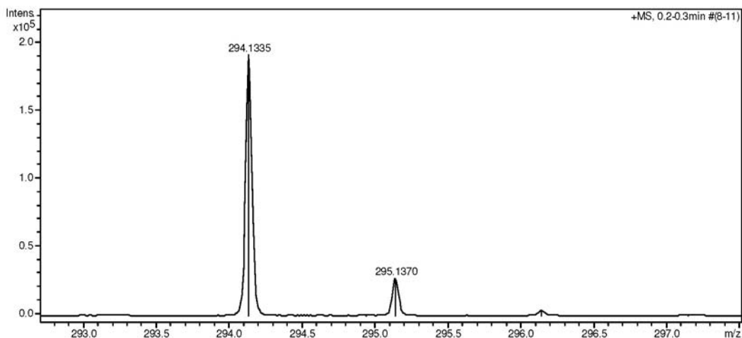
Figure S28. ESI-HRMS spectrum of compound 25.
