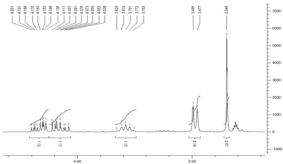
Figure S48. ^1\text{H} NMR spectrum of compound 9 .
