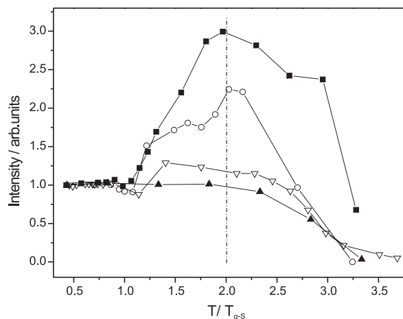
Figure 7. Temperature dependence of the intensity of the layer reflexions in P_{11M} (■), P_{11Cl} (○), P_{410} (▽) and P_{48} (▲).
