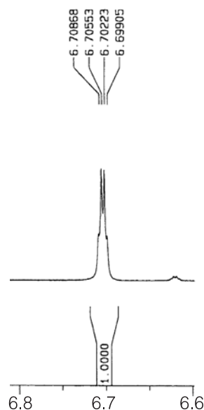
Figure 6. Expansion of the vinylic resonance ( \delta 6.70 and 6.61) for natural 1a/1b .
