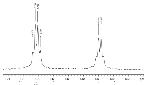
Figure 3. Expansion of the vinylic resonances ( \delta 6.70 and 6.61) for synthetic 1a/1b .
