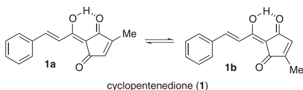
Figure 1. Enol forms of cyclopentenodione derivative ( 1 ).
