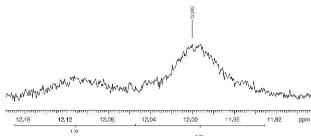
Figure 9. Expansion of the OH resonance ( \delta 12.1 and 12.0) for synthetic 1a/1b after \text{SiO}_2 column chromatography.
