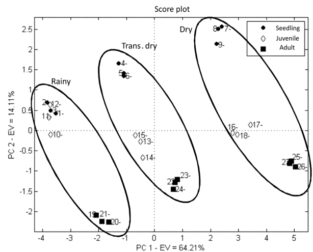
Figure 2. Score plot for principal component analysis.
