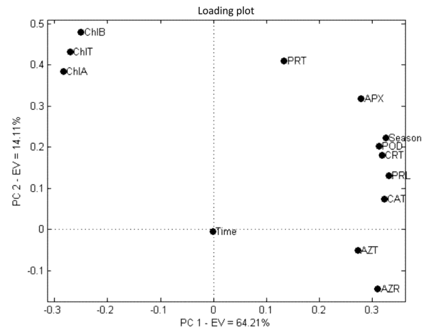
Figure 1. Loading plot for principal component analysis.
