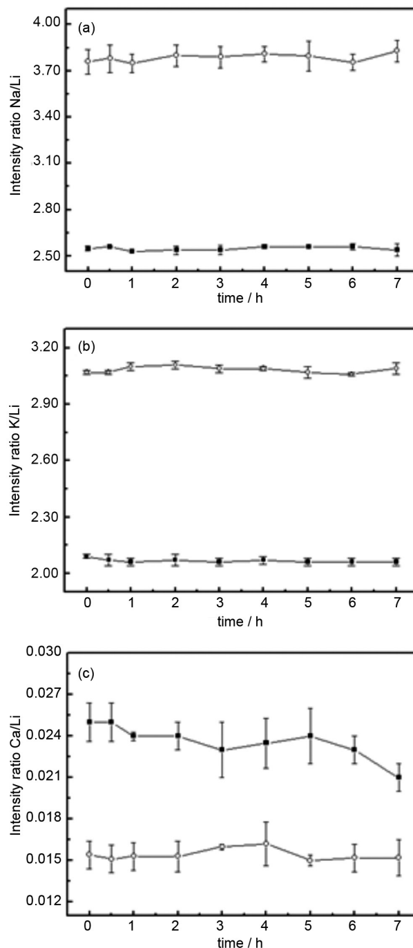
Figure 3. Variation in the intensity ratio for Na, K and Ca for biodiesel emulsions (O) and standard solutions (■): (a) sunflower biodiesel emulsion and 1.0 mg kg -1 of Na; (b) cotton biodiesel emulsion and 1.0 mg kg -1 of K; (c) sunflower biodiesel emulsion and 2.5 mg kg -1 of Ca.
