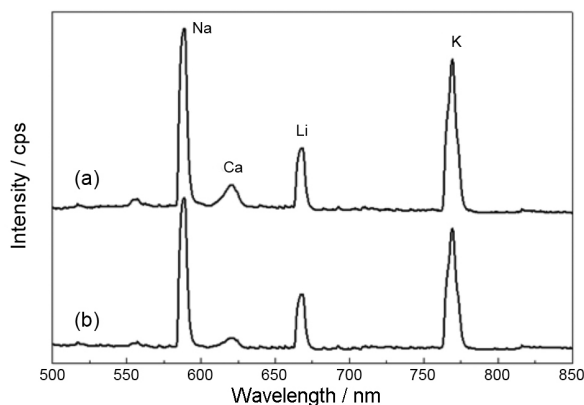
Figure 1. Line emission spectra for Na ( 1 \text{ mg kg}^{-1} ), Ca ( 5 \text{ mg kg}^{-1} ), Li ( 1 \text{ mg kg}^{-1} ) and K ( 1 \text{ mg kg}^{-1} ) in organometallic standard solution diluted in (a) kerosene and in (b) aqueous standard solution.
