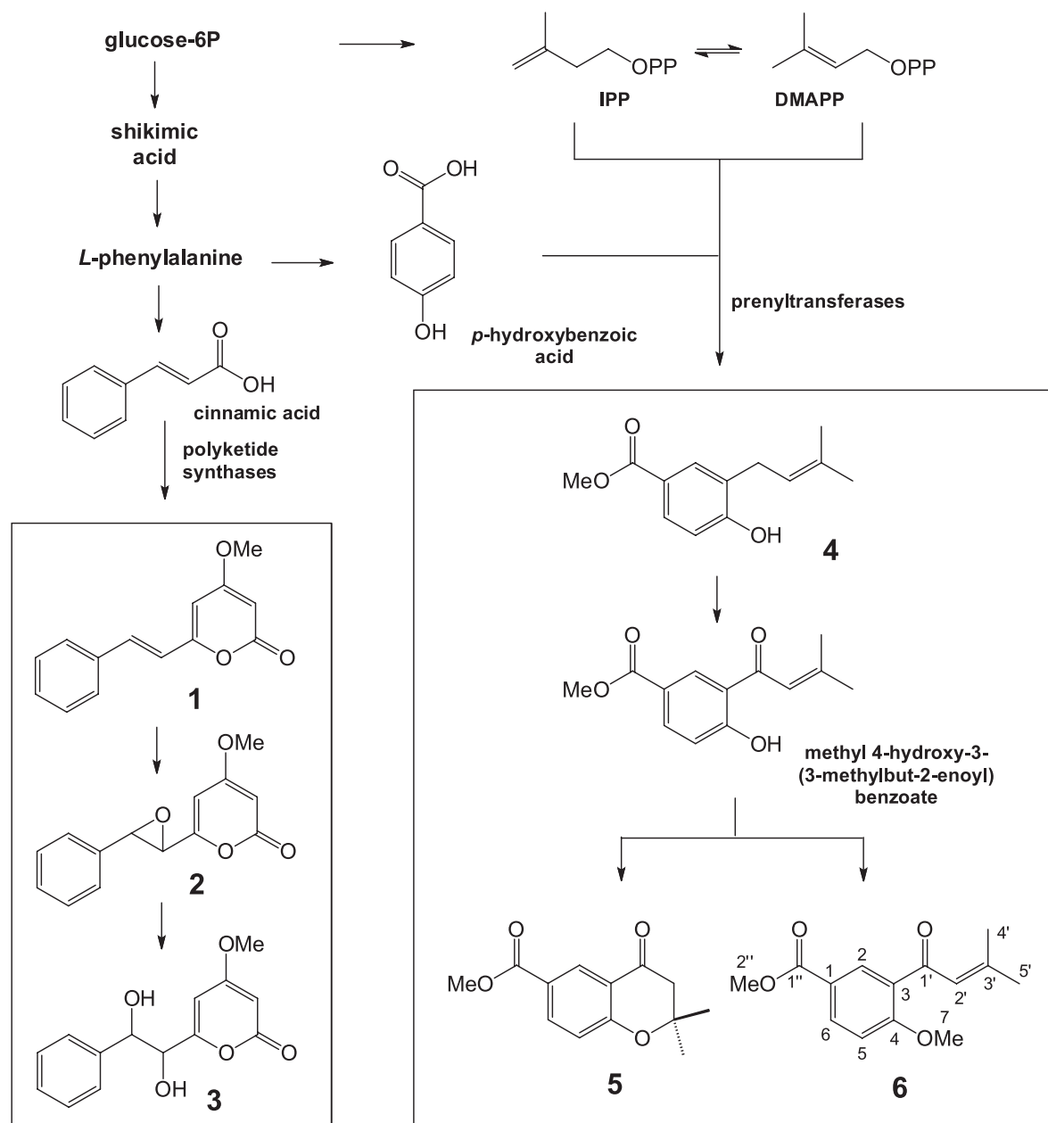
Figure 1. Compounds isolated from P. fuliginum (1-6) and their biosynthetic relationships. IPP: isopentenyl diphosphate; DMAPP: 3,3-dimethylallyl diphosphate.
