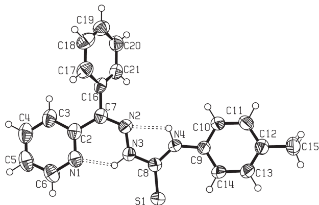
Figure 2. Molecular plot of HL3 showing the labeling scheme of the non-H atoms and their displacement ellipsoids at the 50% probability level.
