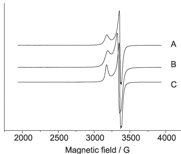
Figure 3. X-band EPR spectra of (A) [Cu(HL1)Cl 2 ] (1); (B) [Cu(HL2)Cl 2 ] (2); (C) [Cu(HL3)Cl 2 ] (3) at room temperature (~300 K).
