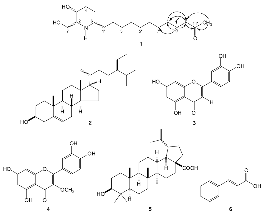
Figure 1. Compounds isolated from flowers and unripe fruits of S. spectabilis and correlations ^1\text{H} \rightarrow ^{13}\text{C} observed in the HMBC contour map of 1 .
