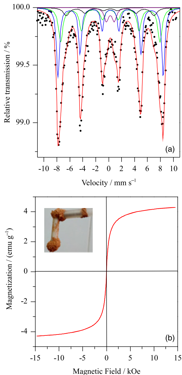
Figure 8. (a) 150 K Mössbauer spectra; (b) M-H curve of MCat after the 4 th cycle of reuse.
