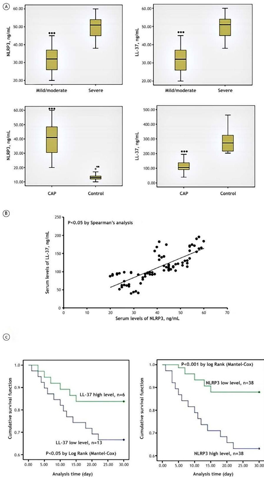
Figure 1. (A) Serum NLRP3 and LL-37 levels in patients with CAP (n=76) and healthy controls (n=50) and levels in patients with mild/moderate (n=41) or severe (n=35) CAP patients determined by ELISA. *p<0.05 vs. control group; (B) Correlation analysis between NLRP3 and LL-37 in CAP patients using Spearman's correlation analysis; (C) Kaplan-Meier survival curve of CAP patients with low or high serum NLRP3 or LL-37 levels.
