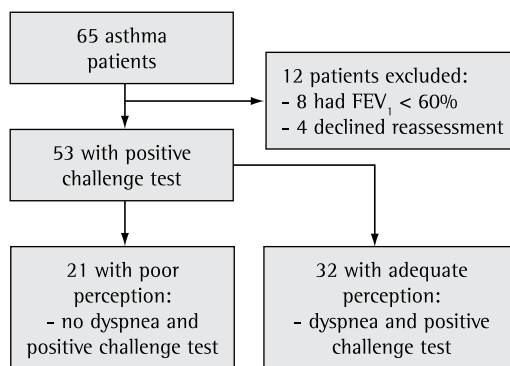
Figure 1 - Study algorithm.
